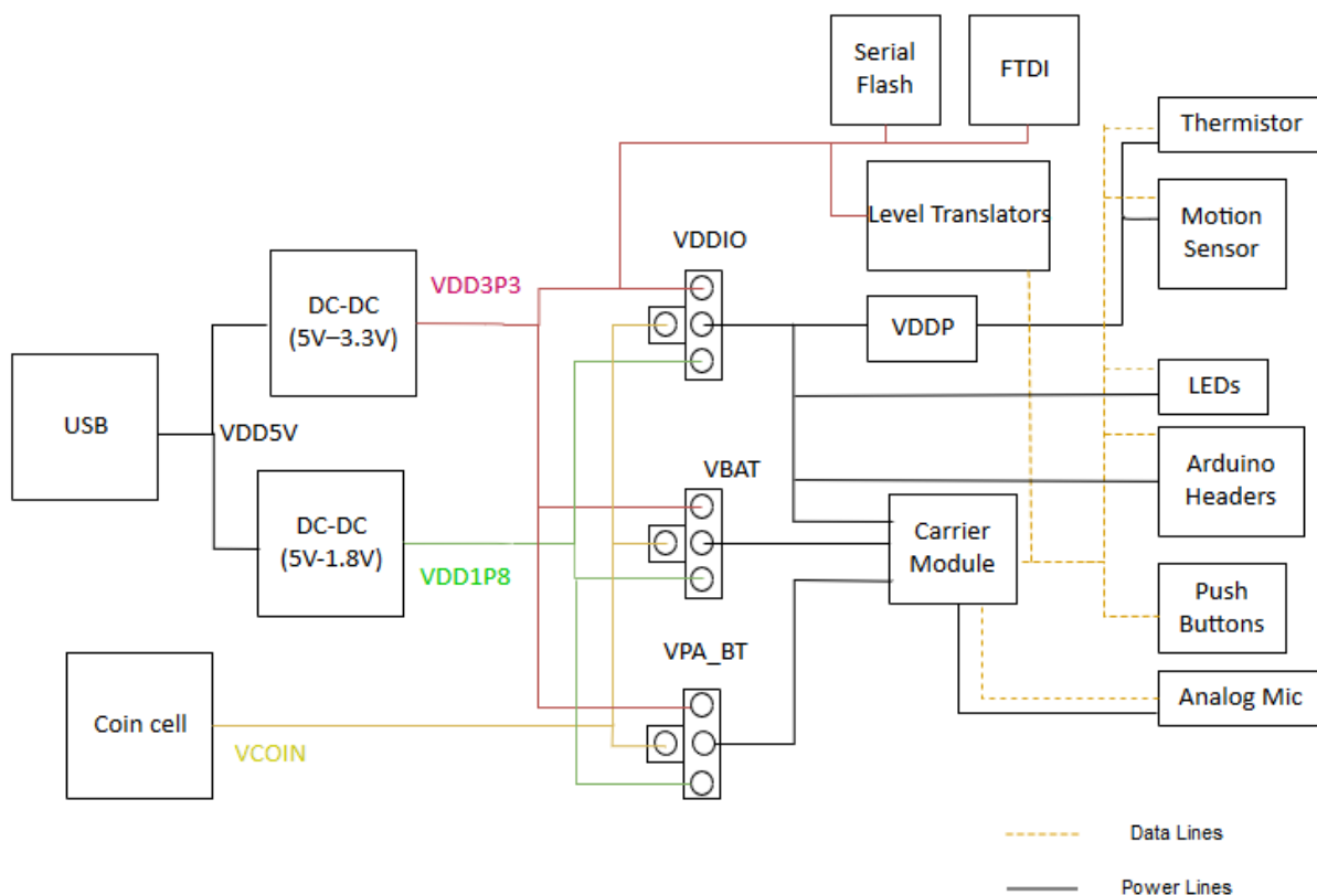
Figure 3-2. Power Architecture
