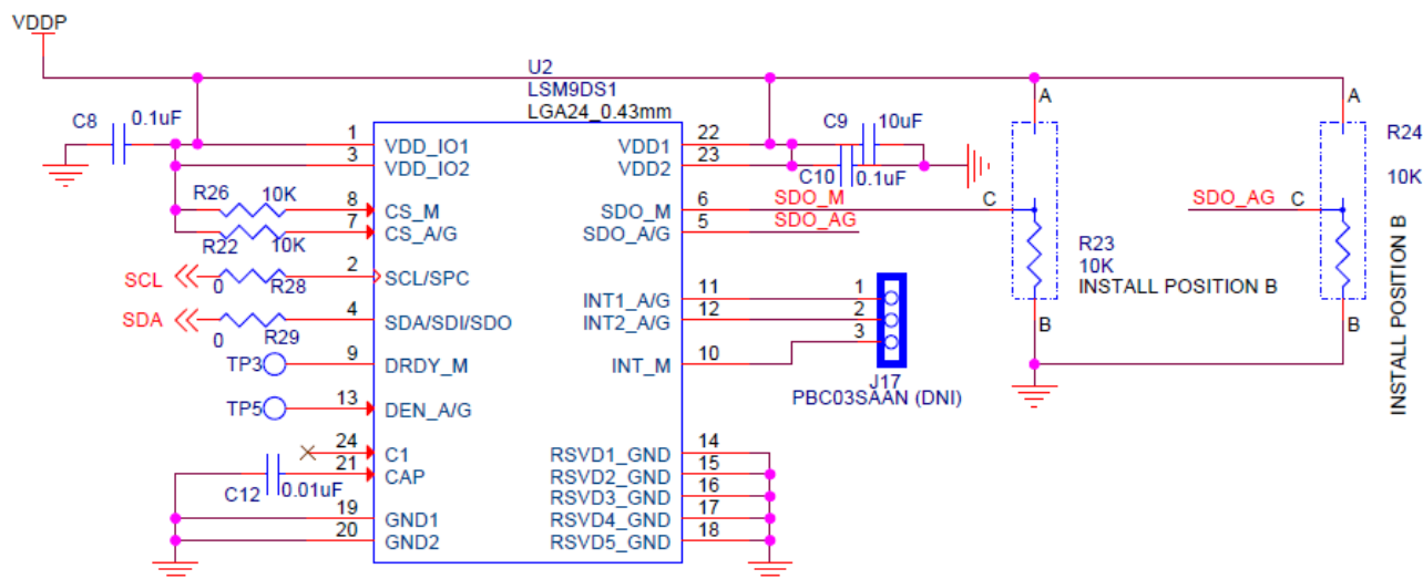
Figure 3-13. Motion Sensor Circuit
