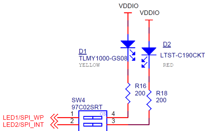
Figure 3-14. LED Circuit
