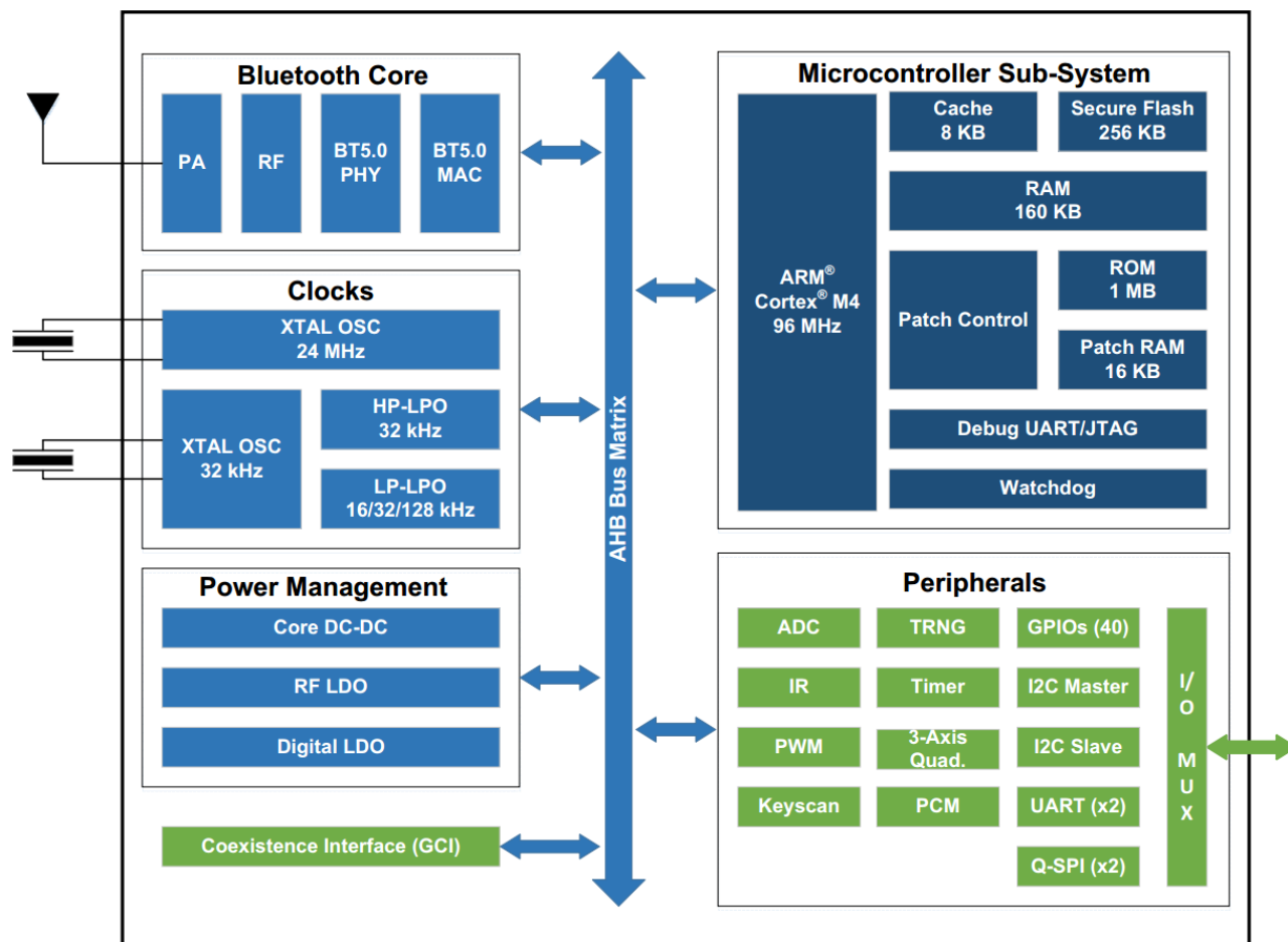
Figure 2-1. Block Diagram of CYW20819-A1
