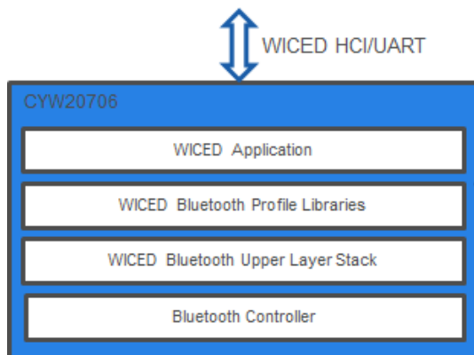
Figure 1-1. CYW20706 WICED Architecture
