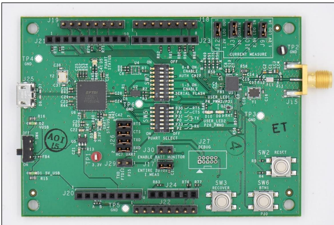
Figure 3-1. CYW920706WCDEVAL Evaluation Board
