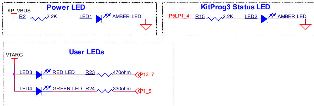
Figure 5-9. Schematics of LEDs
