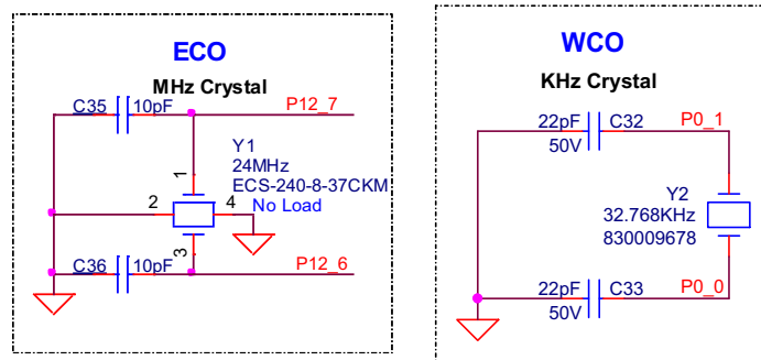
Figure 5-12. Schematics of Crystal Oscillator
