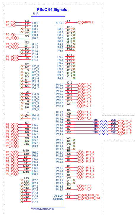
Figure 5-1. Schematics of PSoC 64 Signals
