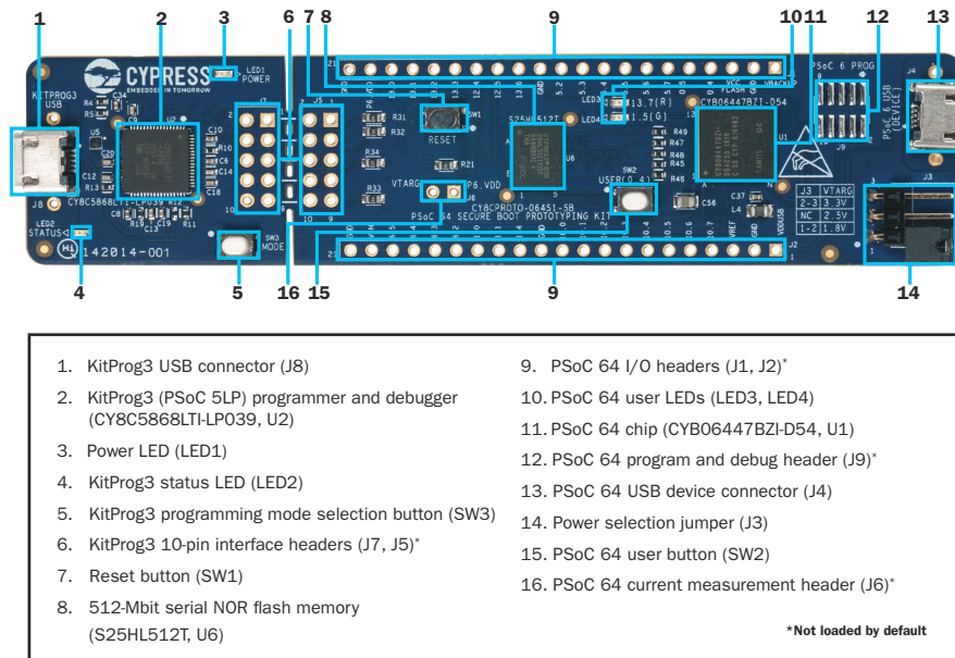
Figure 3-3. PSoC 64 “Secure Boot” Prototyping Board - Top View
