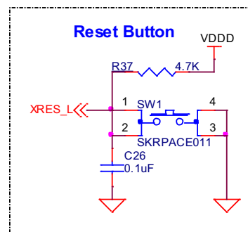
Figure 5-11. Reset Button
