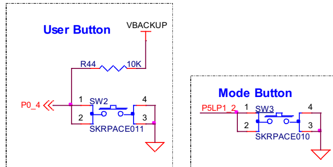
Figure 5-10. Schematics of Push Buttons
