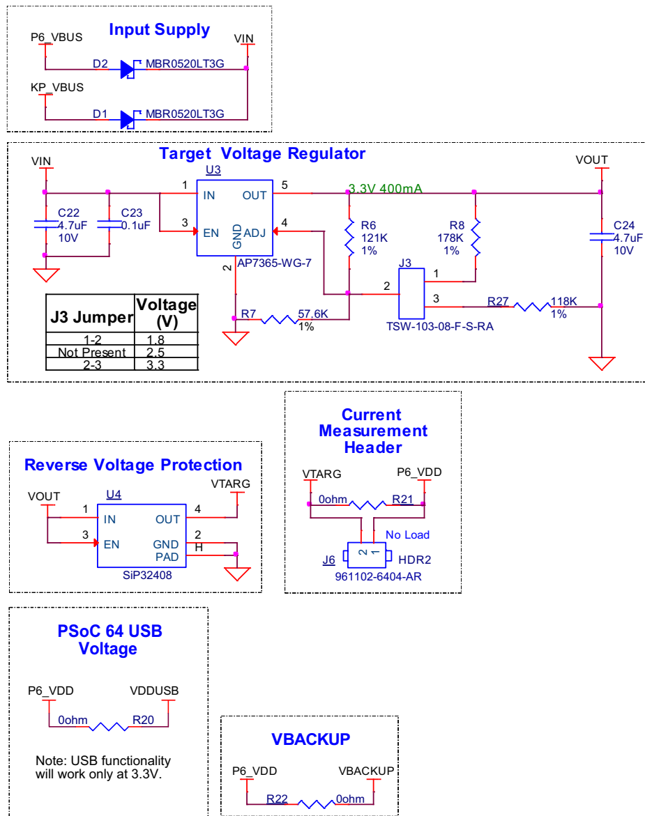
Figure 5-4. Schematics of Power Supply System
