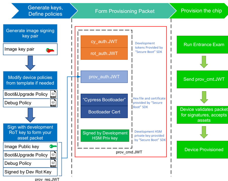
Figure 4-1. Provisioning Flow
