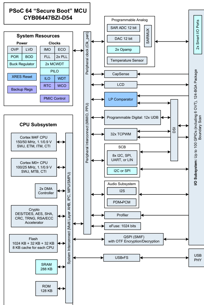
Figure 3-1. PSoC 64 Block Diagram
