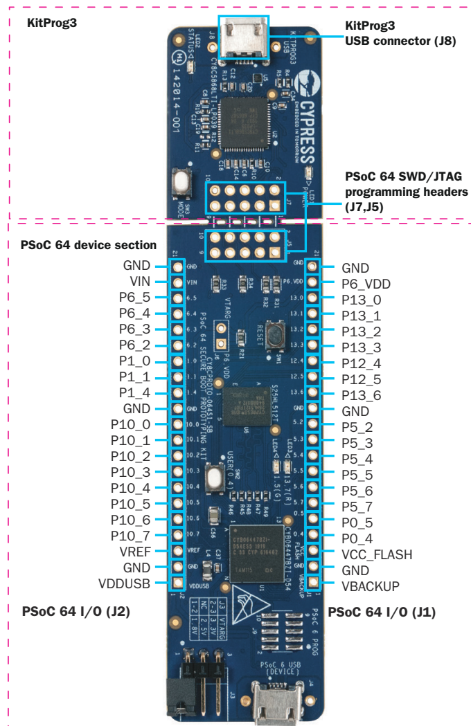
Figure 5-6. J1 and J2 Headers
