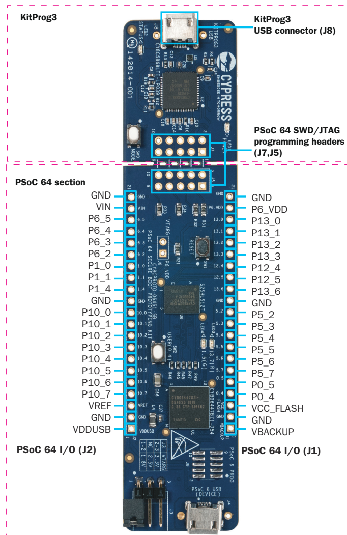
Figure 1-1. Prototyping Board Pinout
