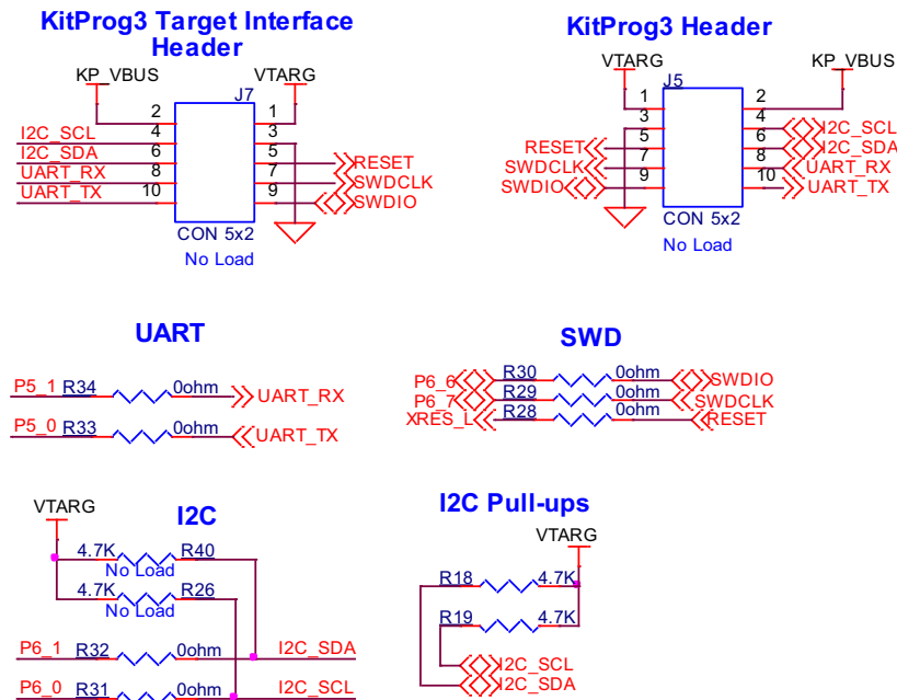
Figure 5-3. Schematics of Programming and Serial Interface Connections
