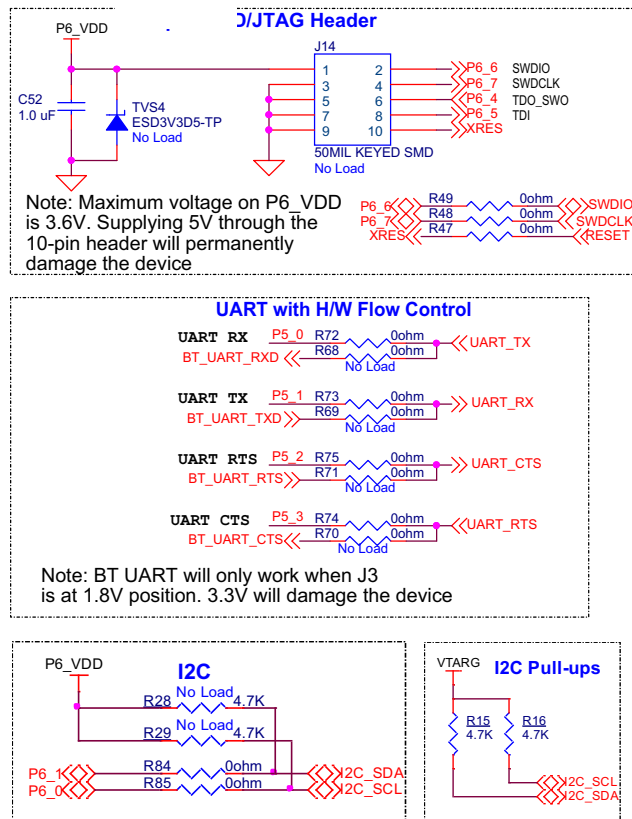
Figure A-3. Schematics of Programming and Serial Interface Connections
