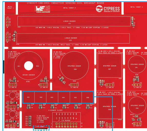
CY8CKIT-148-COIL Inductive Sensing Coil Breakout Board
