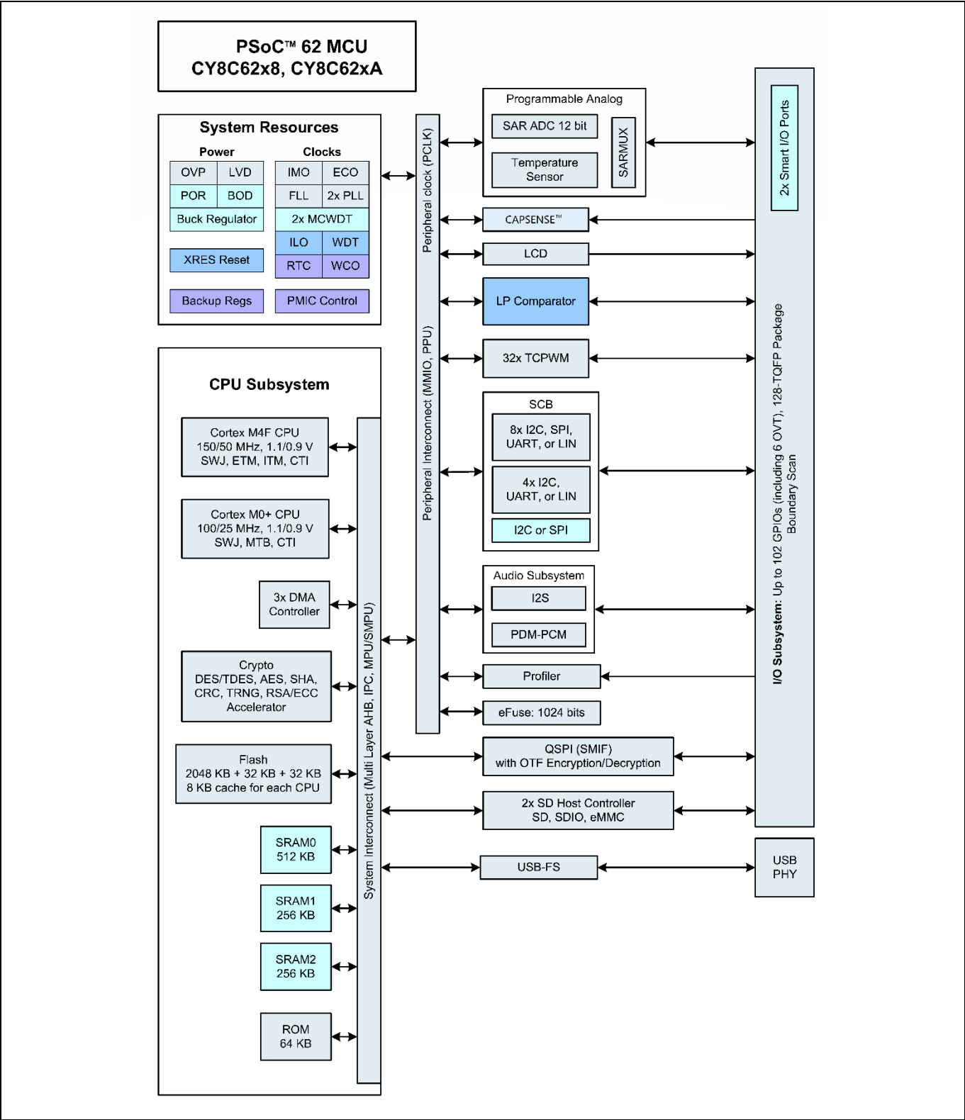
Figure 5 PSoC™ 62 MCU block diagram
