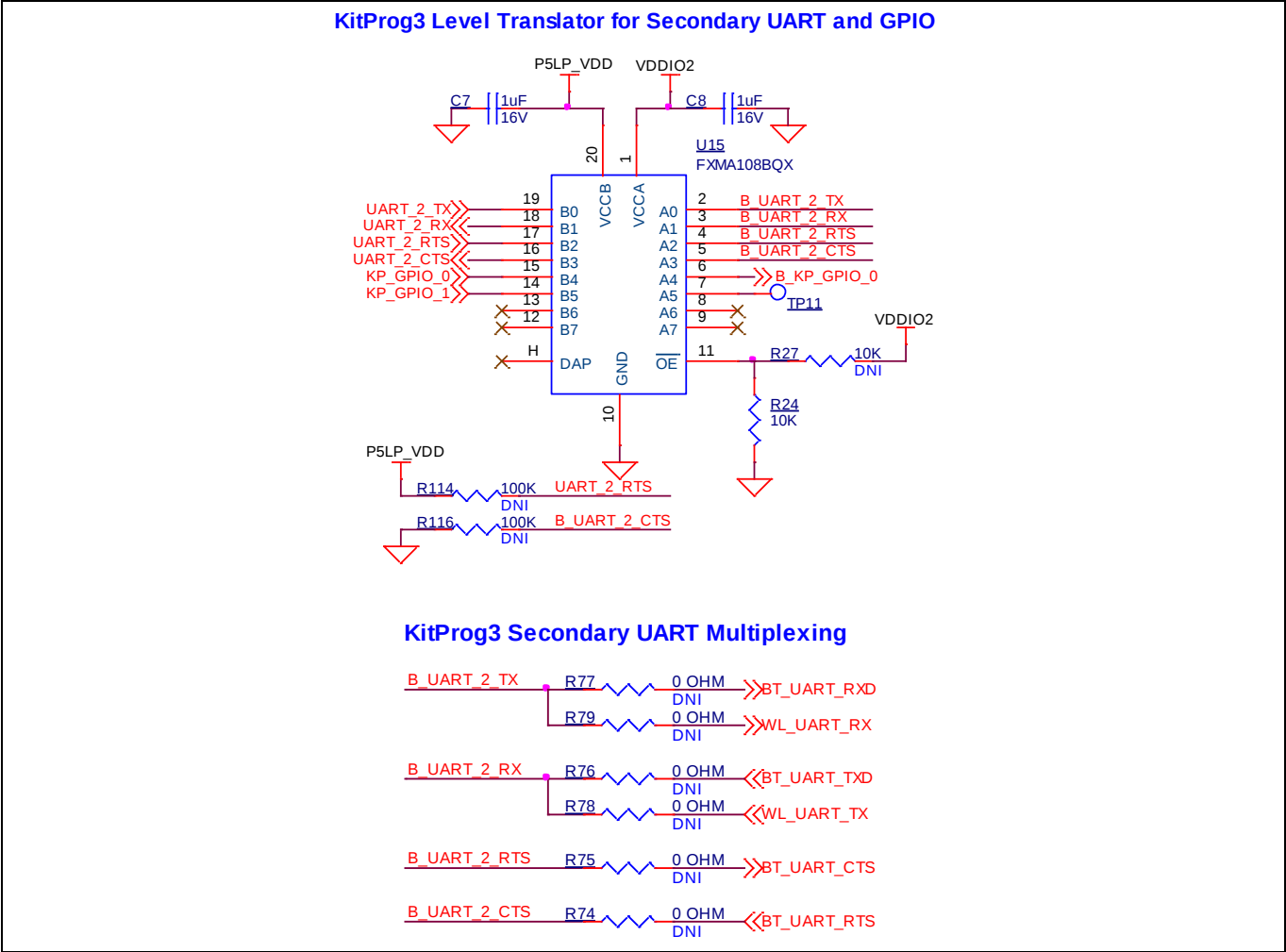
Figure 23 Serial interconnection between PSoC™ 5LP and M.2 interface
