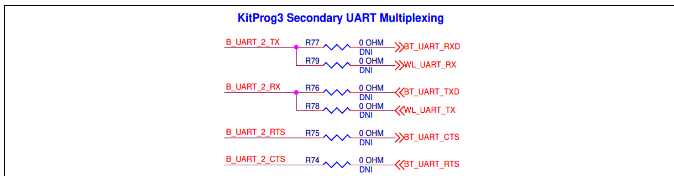
Figure 47 Secondary UART interface between PSoC™ 5LP and M.2 module
