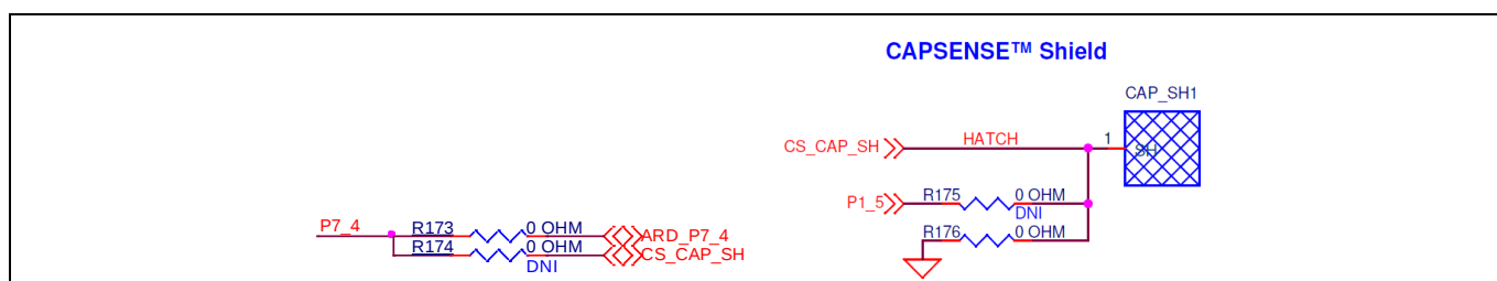
Figure 41 CAPSENSE™ shield
