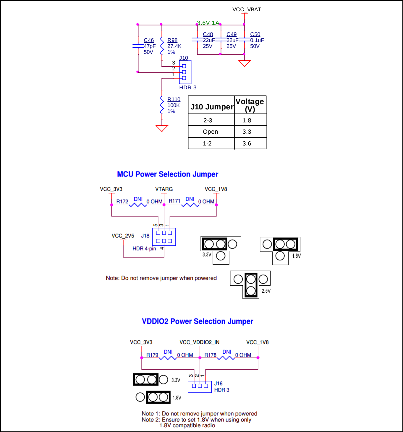
Figure 26 Voltage selection
