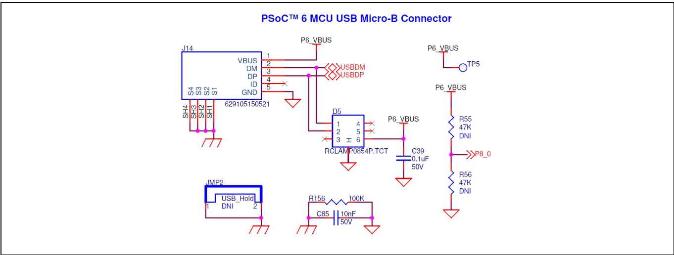
Figure 39 PSoC™ 6 MCU USB Micro-B connector
