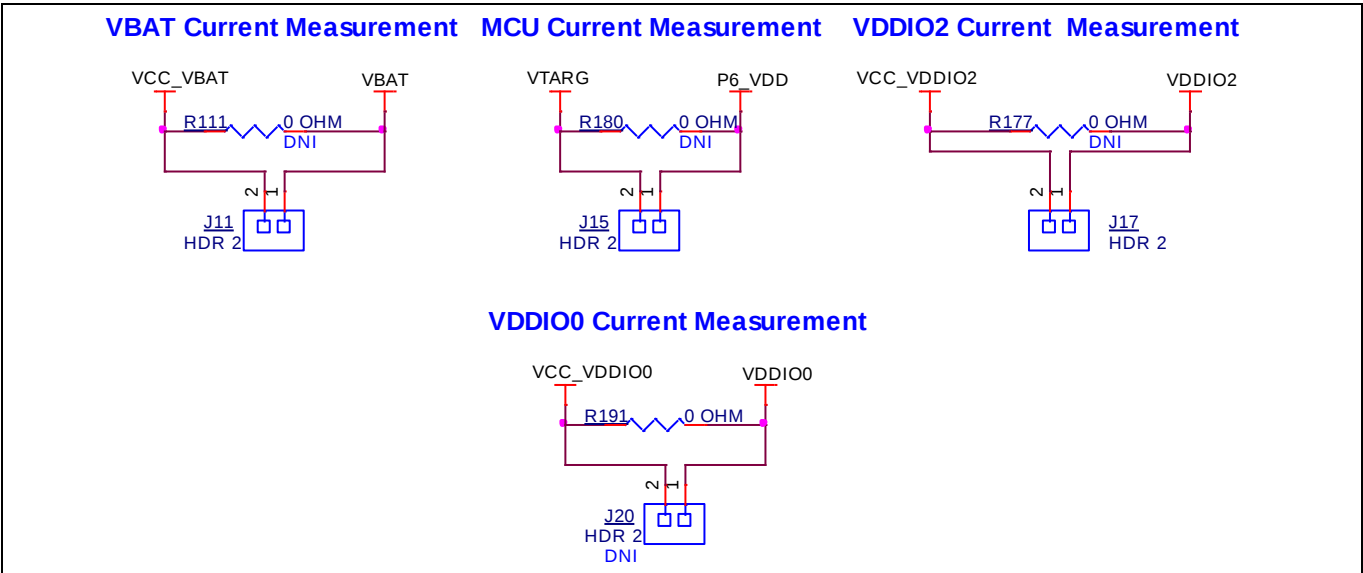
Figure 28 Current measurement headers
