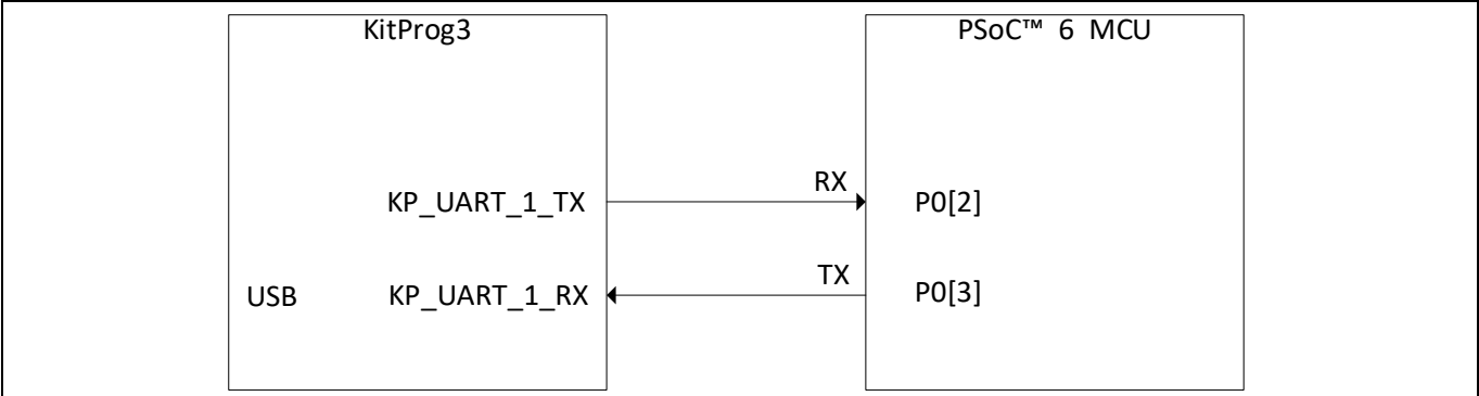
Figure 16 UART connection between KitProg3 and PSoC™ 6 MCU
