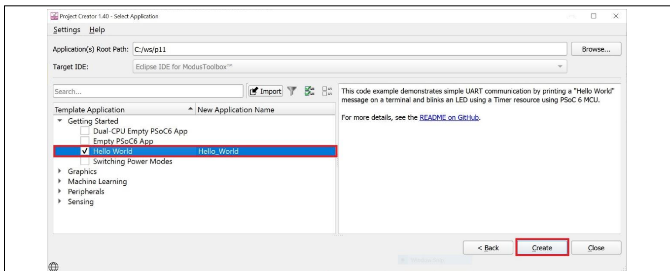
Figure 12 Creating a new application: Select Application
