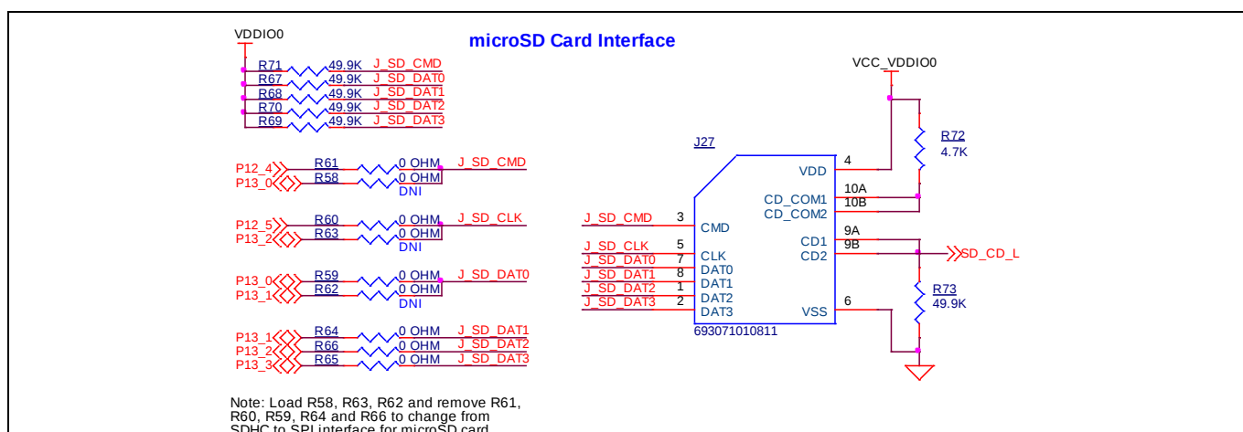
Figure 38 microSD card section
