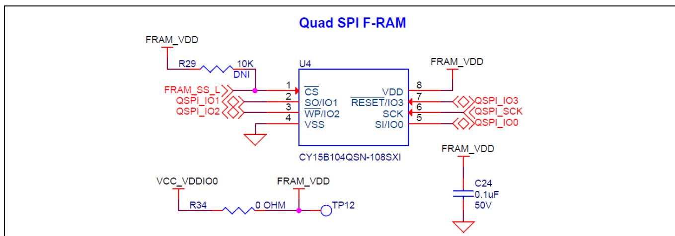
Figure 36 Quad SPI F-RAM
