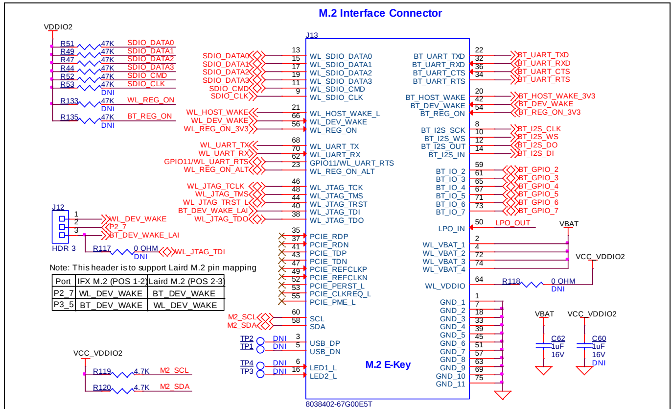
Figure 20 M.2 interface connector
