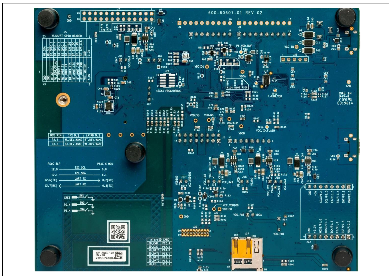
Figure 3 PSoC™ 62S2 evaluation board – bottom view
