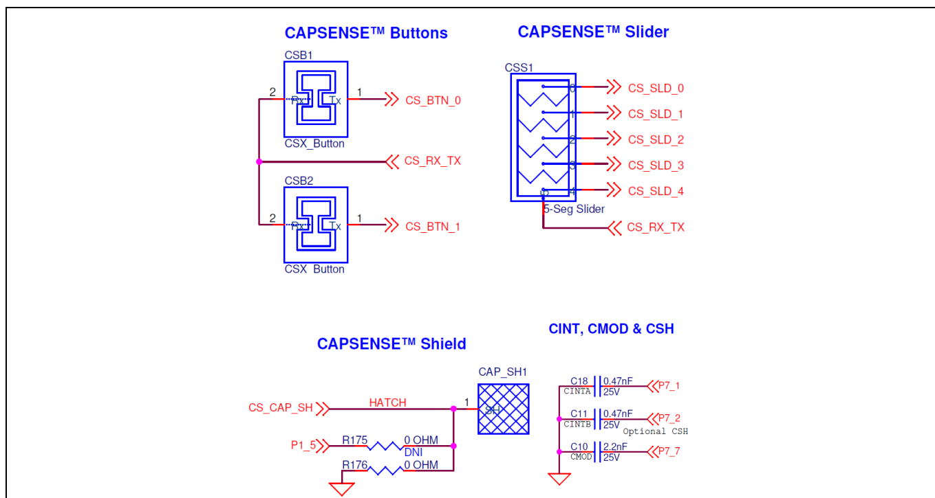
Figure 31 CAPSENSE™ circuit
