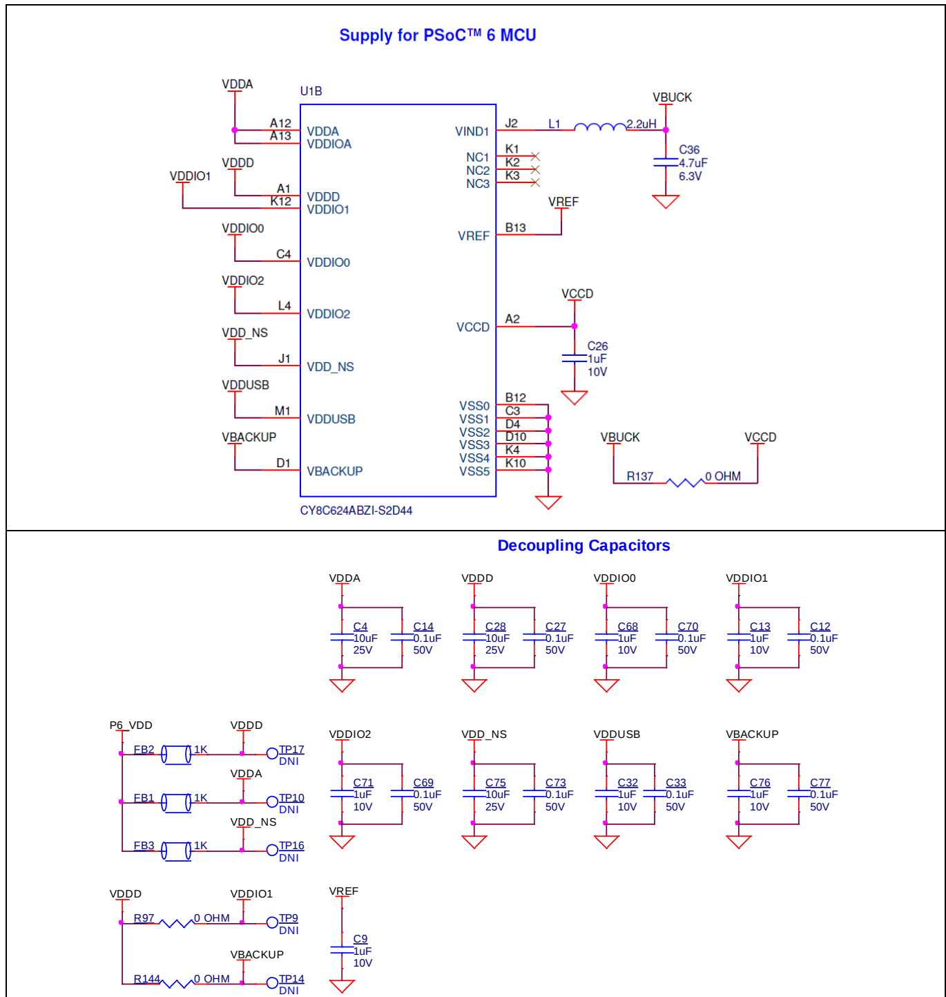
Figure 19 PSoC™ 6 MCU
