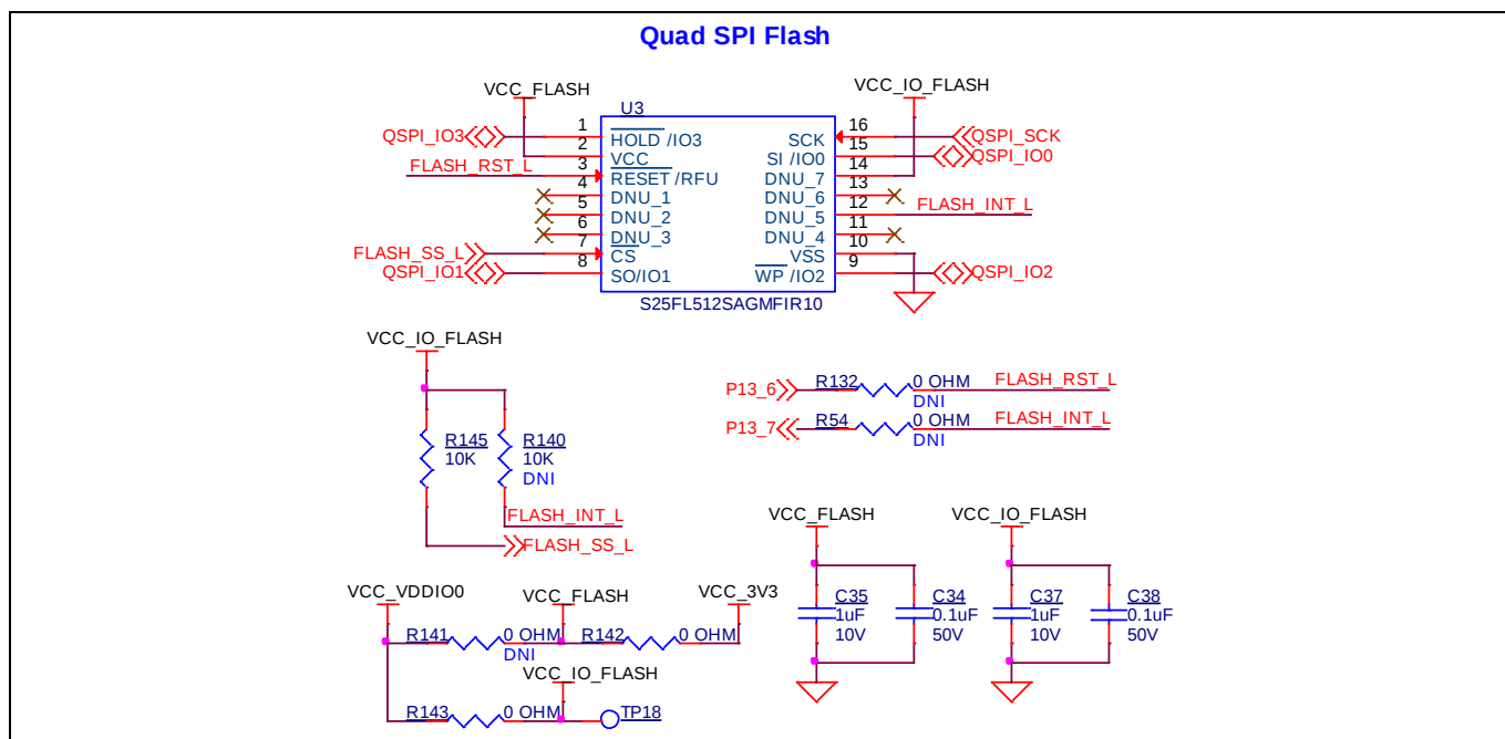
Figure 35 QSPI NOR flash
