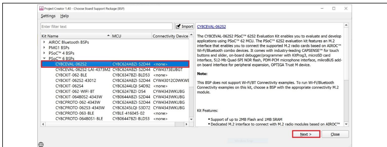
Figure 11 Creating a new application: Choose Board Support Package
