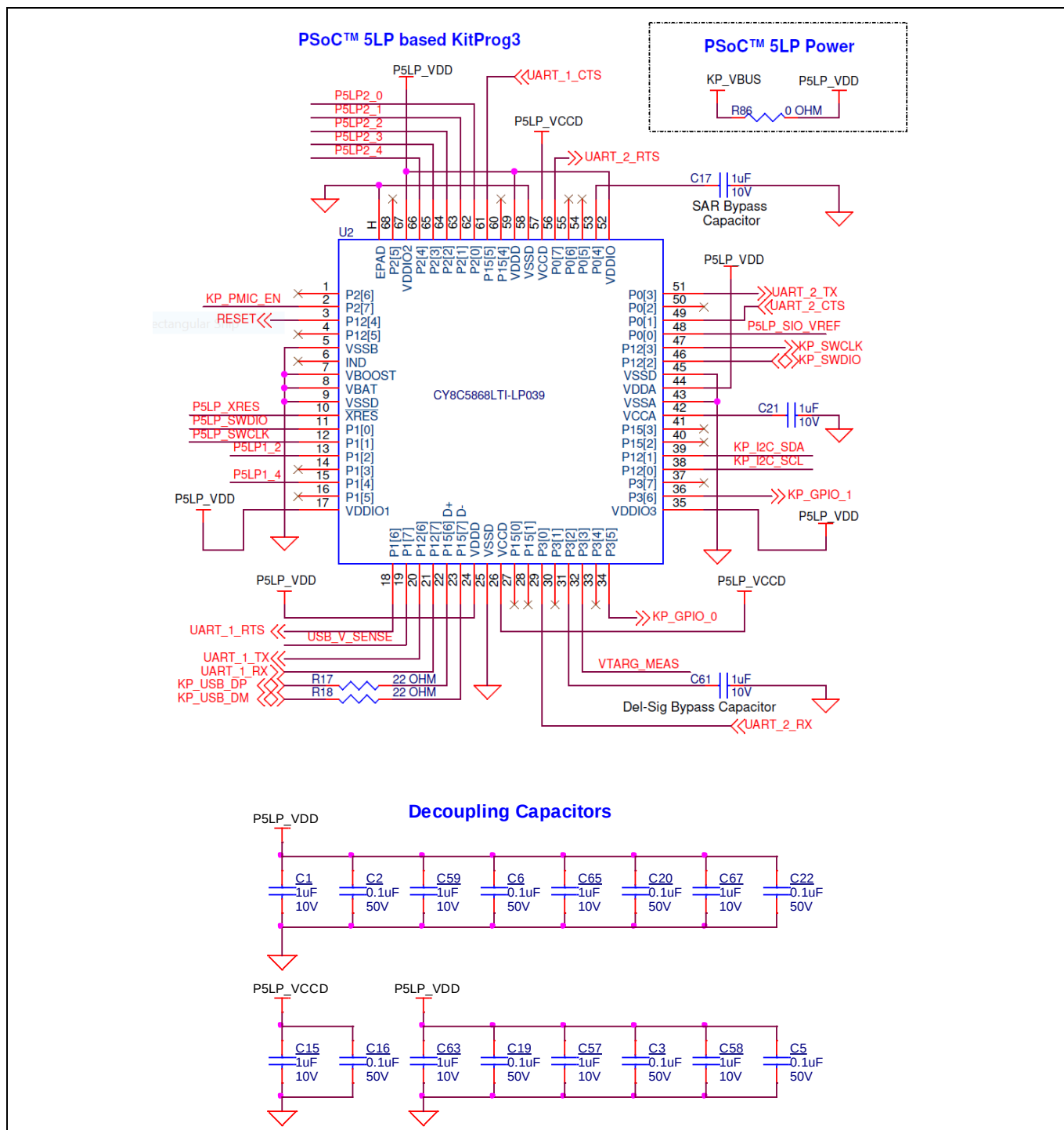
Figure 21 PSoC™ 5LP-based KitProg3 (U2)
