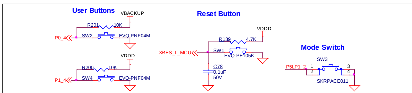
Figure 33 Push buttons
