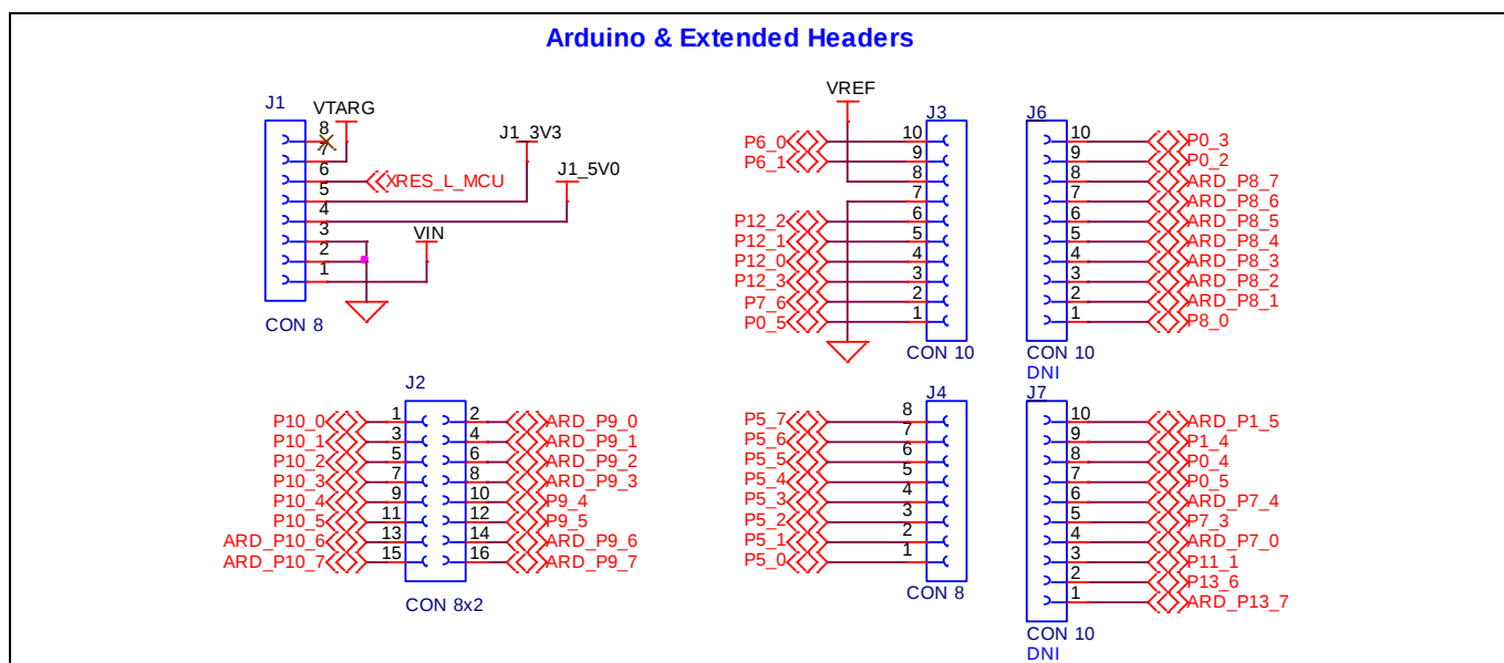
Figure 29 Headers compatible with Arduino Uno R3
