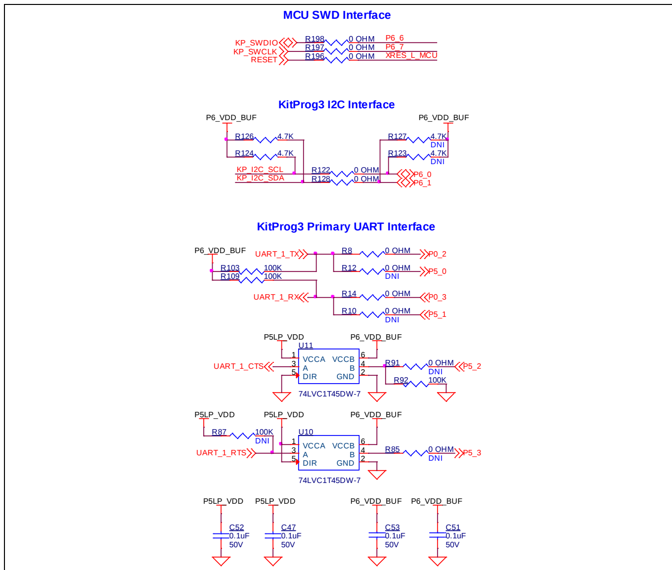
Figure 22 Programming and serial interface connections
