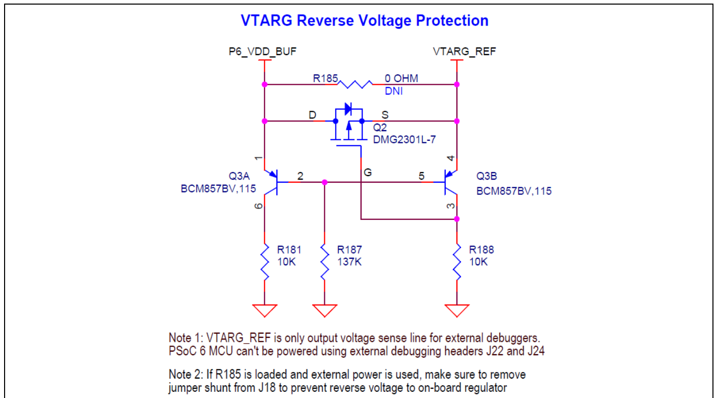
Figure 48 VTARG reverse voltage protection
