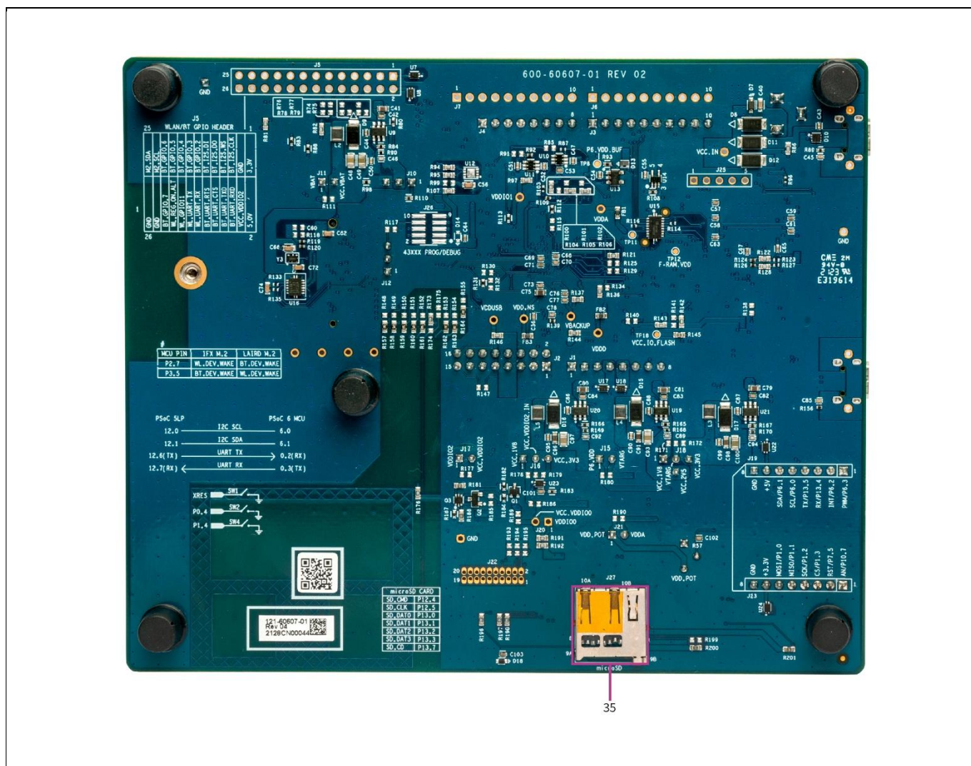
Figure 8 PSoC™ 62S2 evaluation board – bottom view
