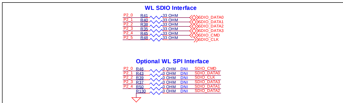
Figure 45 WLAN interface SPI multiplexing
