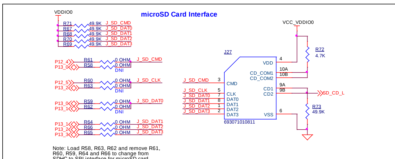
Figure 44 microSD card SPI multiplexing
