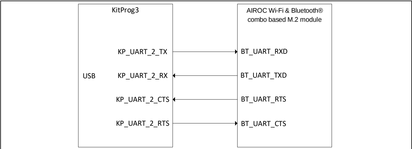
Figure 17 UART connection between KitProg3 and AIROC™ Wi-Fi & Bluetooth® combo-based M.2 module
