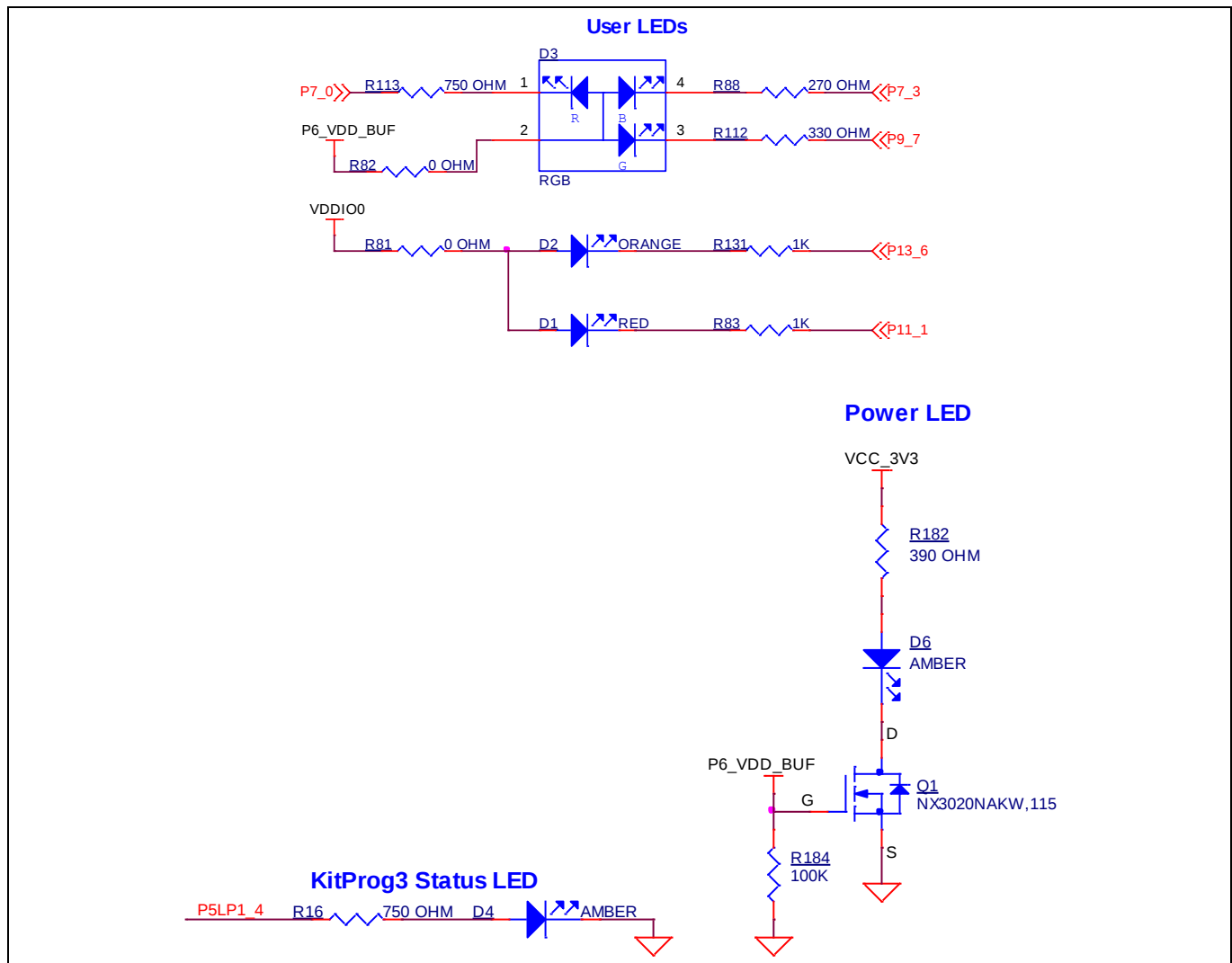
Figure 32 LEDs
