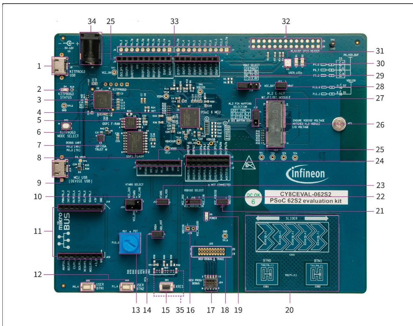
Figure 2 PSoC™ 62S2 evaluation board – top view
