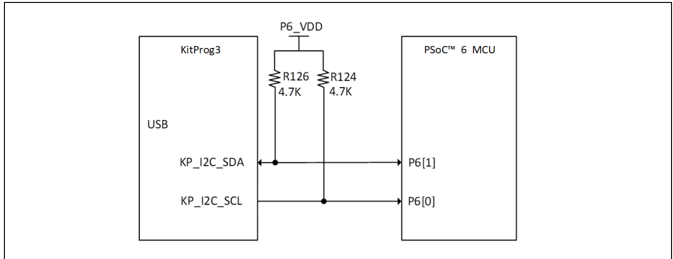
Figure 18 I2C connection between KitProg3 and PSoC™ 6 MCU
