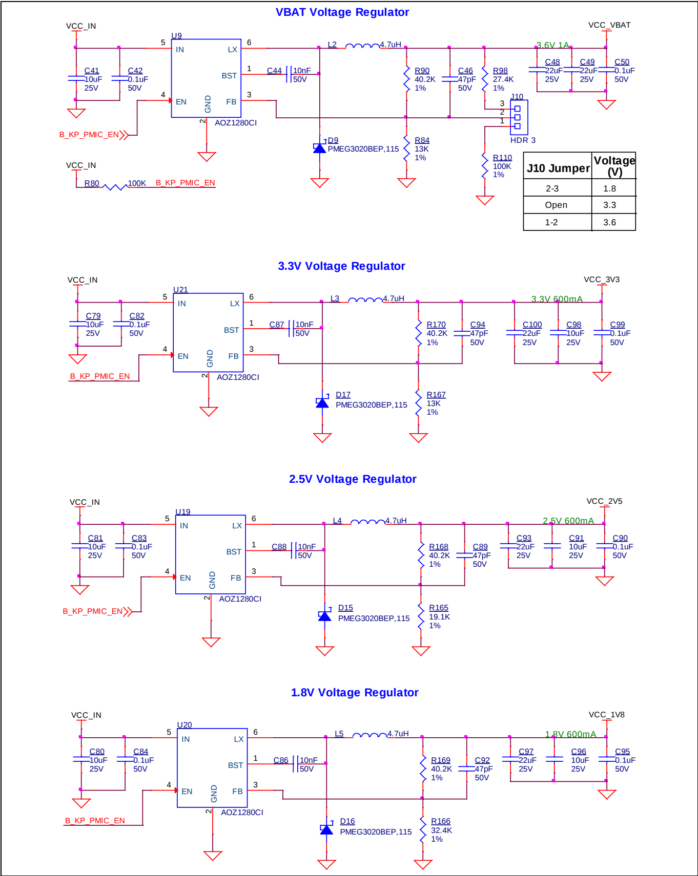
Figure 25 Voltage regulators
