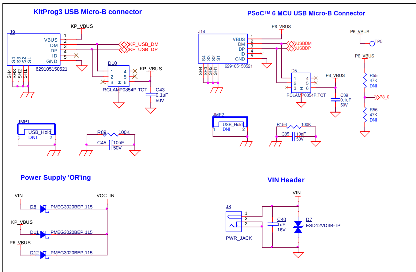
Figure 24 Power supply input and ORing
