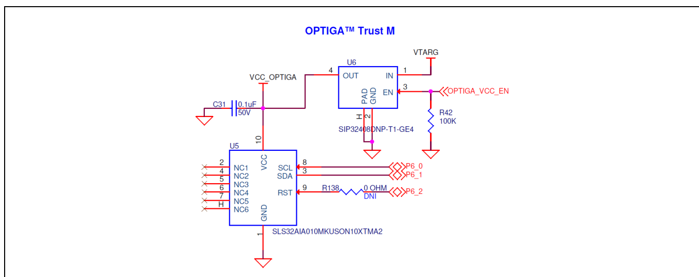
Figure 37 OPTIGA™ Trust M
