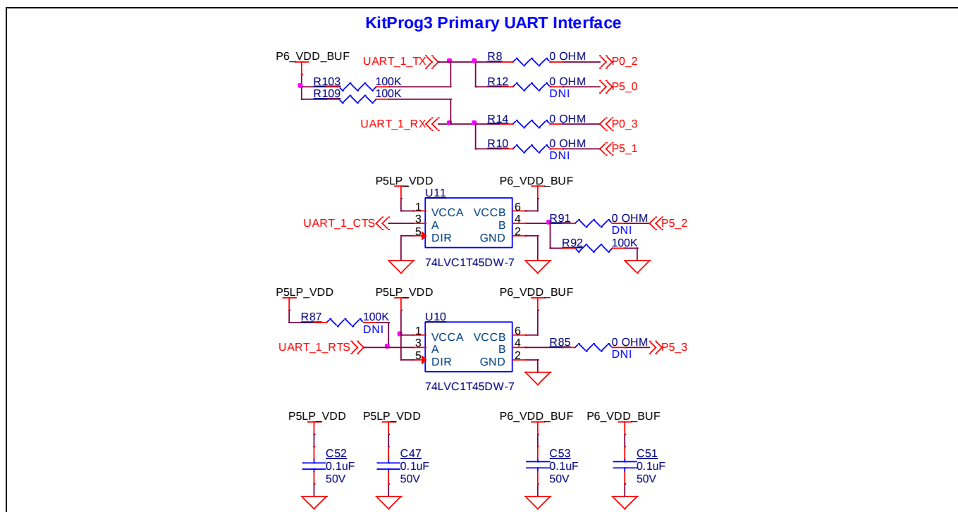
Figure 46 UART interface between PSoC™ 5LP and PSoC™ 6 MCU with flow control
