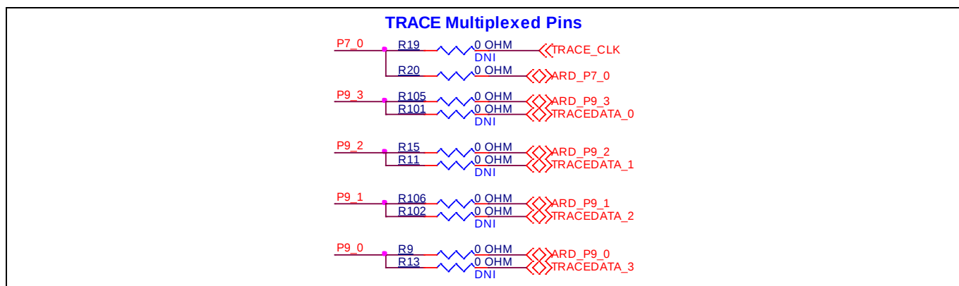
Figure 42 ETM trace header
