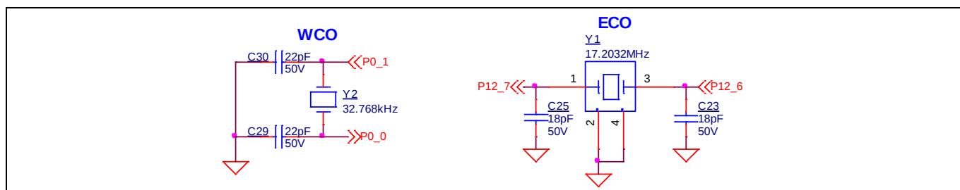
Figure 34 Crystal oscillators
