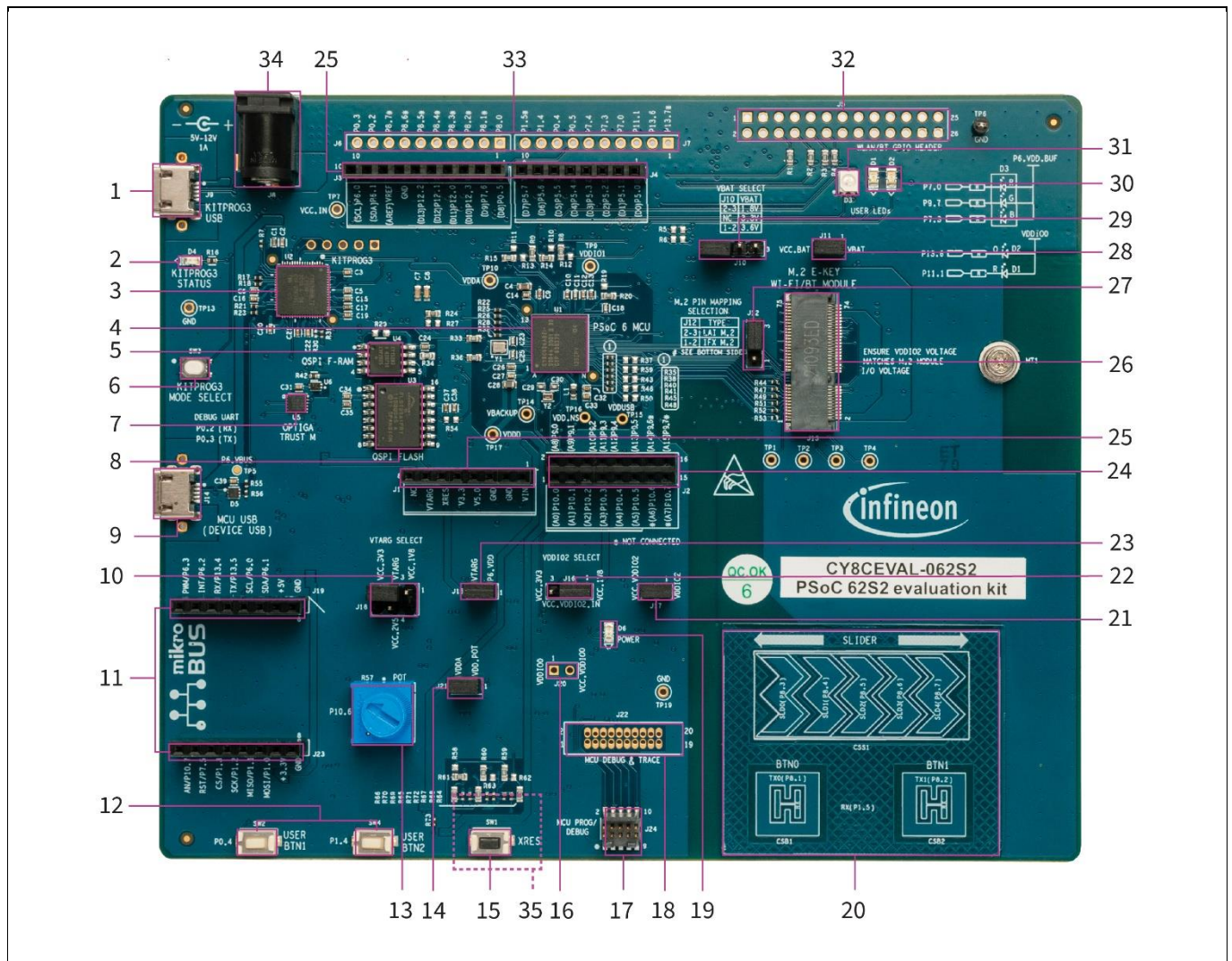
Figure 7 PSoC™ 62S2 evaluation board – top view
