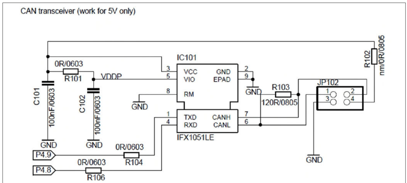
Figure 7 CAN transceiver circuitry
