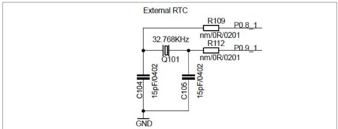
Figure 5 The external 32.768 kHz RTC crystal
