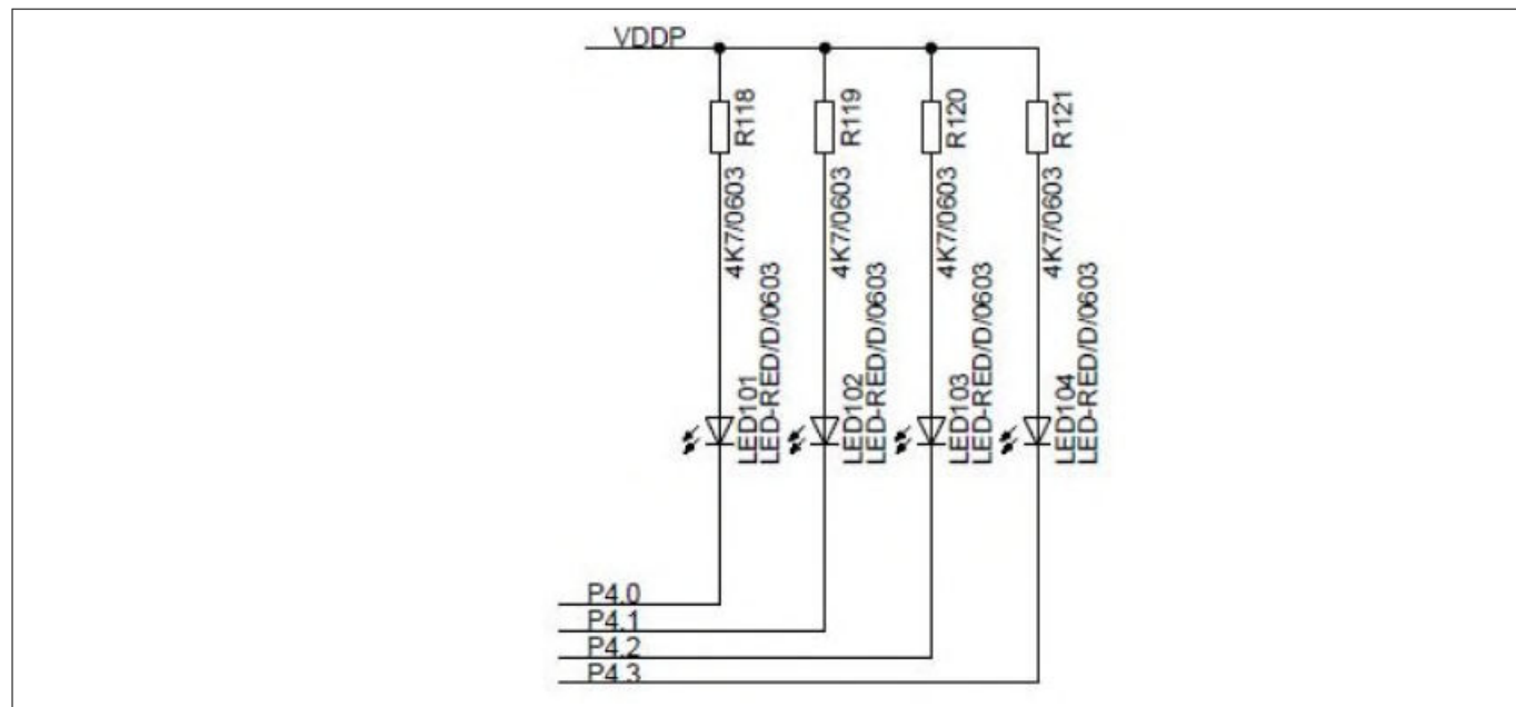
Figure 9 LEDs circuit
