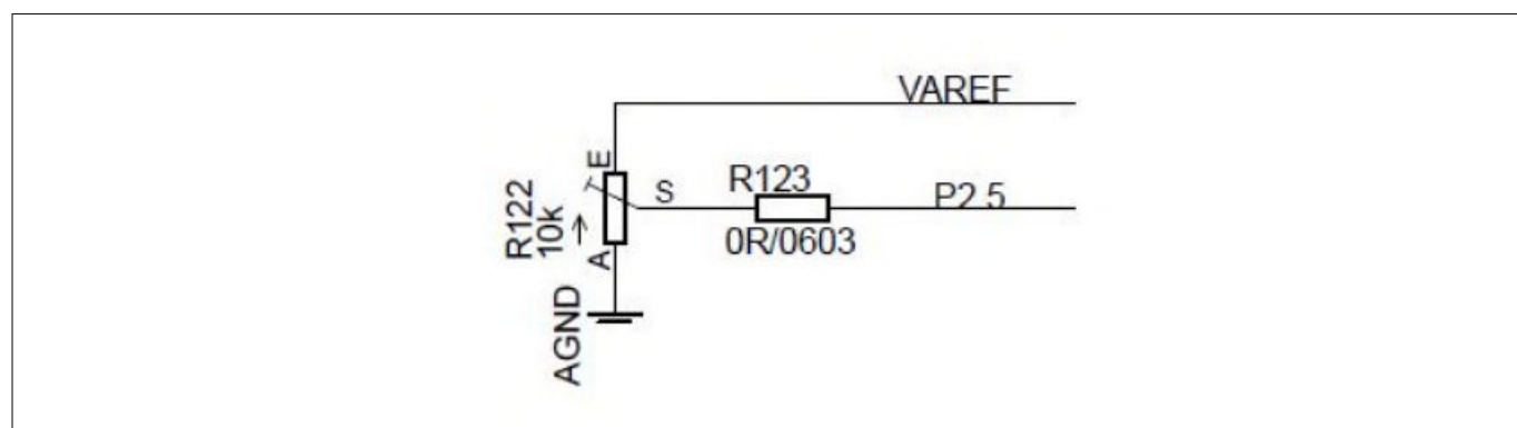
Figure 10 Potentiometer Circuit
