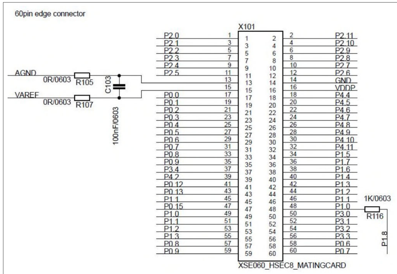
Figure 11 Pinout of the 2x30 pin edge connector
