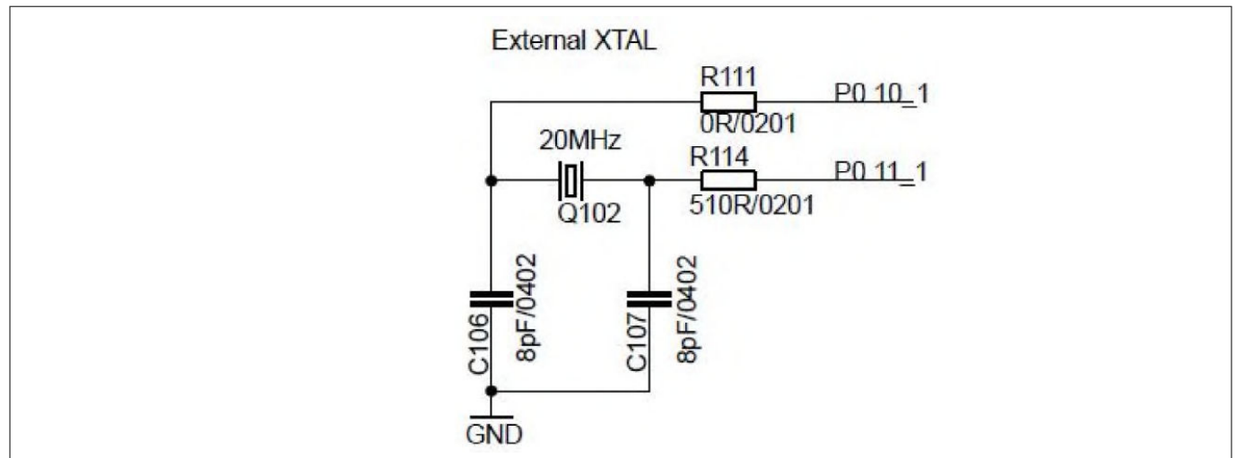
Figure 4 The external 20 MHz crystal
