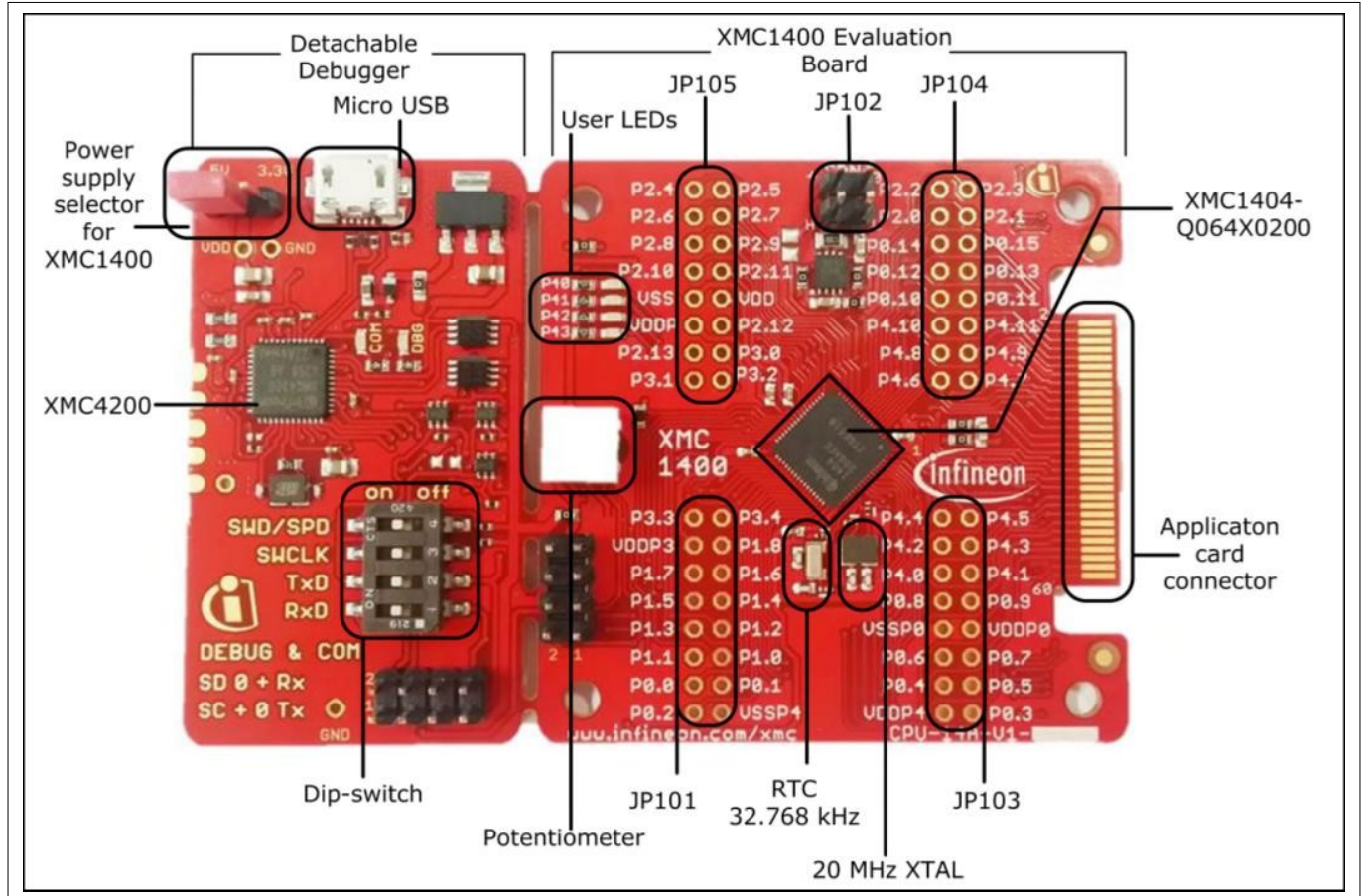
Figure 2 XMC1400 Boot Kit
