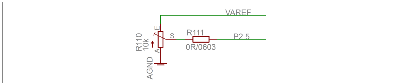
Figure 5 Potentiometer Circuit
