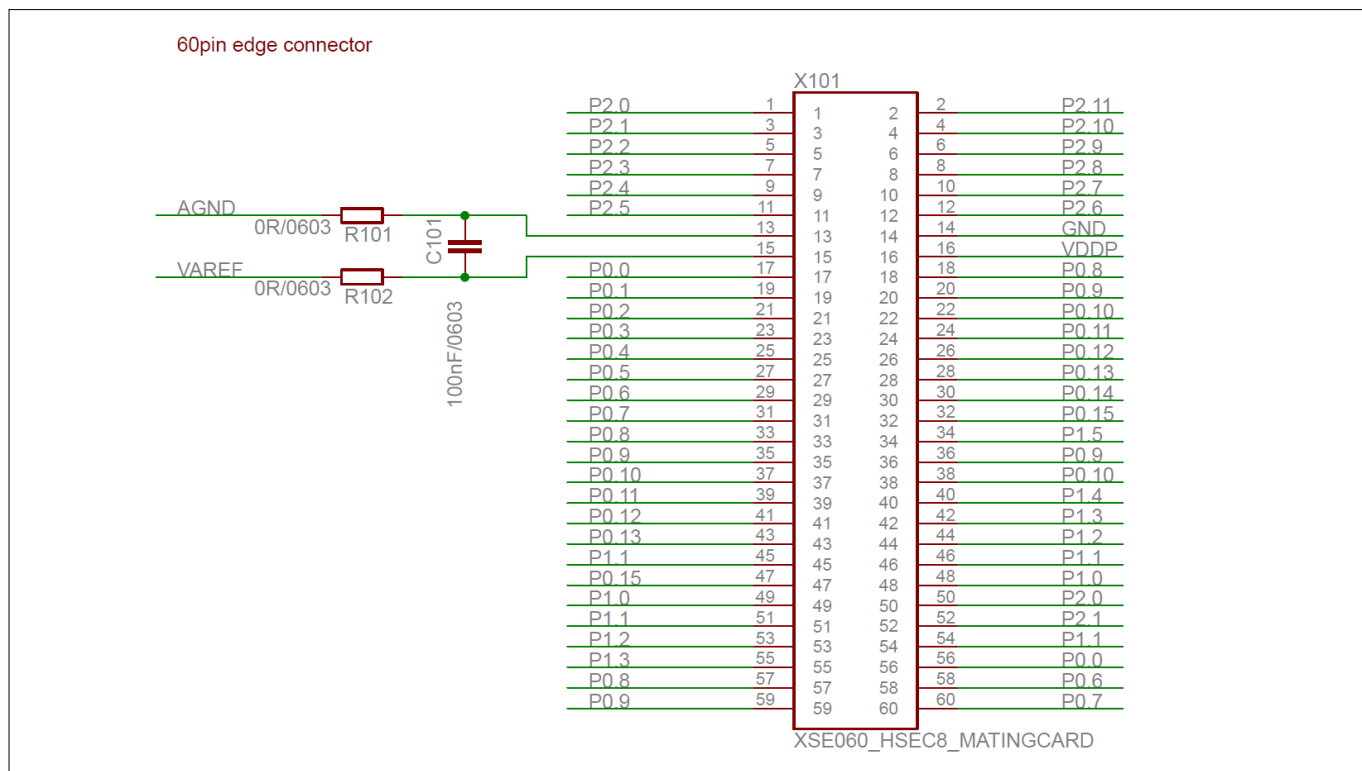
Figure 6 Pinout of the 2x30 pin edge connector
