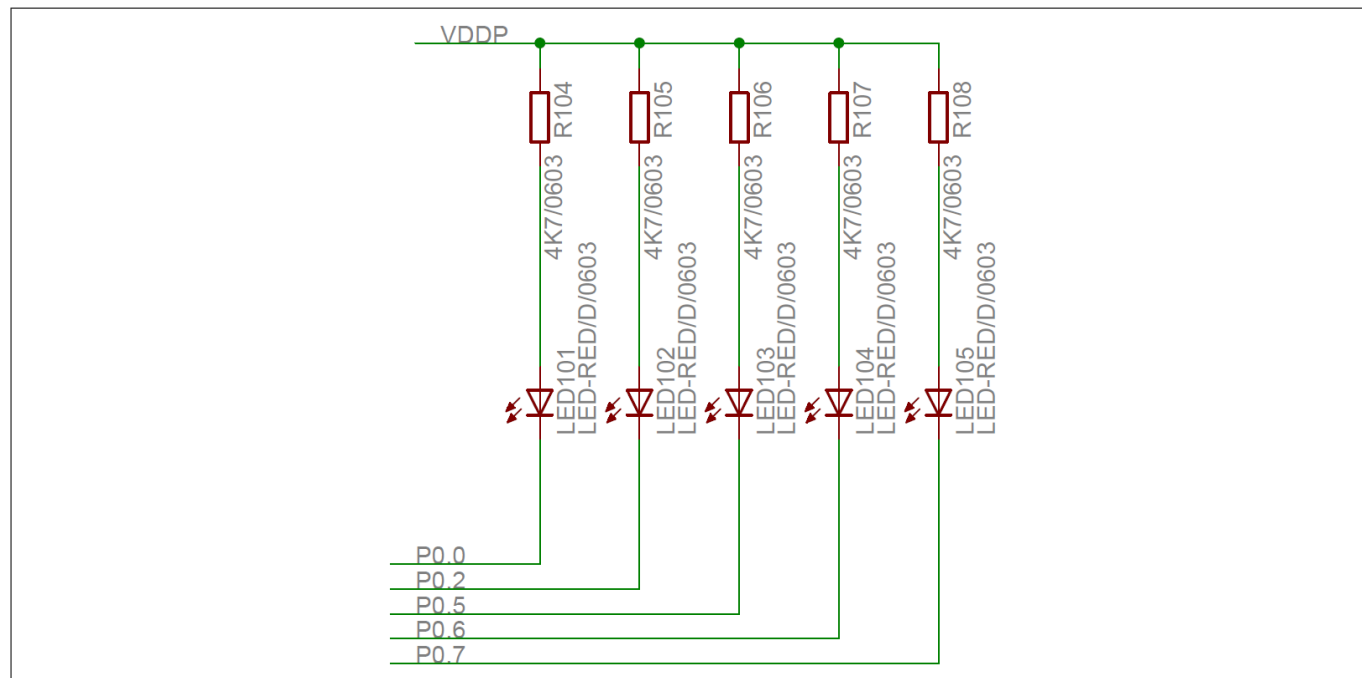
Figure 4 LEDs circuit
