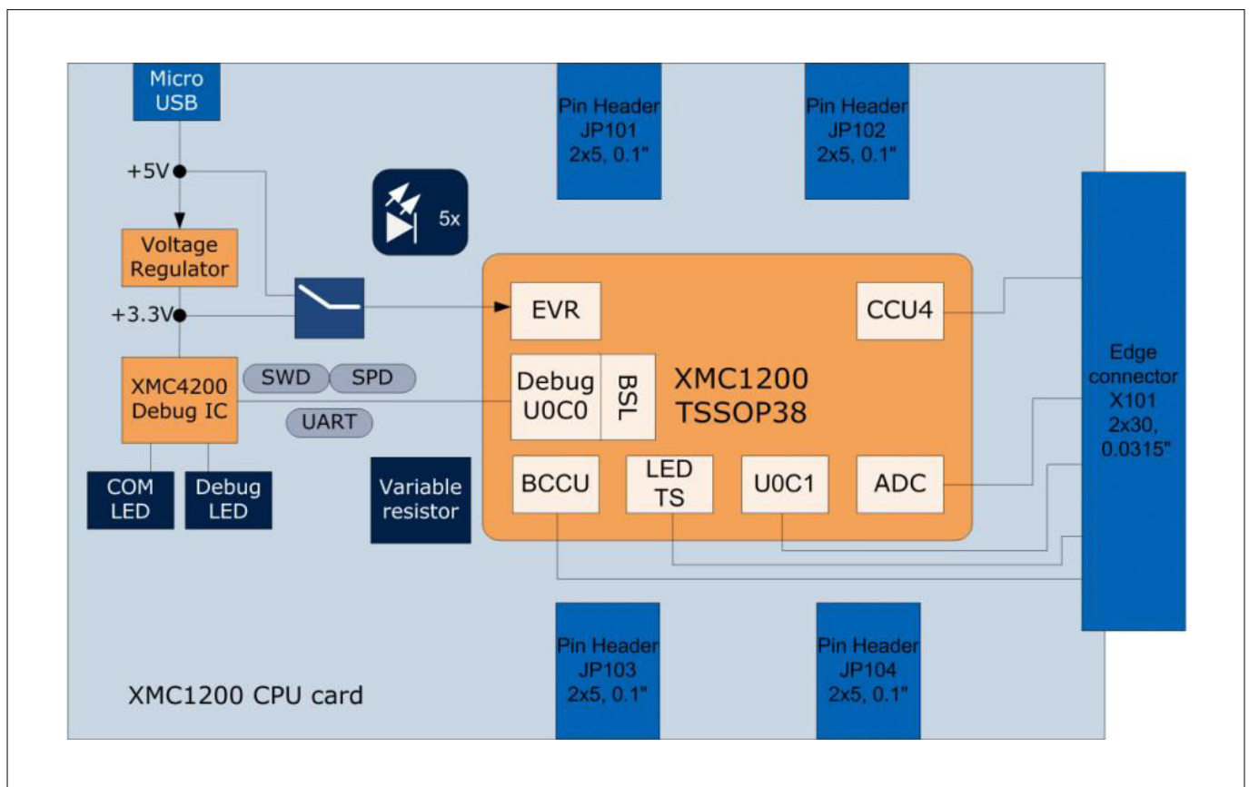
Figure 1 Block Diagram of XMC1200 CPU Card
