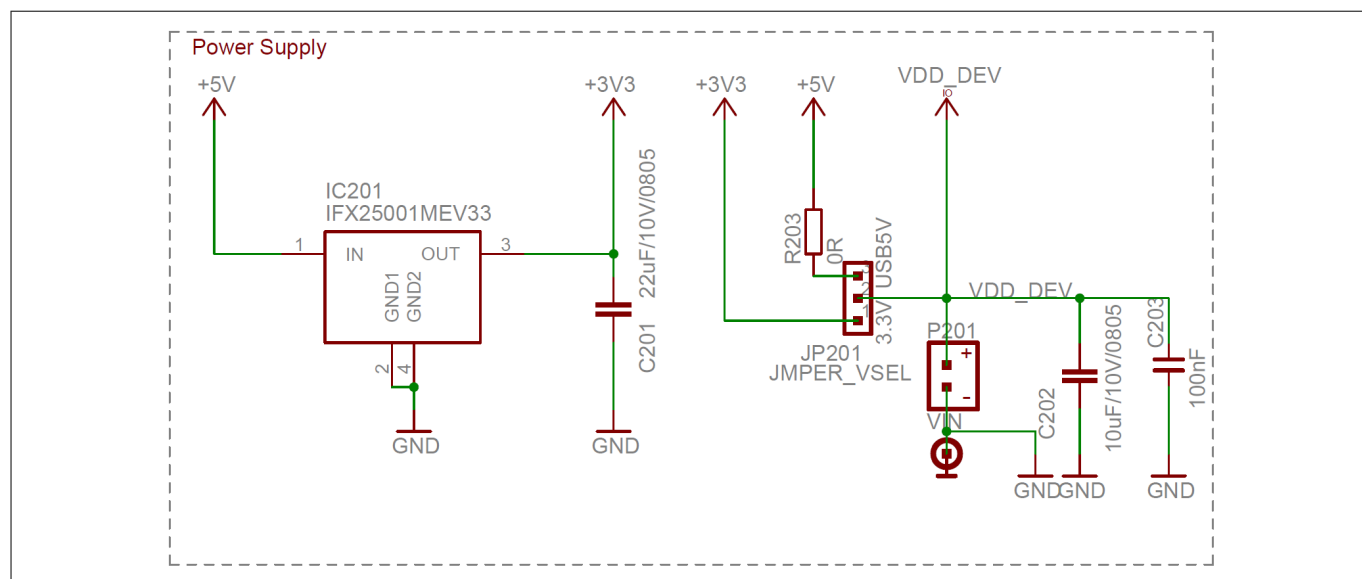
Figure 3 Power Supply circuit
