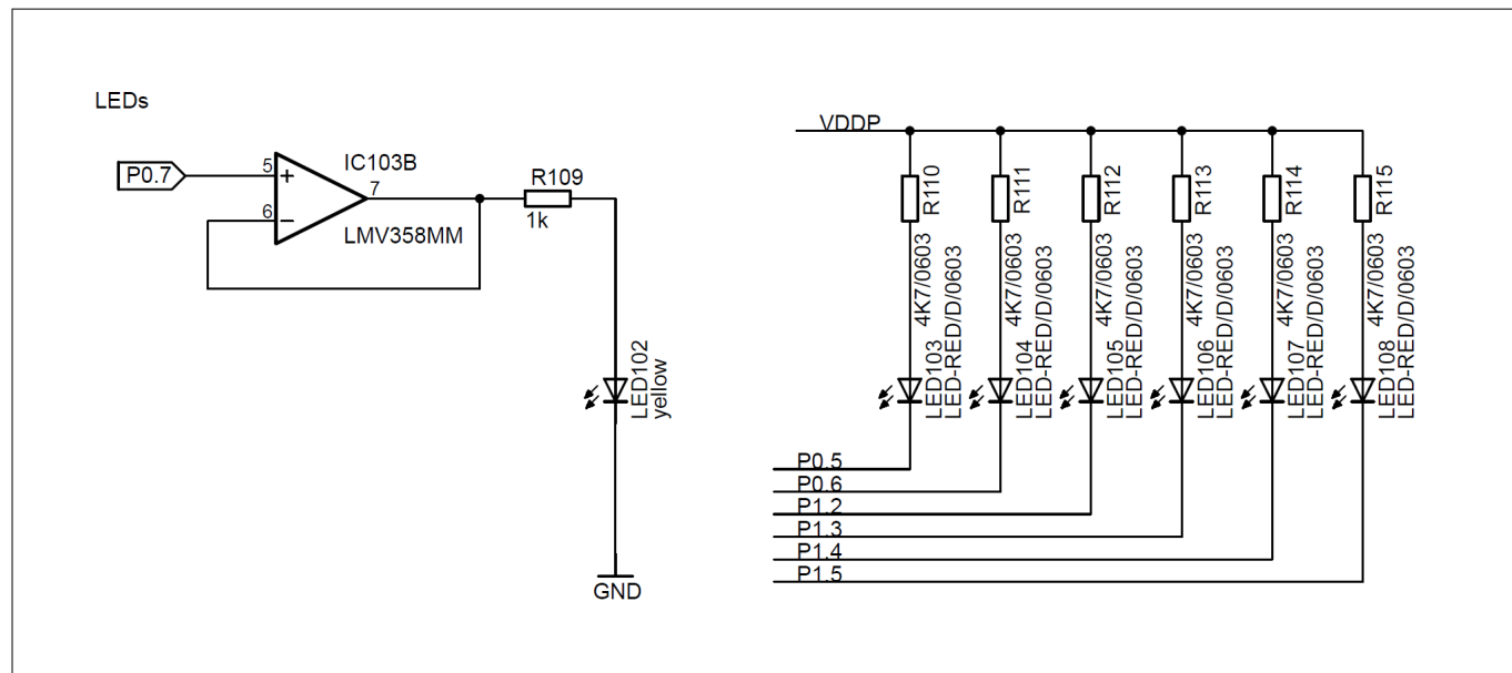
Figure 7 LEDs Circuit
