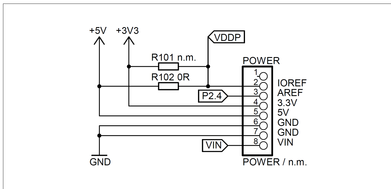
Figure 5 POWER connector
