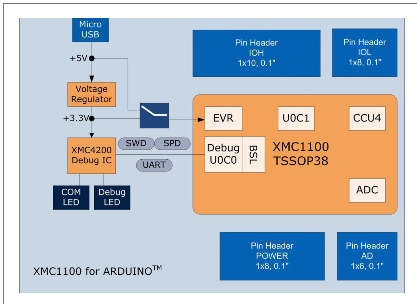
Figure 1 Block Diagram of XMC1100 CPU Card for Arduino™
