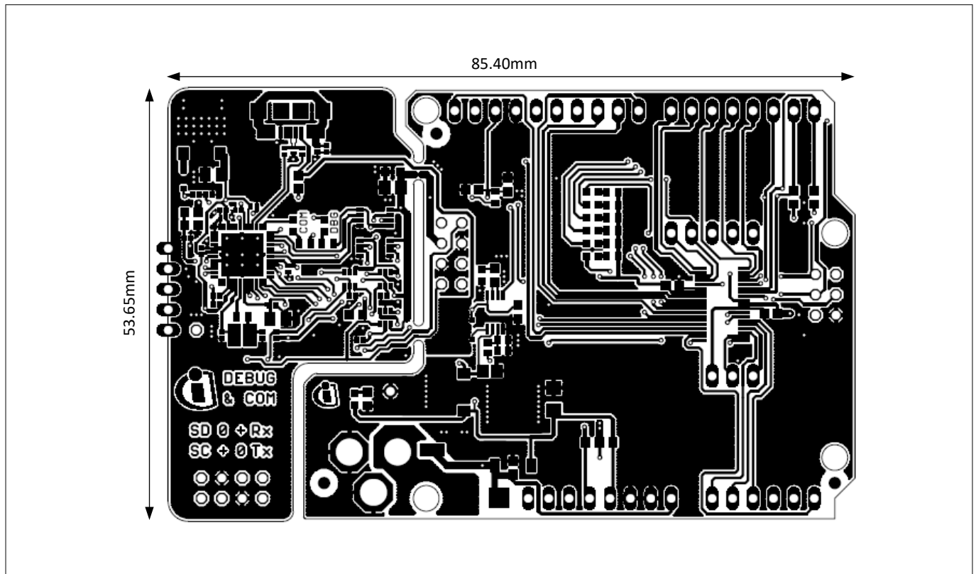
Figure 11 XMC1100 CPU Card for Arduino™ layout and geometry
