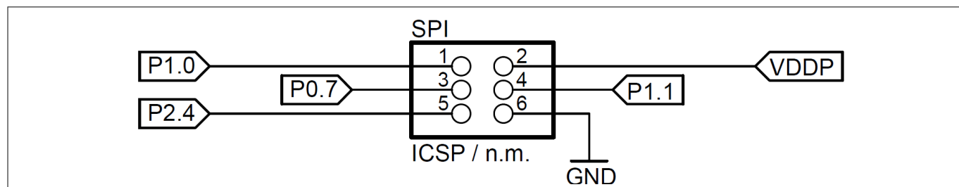
Figure 6 ICSP connector
