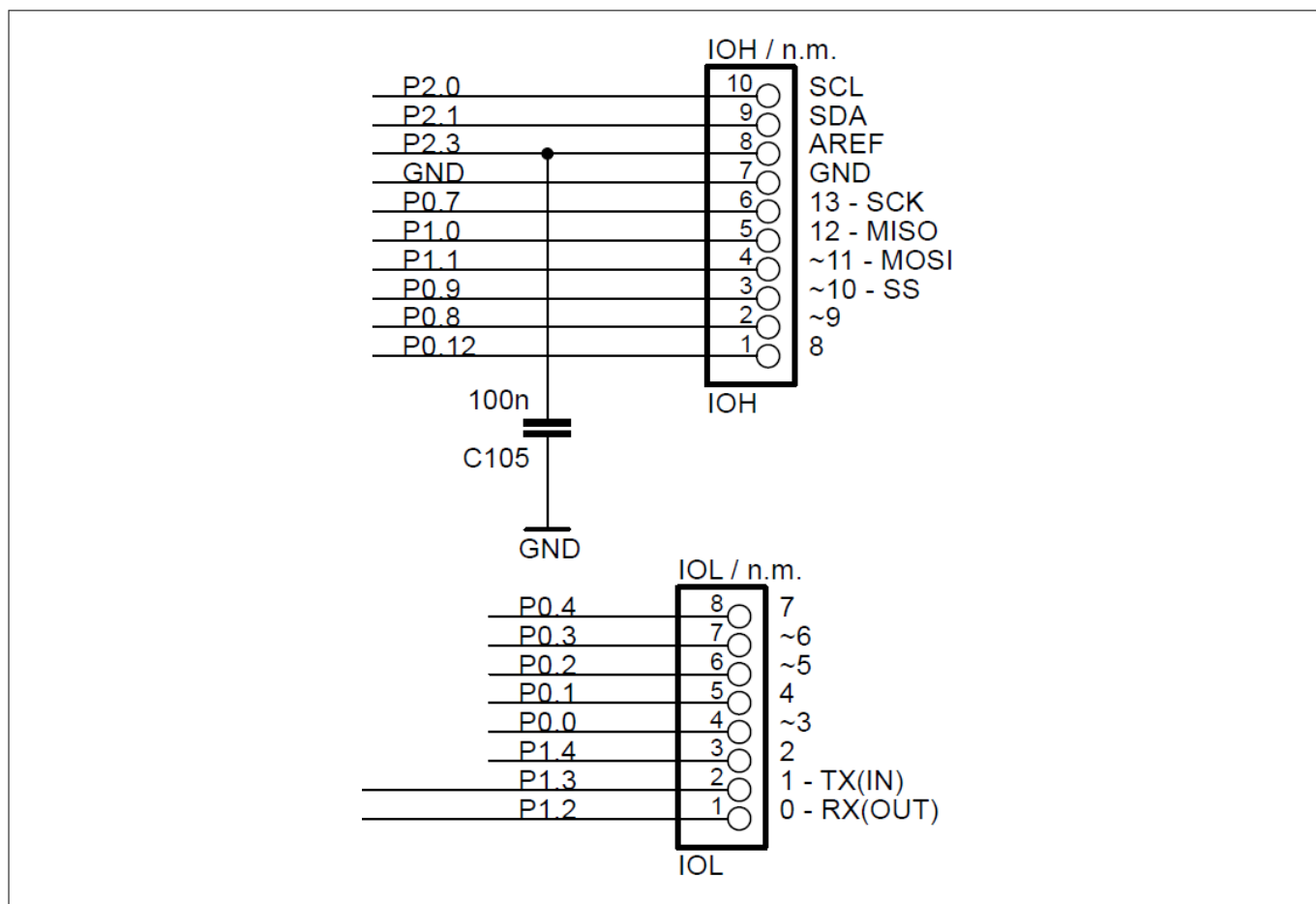
Figure 3 Digital IO connectors IOH, IOL
