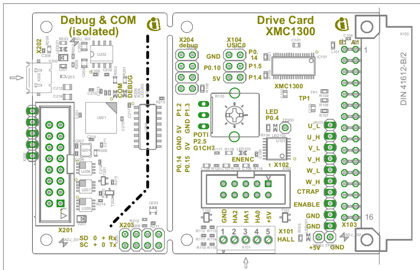
Figure 18 Component Placement
