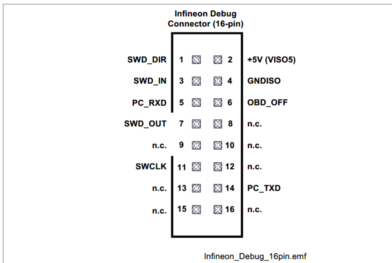
Figure 9 Infineon Debug Connector (16-pin)
