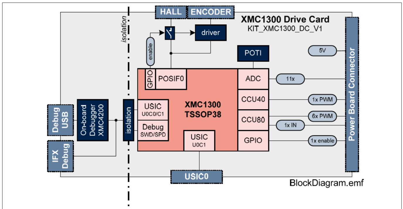
Figure 1 Block Diagram of KIT_XMC1300_DC_V1
