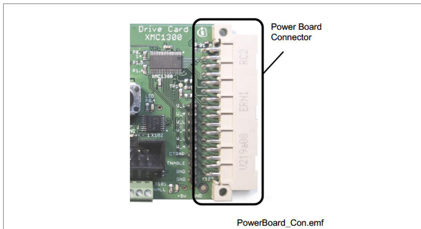
Figure 14 Power Board Connector
