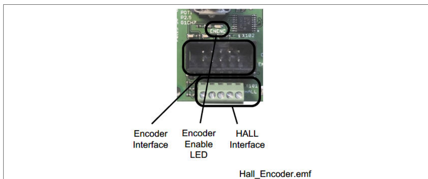
Figure 12 Hall Sensor and Encoder Connectors
