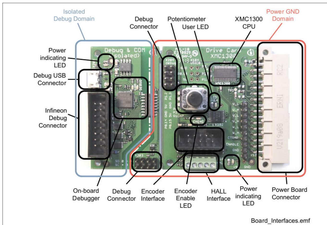
Figure 2 XMC1300 Drive Card (KIT_XMC1300_DC_V1)
