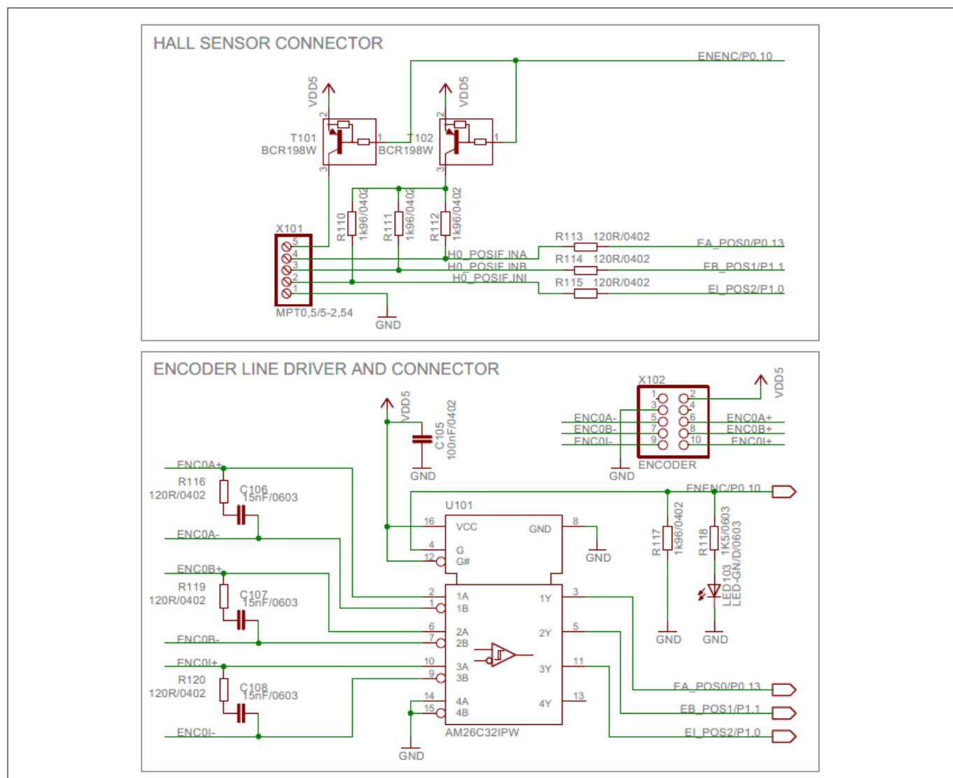
Figure 13 Hall Sensor and Encoder Interface Circuitry
