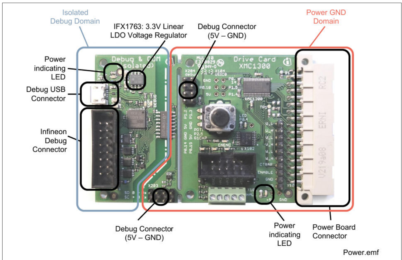
Figure 3 Power Supply Concept and Powering Options
