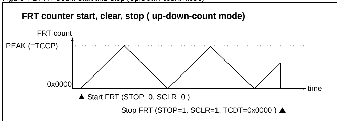
Figure 4-2 FRT Count Start and Stop (Up/Down-count Mode)
