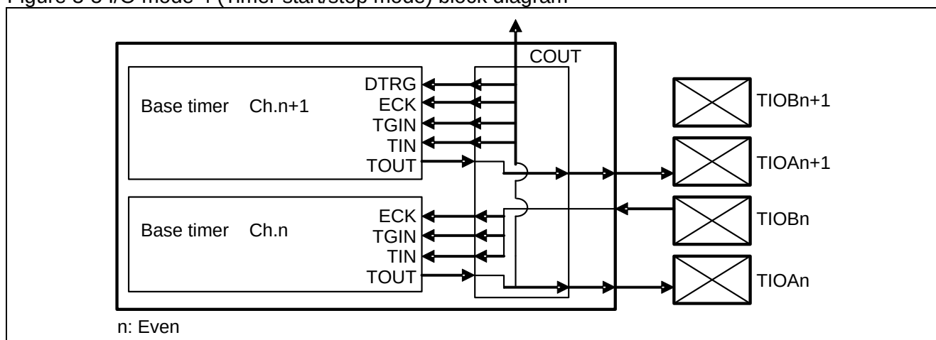
Figure 3-5 I/O mode 4 (Timer start/stop mode) block diagram
