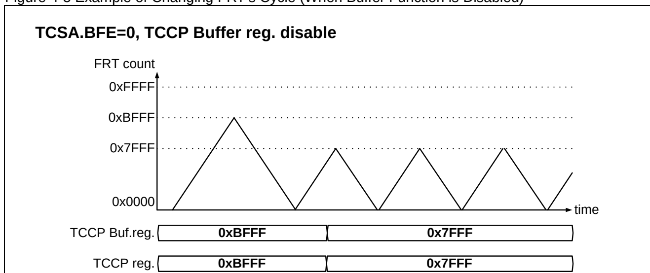
Figure 4-5 Example of Changing FRT's Cycle (When Buffer Function is Disabled)
