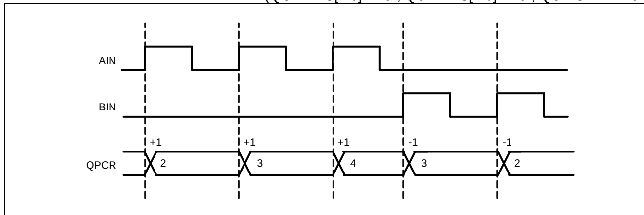
Figure 3-1 Operations in up/down count mode
