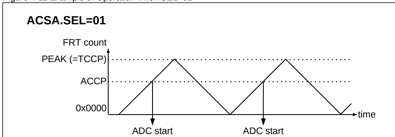
Figure 4-11 Example of Operation when SEL=01
