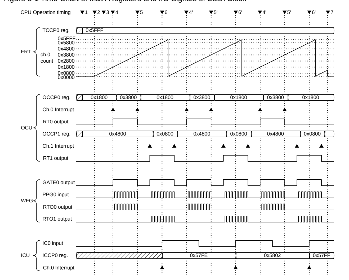
Figure 3-1 Time Chart of Main Registers and I/O Signals of Each Block
