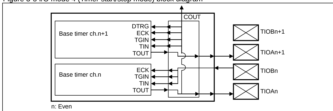
Figure 3-5 I/O mode 4 (Timer start/stop mode) block diagram
