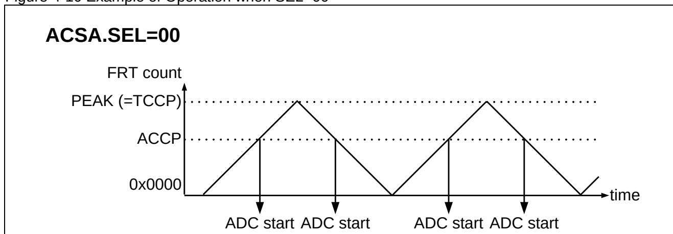
Figure 4-10 Example of Operation when SEL=00
