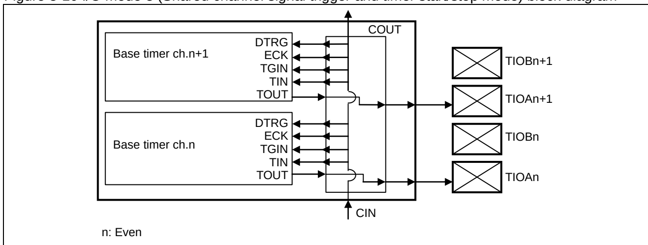
Figure 3-10 I/O mode 8 (Shared channel signal trigger and timer start/stop mode) block diagram
