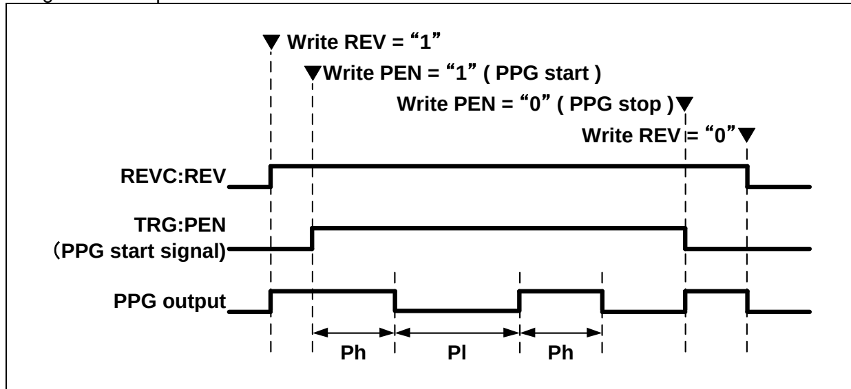
Figure 3-8 Output Waveform When REVn=1
