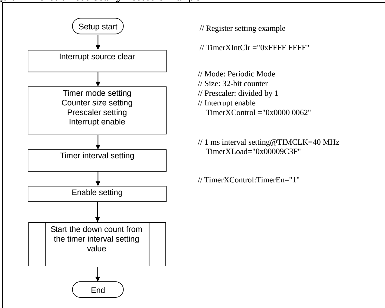
Figure 4-1 Periodic Mode Setting Procedure Example
