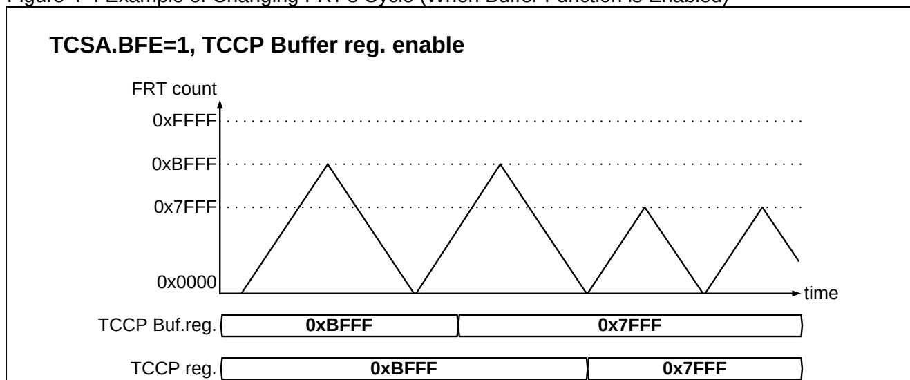
Figure 4-4 Example of Changing FRT's Cycle (When Buffer Function is Enabled)
