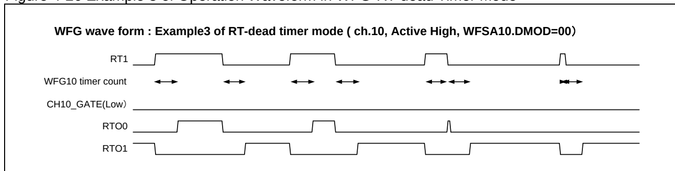
Figure 4-26 Example 3 of Operation Waveform in WFG-RT-dead Timer Mode
