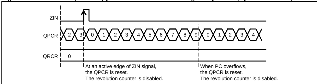
Figure 3-6 RC_Mode0 operation (QPRC Maximum Position Register QMPR=9, QCR:CGSC="0")
