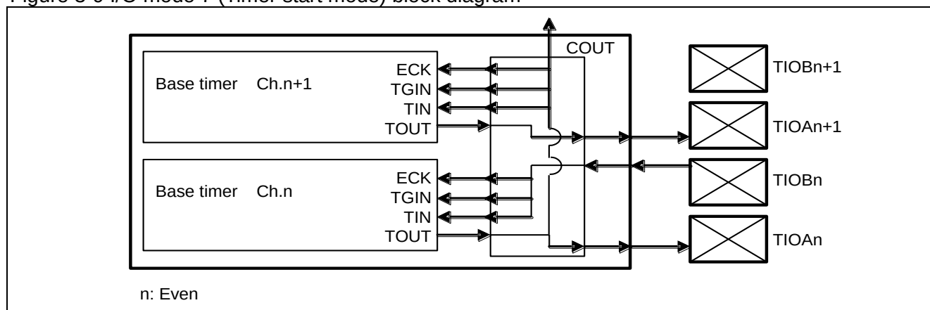
Figure 3-9 I/O mode 7 (Timer start mode) block diagram
