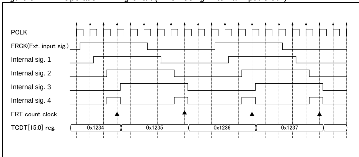
Figure 5-1 FRT Operation Timing Chart (When Using External Input Clock)
