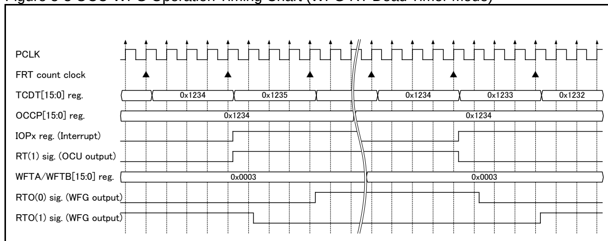
Figure 5-3 OCU-WFG Operation Timing Chart (WFG RT Dead Timer Mode)
