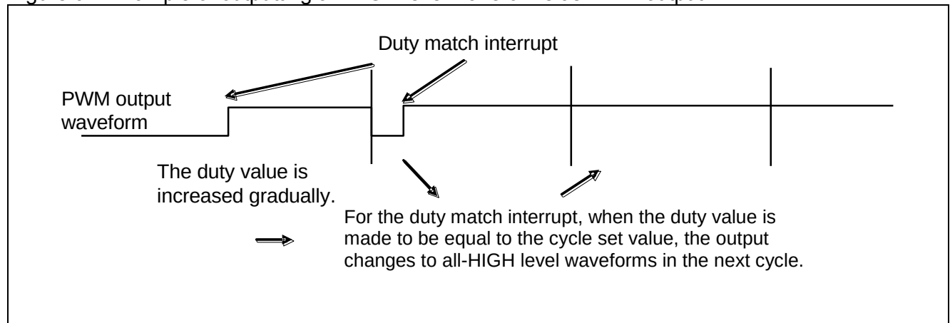
Figure 9-7 Example of outputting all-HIGH level waveforms as PWM output
