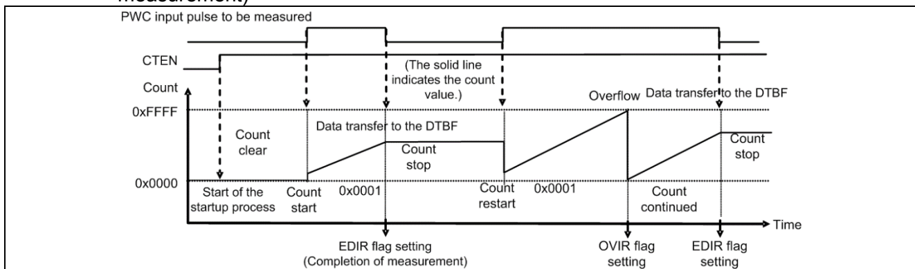
Figure 9-18 Pulse width measurement operation (continuous measurement mode/HIGH width measurement)
