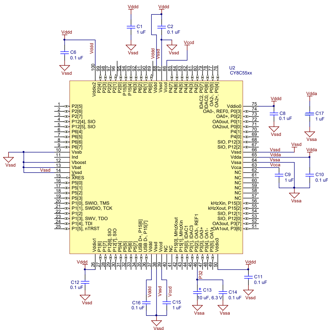
Figure A-5. 100-pin TQFP Part with Power Connections
