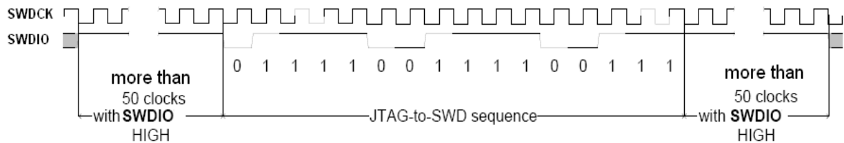
Figure 2-13. First Three Steps of JTAG to SWD Switching
