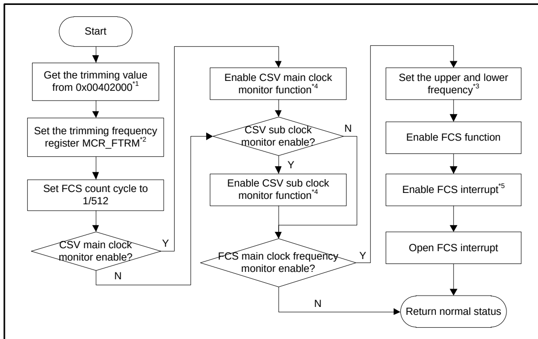
Figure 4-10: IEC60730_InitCSV Flow Chart
