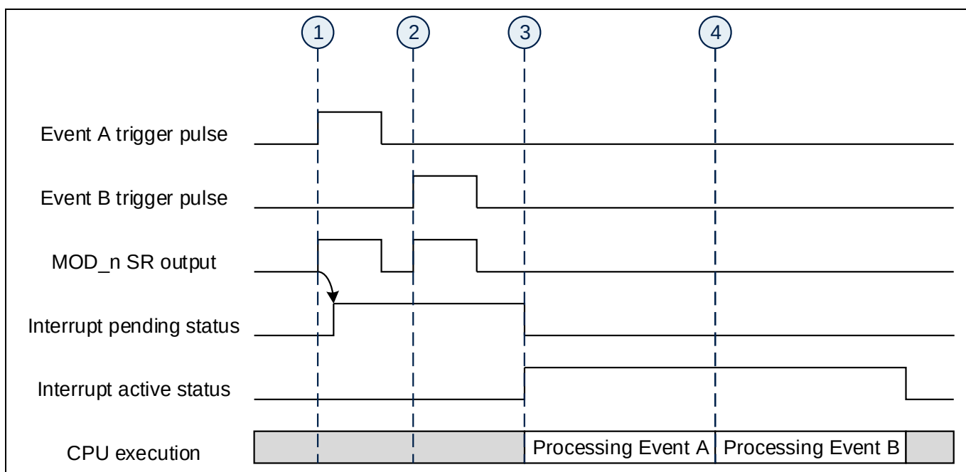
Figure 2 Events A and B occur before interrupt is serviced
