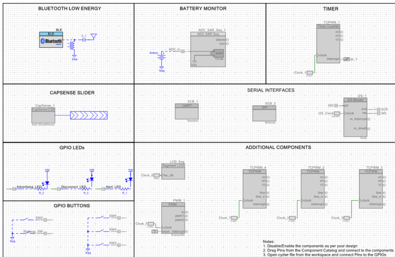
Figure 47. Schematic Configuration
