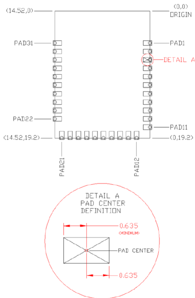
Figure 82. Host Board Required PCB Layout Pattern To Pad Center Relative to Origin
