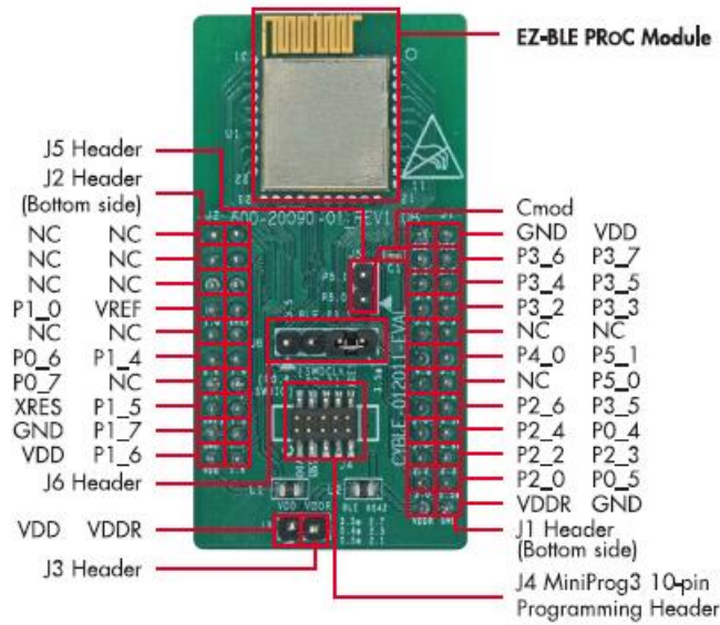
Figure 135. CYBLE-212020-EVAL Board Top Side
