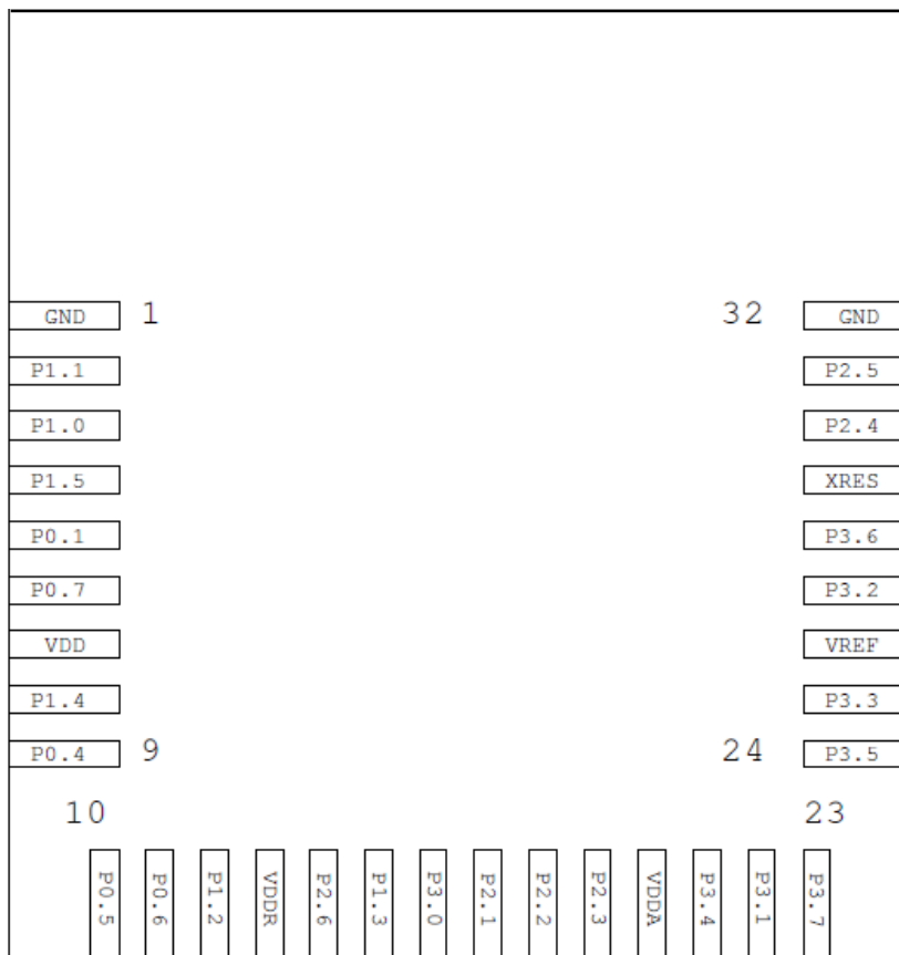
Figure 97. CYBLE-2140XX-0X Module Bottom View (Seen from Bottom)
