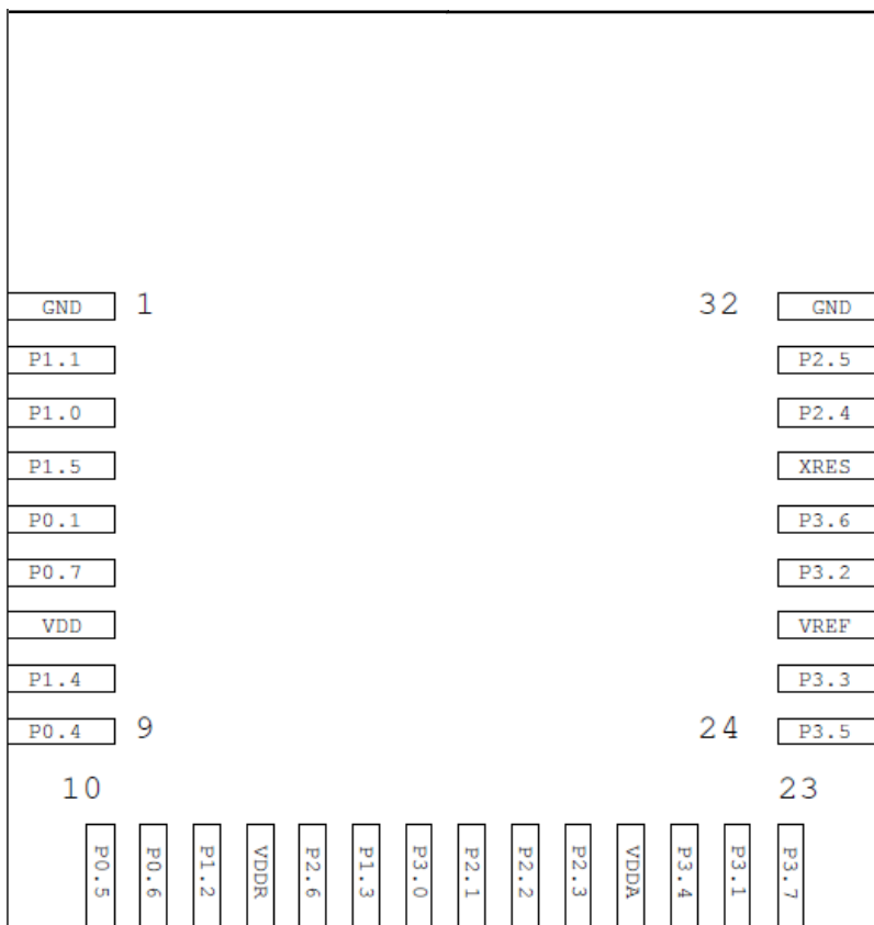
Figure 91. CYBLE-014008-00 Module Bottom View (Seen from Bottom)
