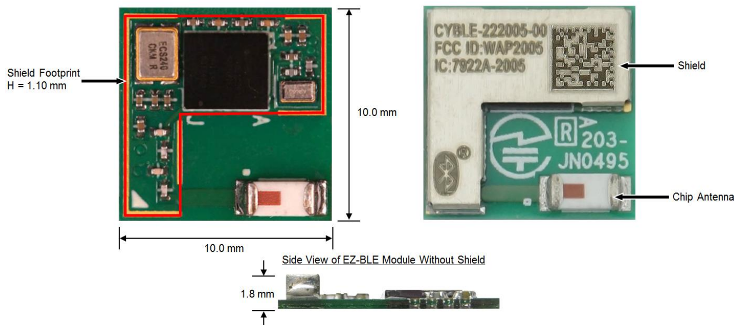
Figure 72. CYBLE-222005-00 Module Top View (with and without Shield) and Side View
