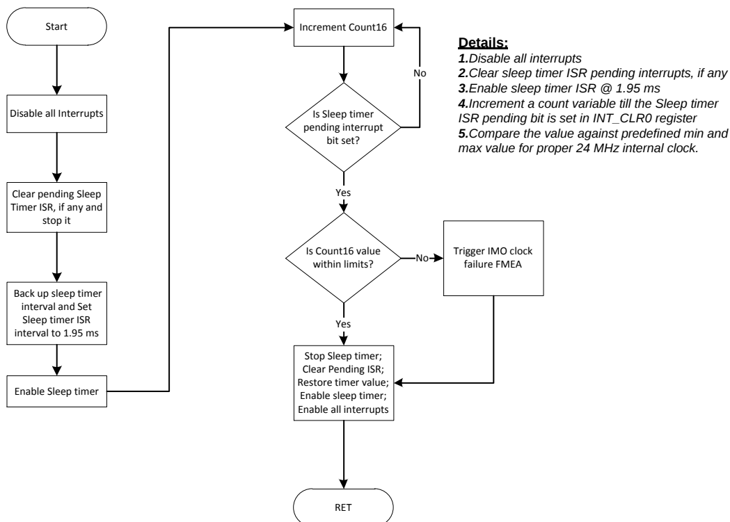
Figure 5. Clock Self-Test
