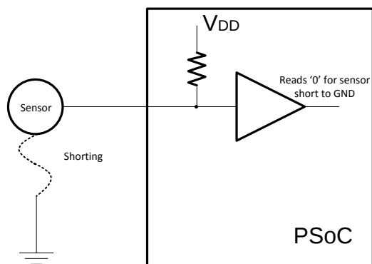
Figure 9. Sensor-to-Ground Short Detection Schematic
