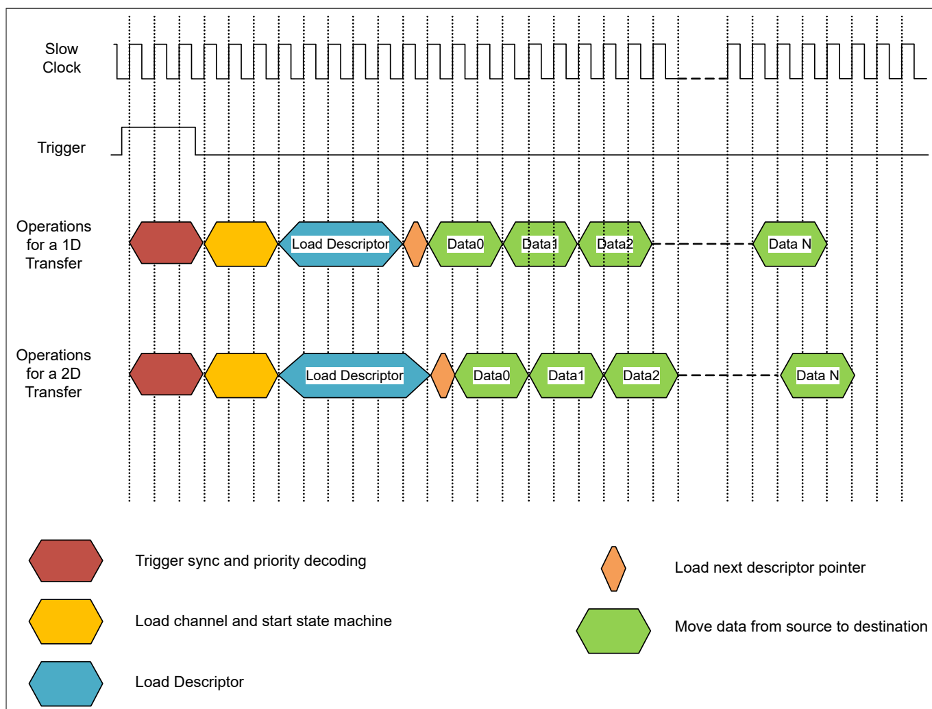
Figure 16 Timing diagram for N-byte transfer in 1D and 2D modes
