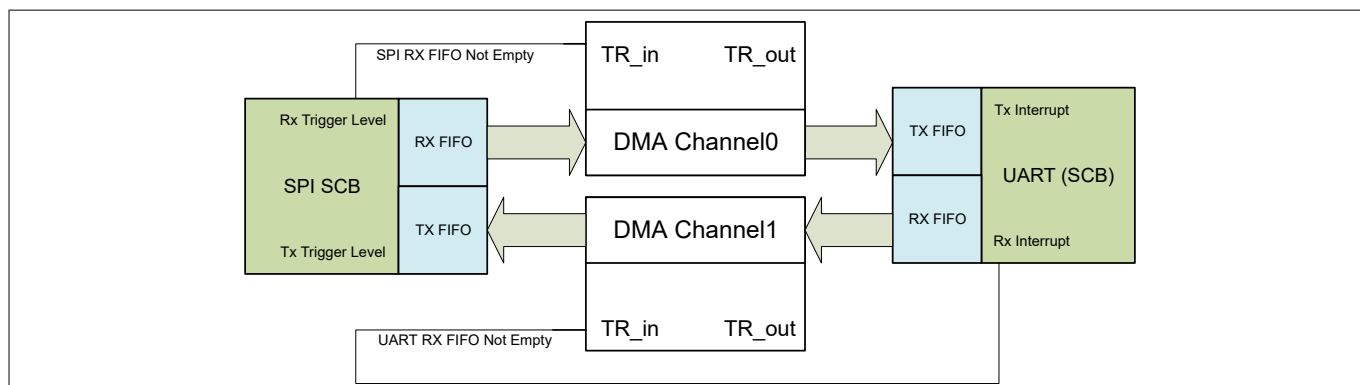
Figure 4 1-to-1 transfer
