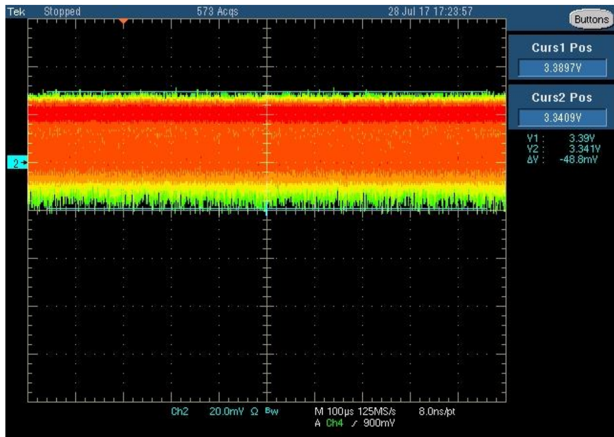
Figure 17 - UTIL_3V3 DC Ripple, 10A, sense
