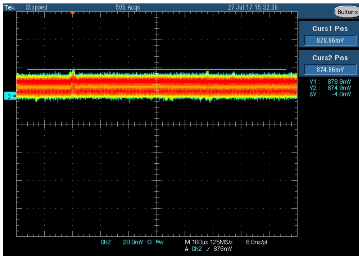
Figure 34 - MGTRAVCC ac ripple release
