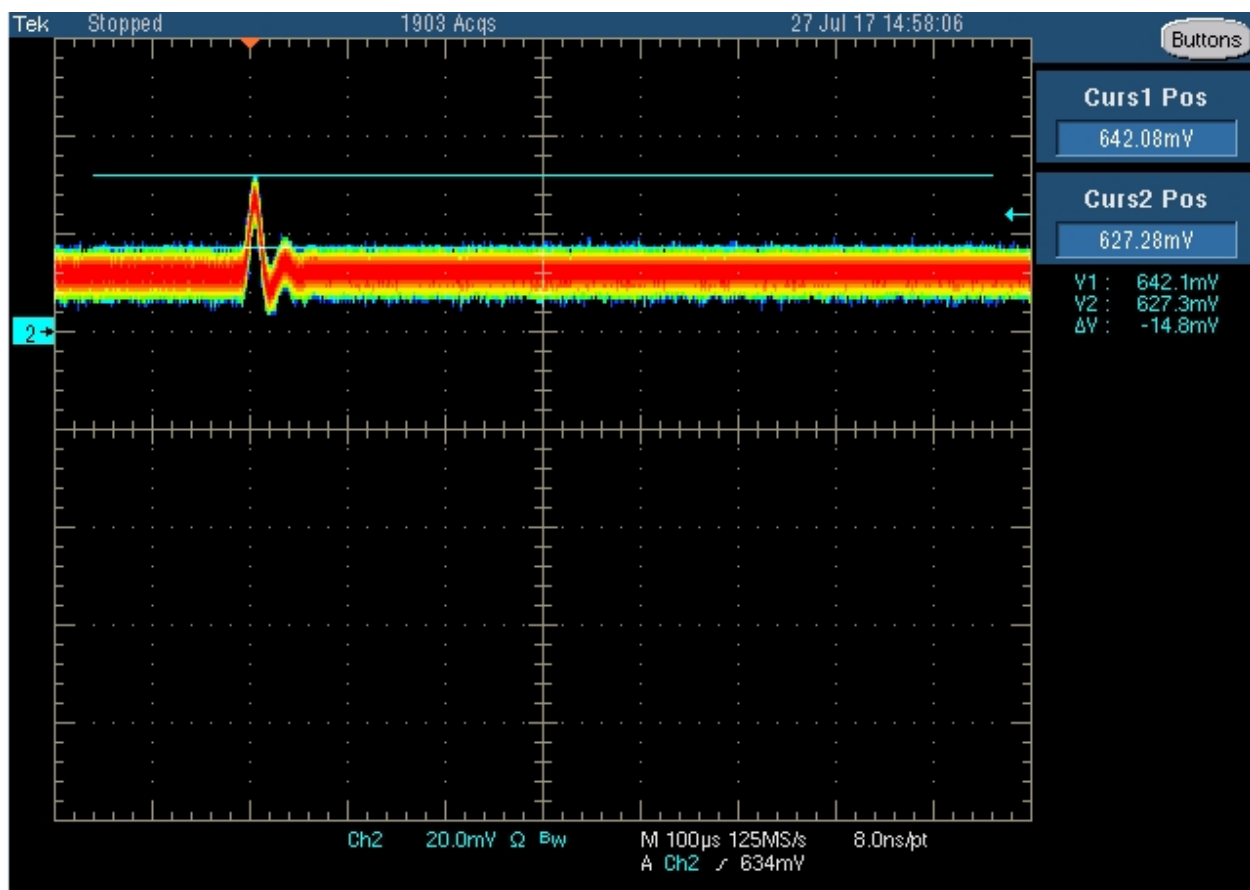
Figure 52 - PS_DDR4_VTT ac ripple release
