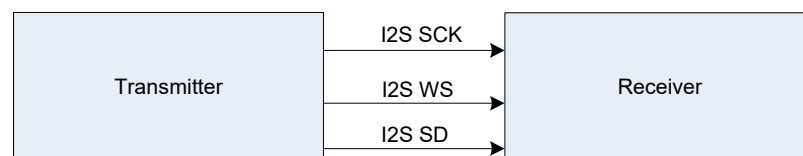
Figure 8-5. I2S Interface
