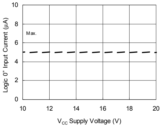
Figure 21B. Logic "0" Input Currentt vs. Supply Voltage
