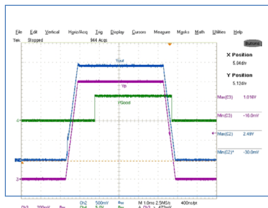
48: Voltage tracking using Vp pin Ch2-Vo,Ch3-Vp,Ch4-PGood
