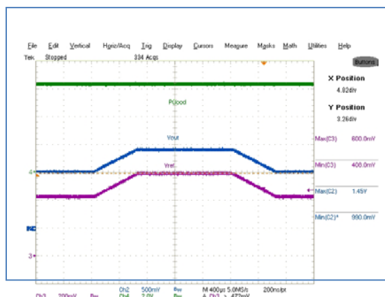
Figure 47: Voltage Margining using Vref pin Ch2-Vo,Ch3-Vref,Ch4-PGood
