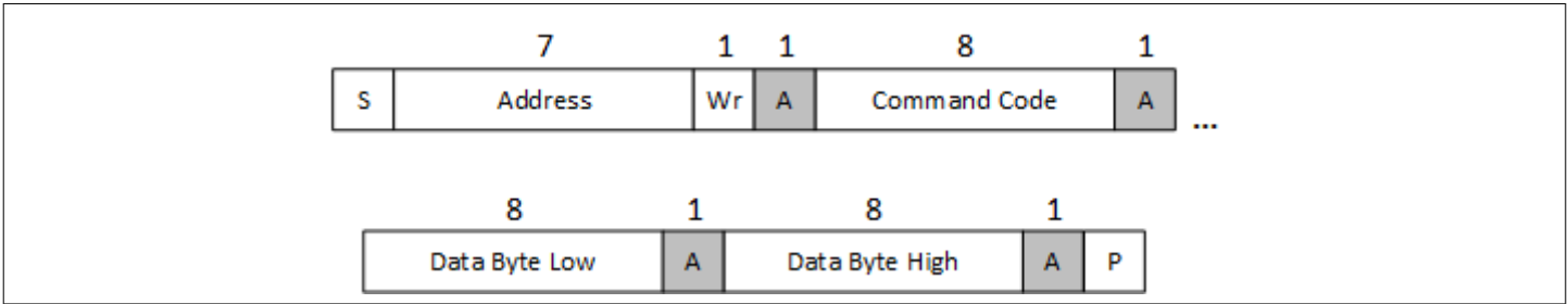
Figure 24 Write word protocol
