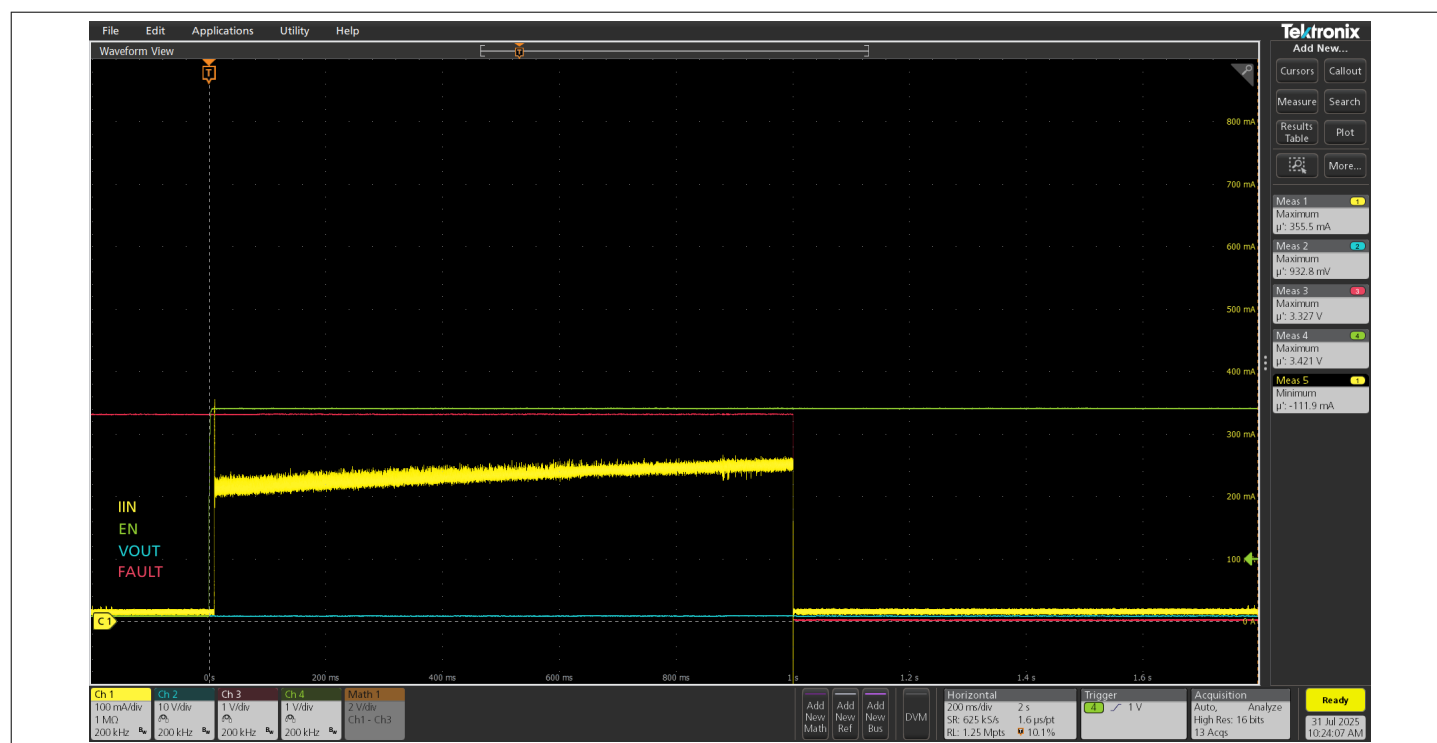
Figure 16 Start-up into short protection triggers watchdog (WD) fault after 1 s
