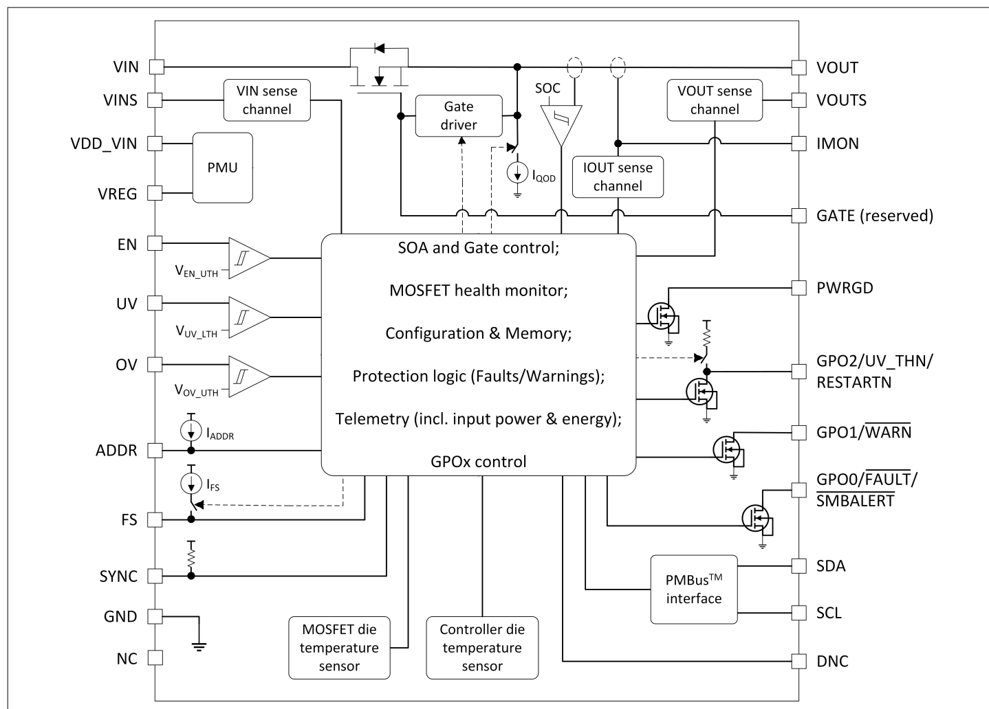
Figure 2 XDP730 block diagram
