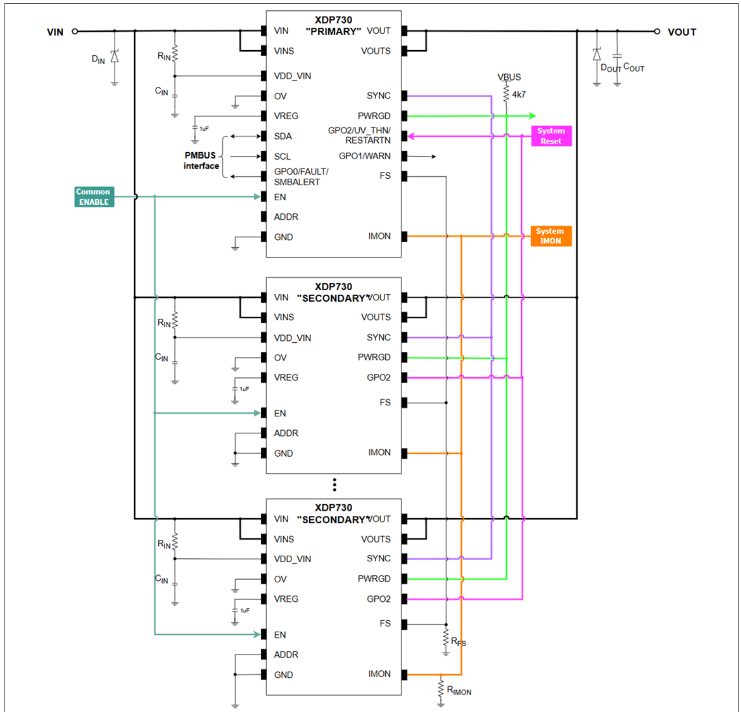
Figure 43 XDP730 typical application schematic (parallel operation)
