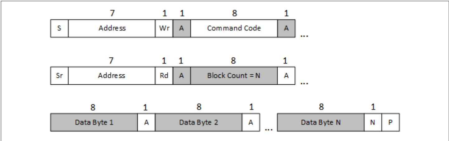
Figure 35 Block read
