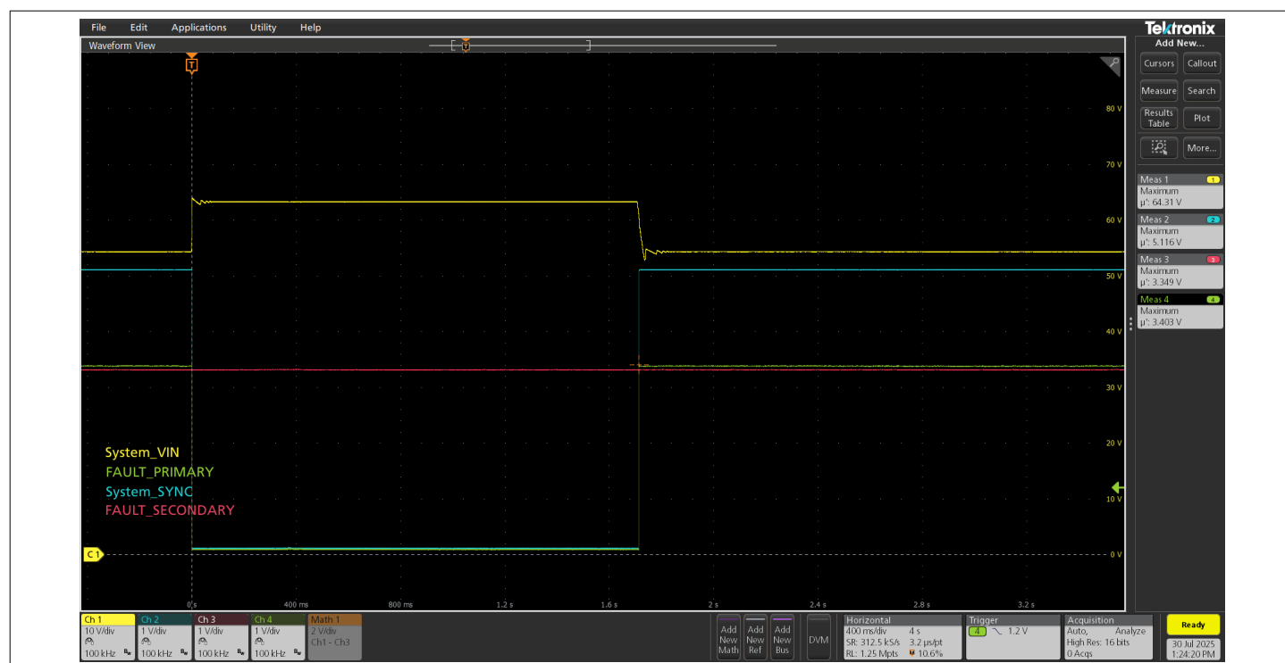
Figure 45 An input OV fault being triggered in PRIMARY device followed by a successful fault release
