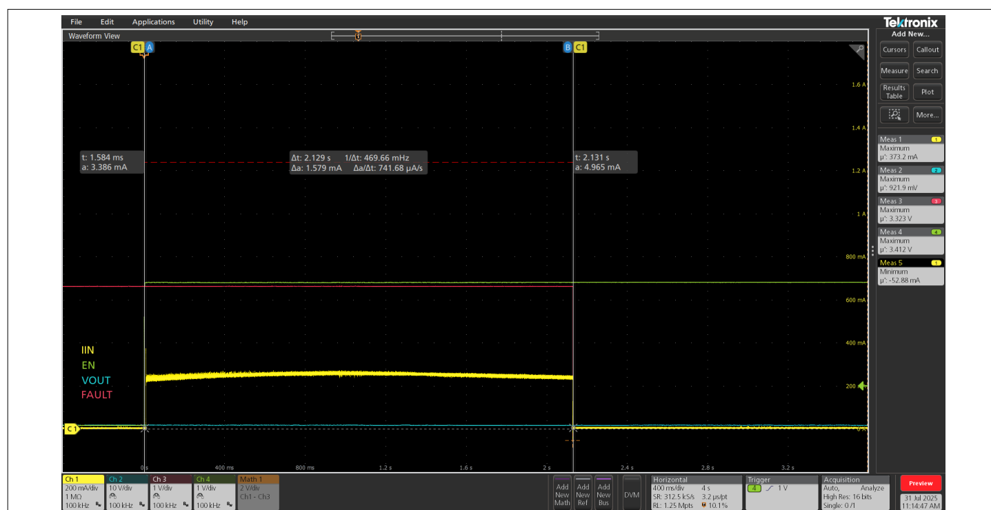
Figure 17 Start-up into short protection triggers thermal shutdown fault (TSD) after ~2.12 s; WD fault is either disabled or programmed to a higher value i.e. > 2 s
