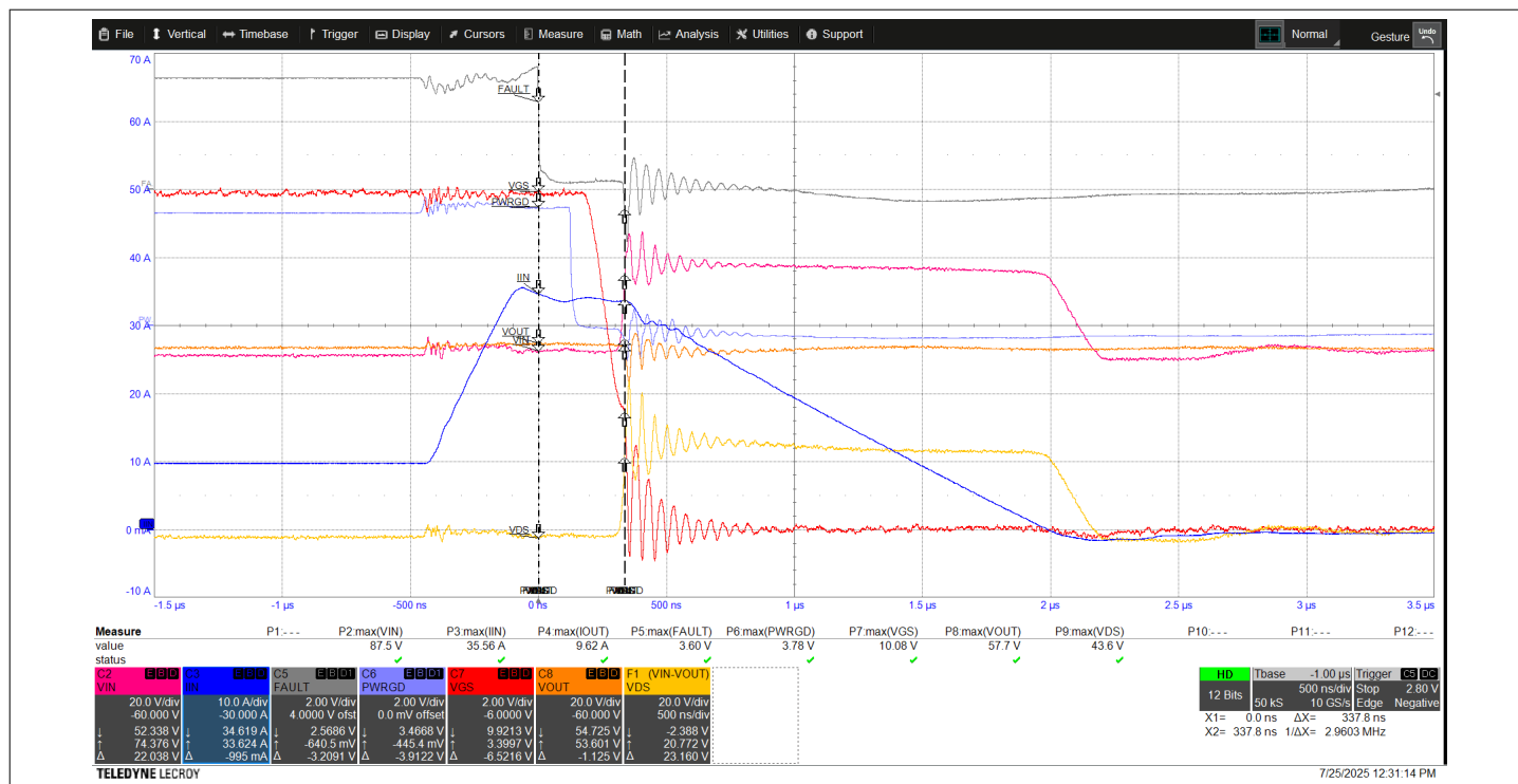
Figure 15 Severe overcurrent fault (SOC_LIMIT_P = ~30 A) being triggered followed by a fast MOSFET turn-off within ~400 ns
