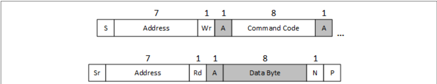
Figure 27 Read byte protocol
