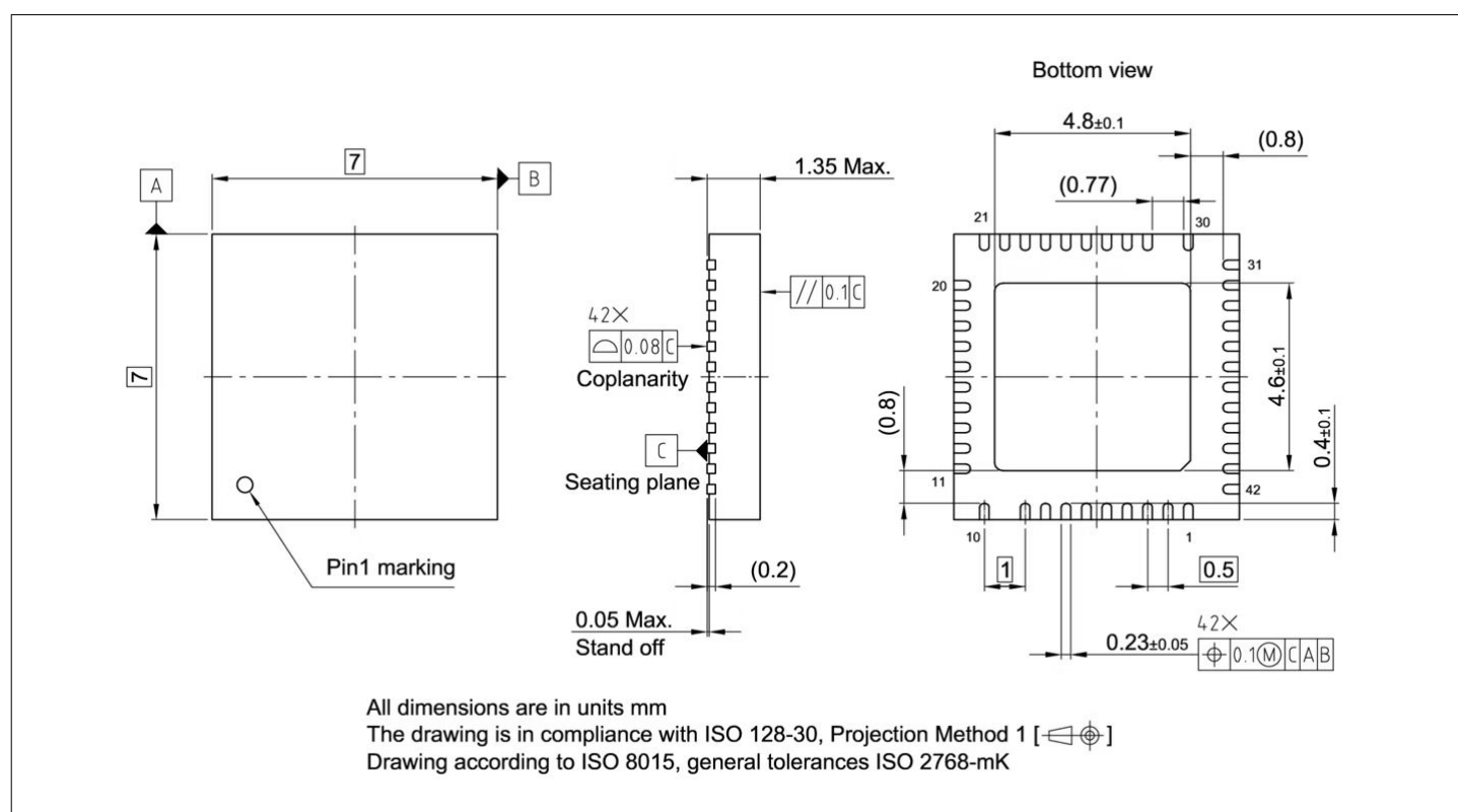
Figure 47 XDP730-001 package dimensions
