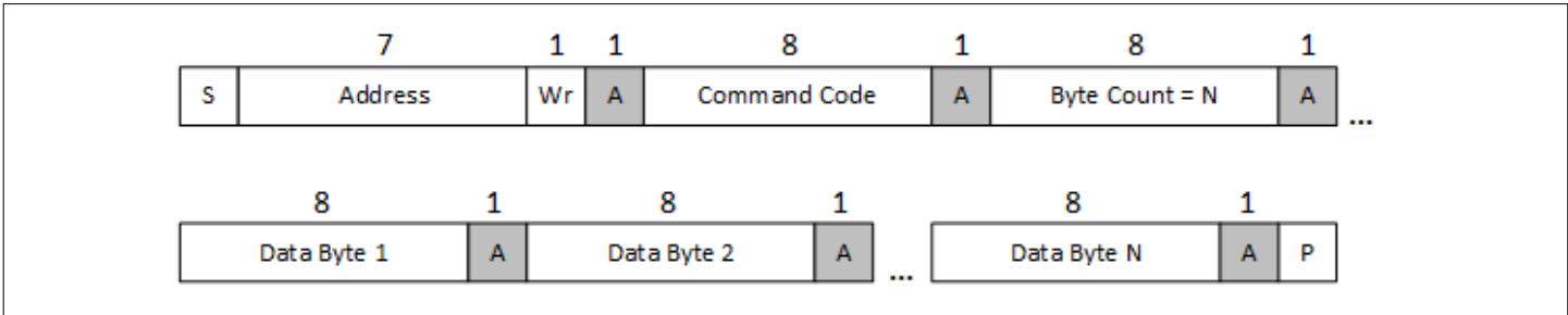
Figure 33 Block write
