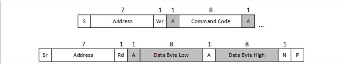
Figure 29 Read word protocol
