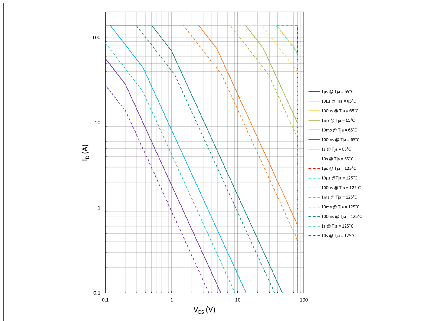
Figure 11 MOSFET's SOA chart during ON state i.e. steady-state operation
