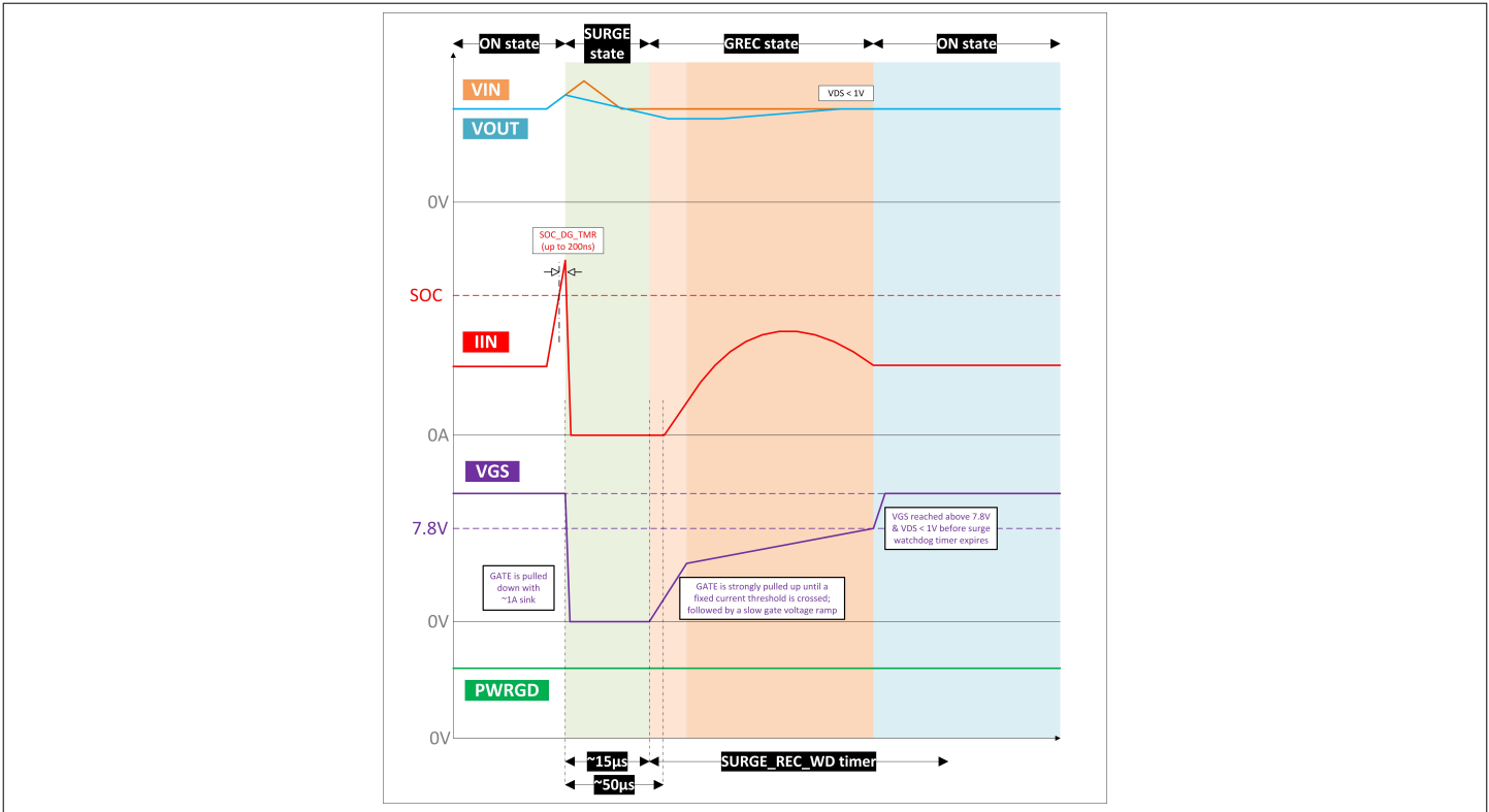
Figure 18 Surge immunity illustration
