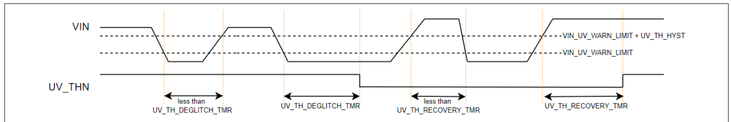
Figure 20 UV throttle function
