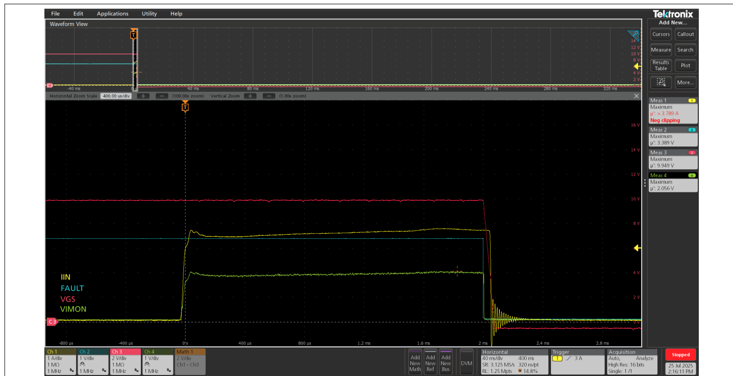
Figure 14 Overcurrent fault ( V_{IMON} > 1.0025 \text{ V} ) being triggered after 2 ms deglitch time; R_{IMON} = 27.5 \text{ k}\Omega
