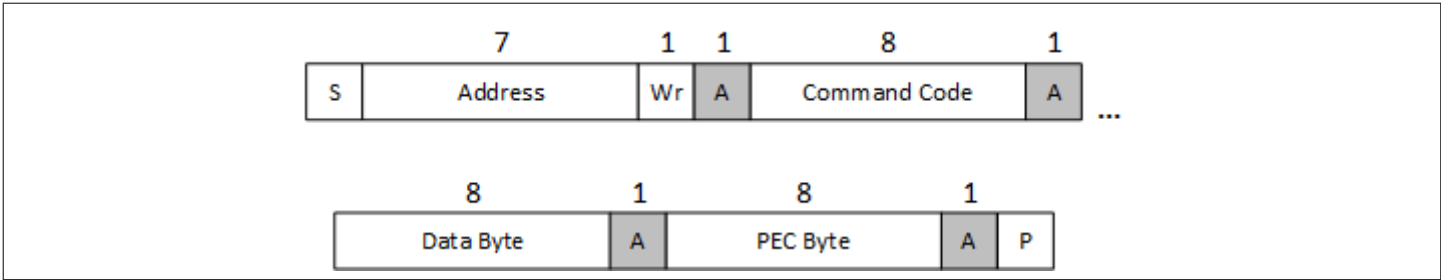
Figure 25 Write byte protocol with PEC
