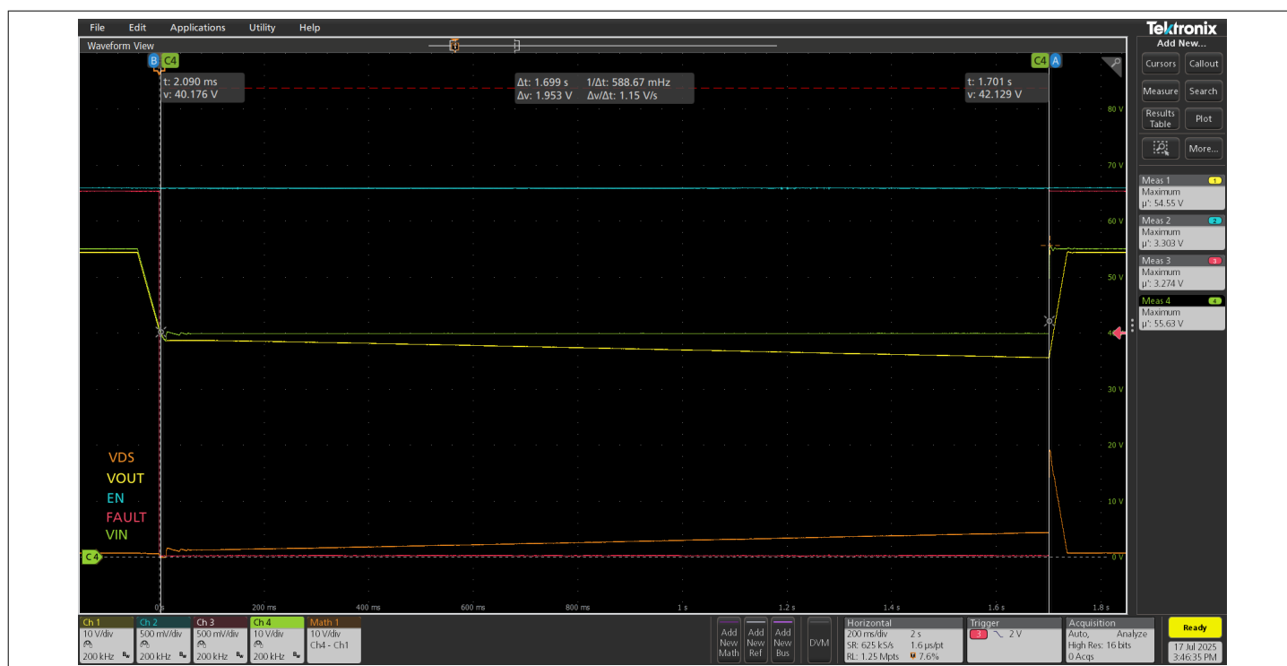
Figure 12 Input UV fault (VIN_UV_FAULT_LIMIT = 40 V) being triggered followed by a successful fault release
