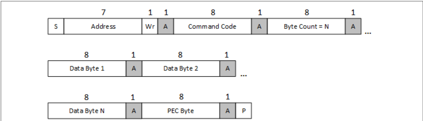
Figure 34 Block write with PEC
