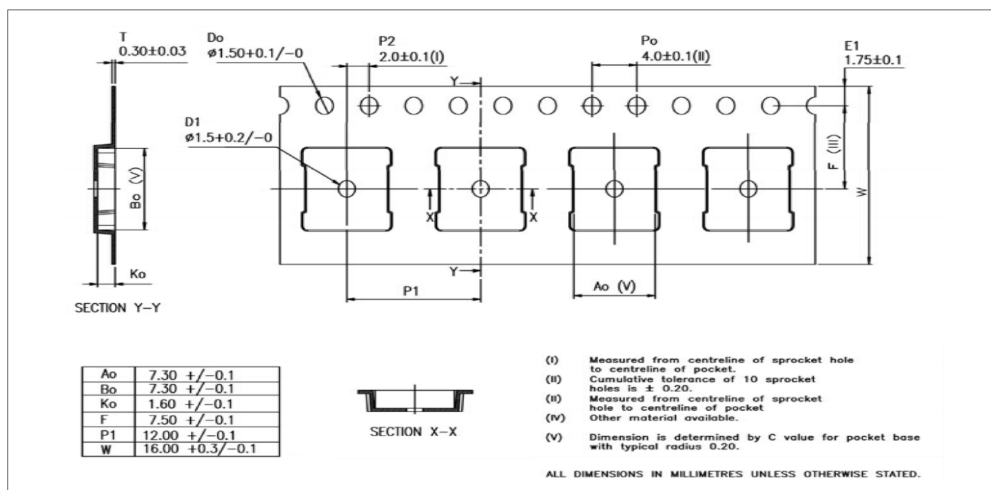
Figure 49 PG-LIQFN-42-1 package information
