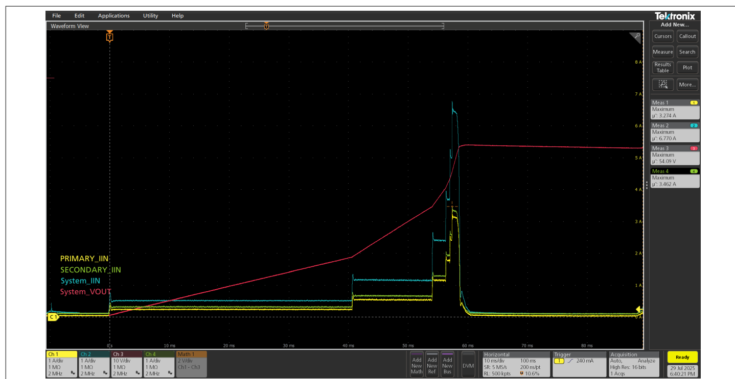
Figure 44 Parallel operation: Default turn-on
