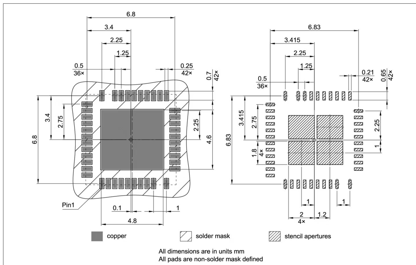
Figure 48 XDP730-001 recommended footprint
