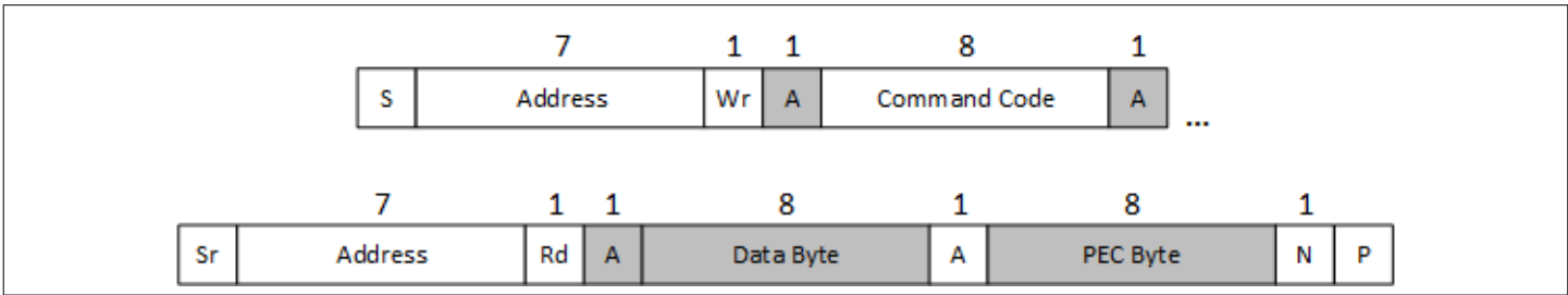
Figure 28 Read byte protocol with PEC
