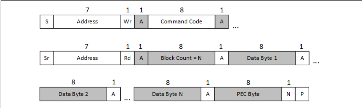
Figure 36 Block read with PEC
