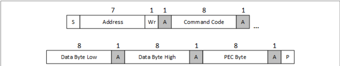
Figure 26 Write word protocol with PEC
