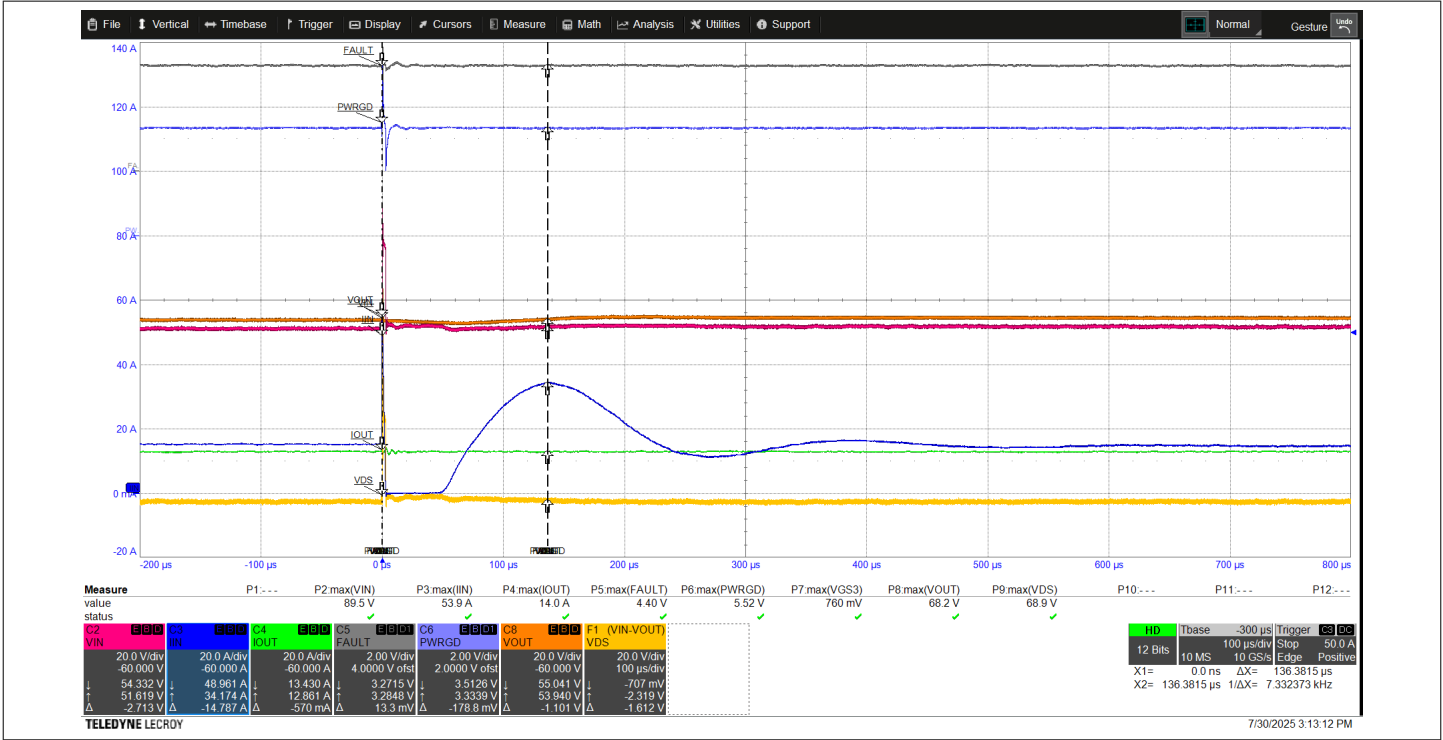
Figure 19 Input surge immunity protection triggers a fast MOSFET turn-off (SOC_LIMIT_P = 50 A) followed by a successful recovery; COUT = 1 mF
