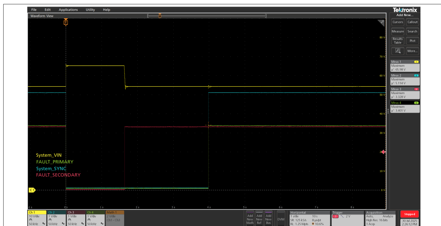
Figure 46 An OV fault being triggered in SECONDARY device resulting in a SYNC fault in PRIMARY device; Auto-retry enabled in PRIMARY with 4 s cool down time
