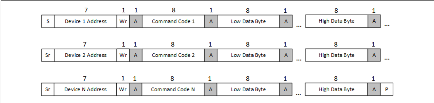
Figure 37 Group command protocol
