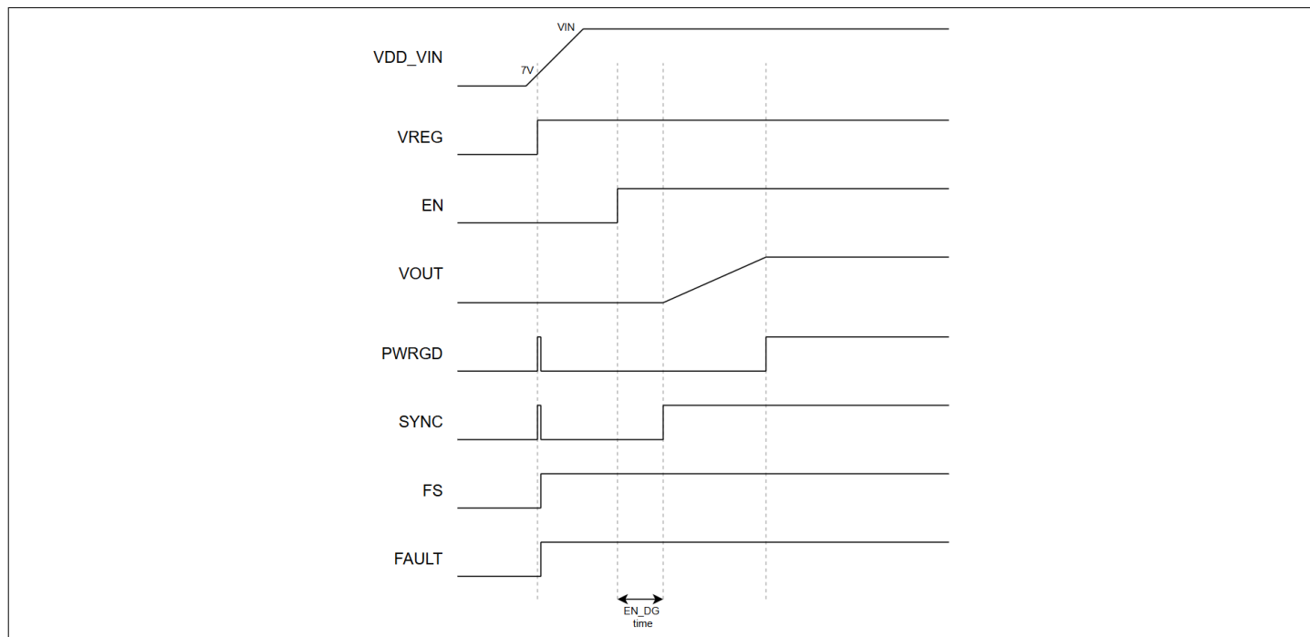
Figure 4 XDP730 power-up sequence (PWRGD and FAULT tied to VREG)
