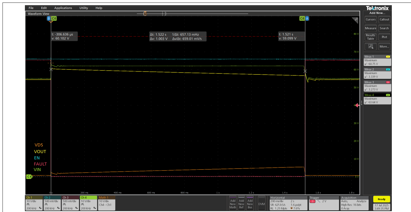
Figure 13 Input OV fault (VIN_OV_FAULT_LIMIT = 60 V) being triggered followed by a successful fault release
