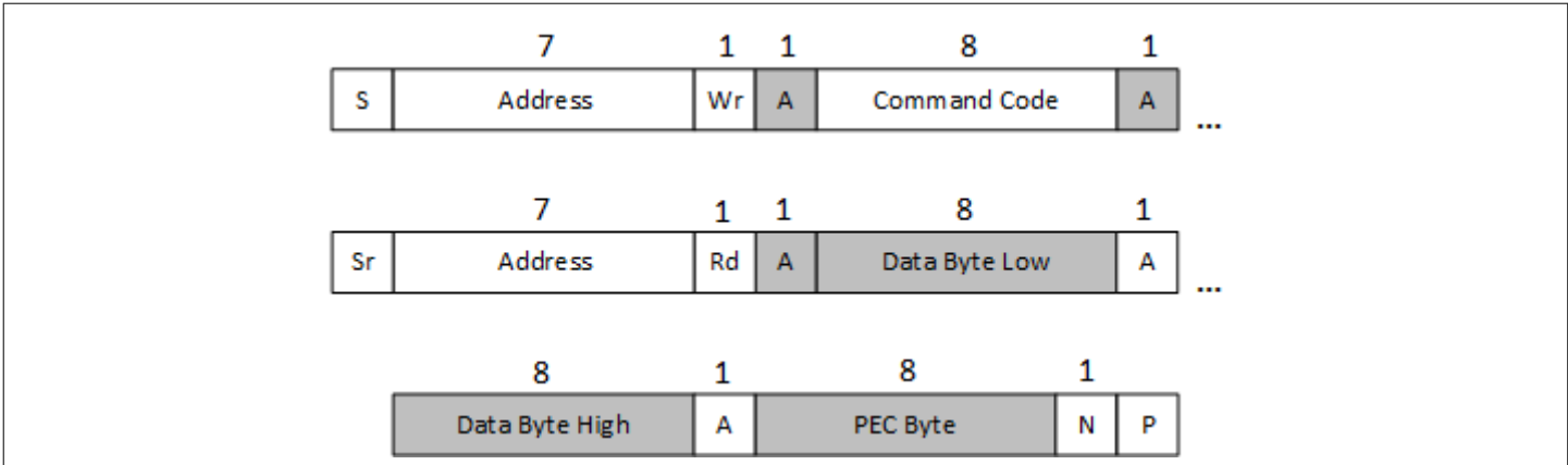
Figure 30 Read word protocol with PEC
