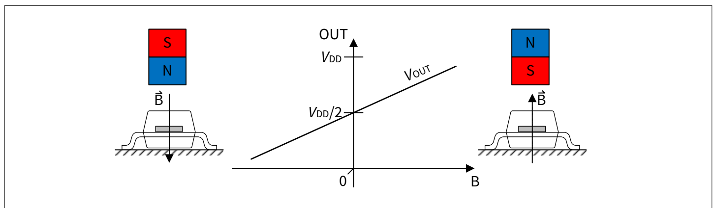
Figure 3 Magnetic field direction with corresponding sensor out signal
