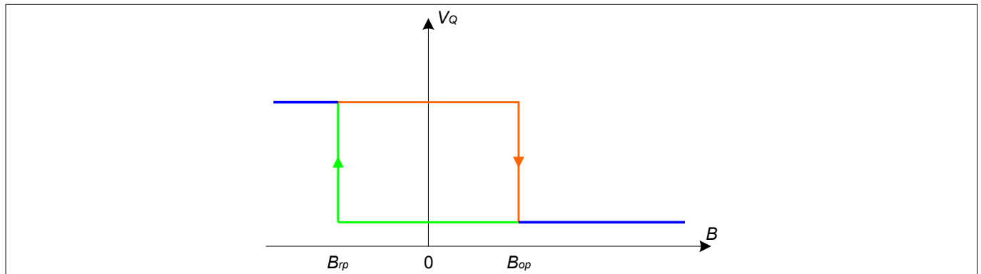
Figure 4 Output signal
