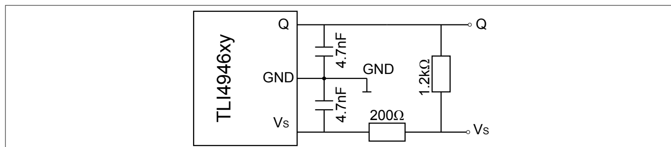
Figure 5 Application circuit
