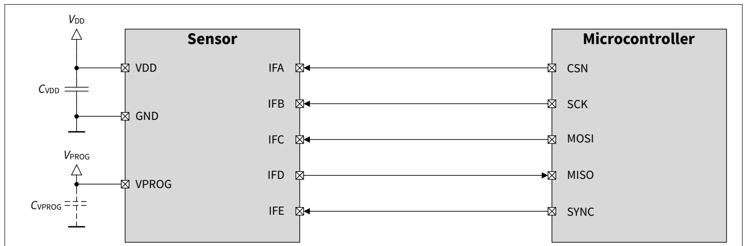
Figure 21 Application diagram - SPI
