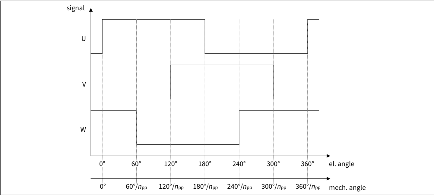
Figure 19 UVW interface switching pattern
