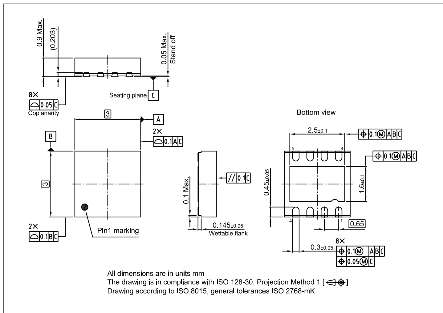
Figure 28 Package outline PG-VSON-8
