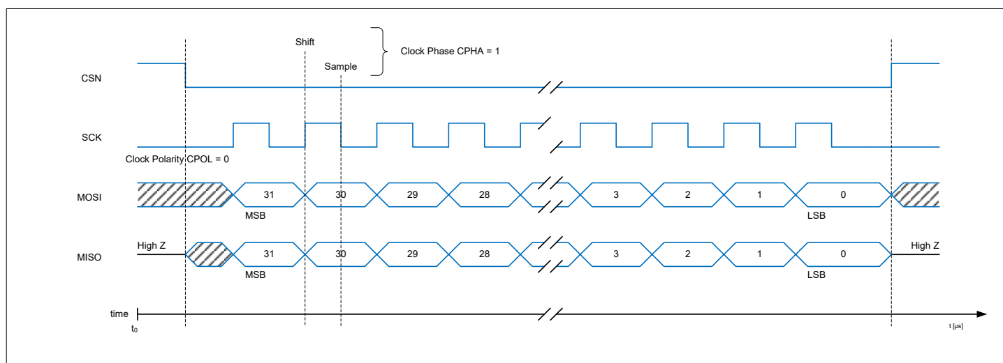
Figure 5 SPI mode 1
