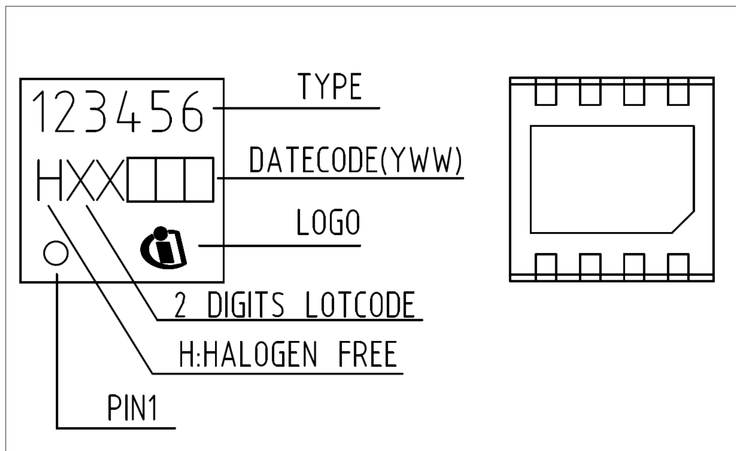
Figure 30 PG-VSON-8 package marking (left top side, right bottom side)
