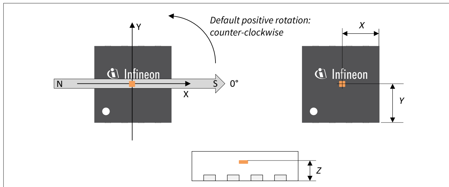
Figure 27 Sensitive area location (orange), Cartesian measurement reference system (black) and magnetic field vector indicating the 0° angle (grey)
