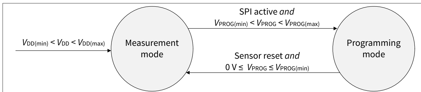
Figure 20 Sensor states for normal operation (measurement mode) and for programming the NVM
