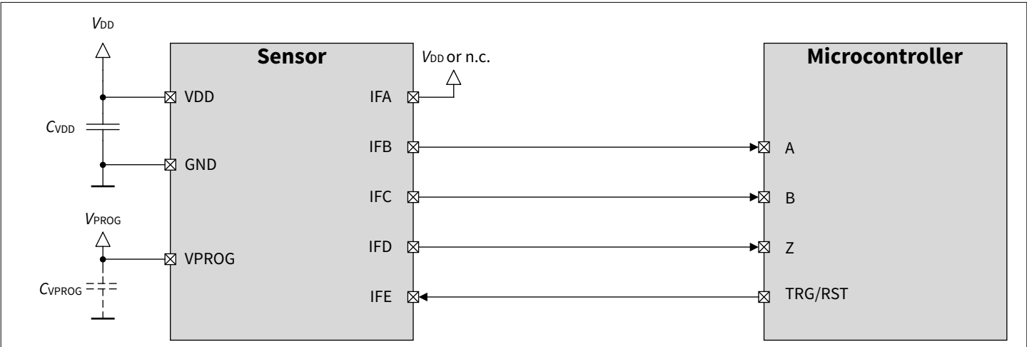
Figure 23 Application diagram - ABZ (encoder mode)
