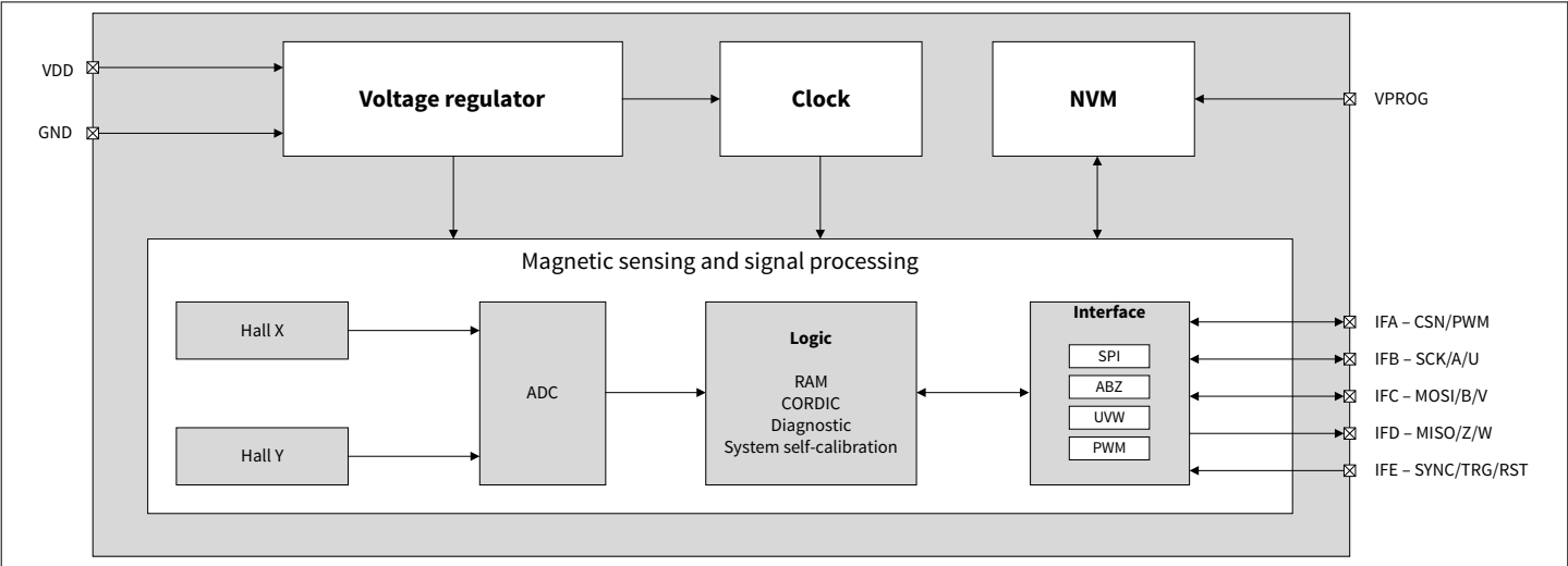
Figure 1 Block diagram
