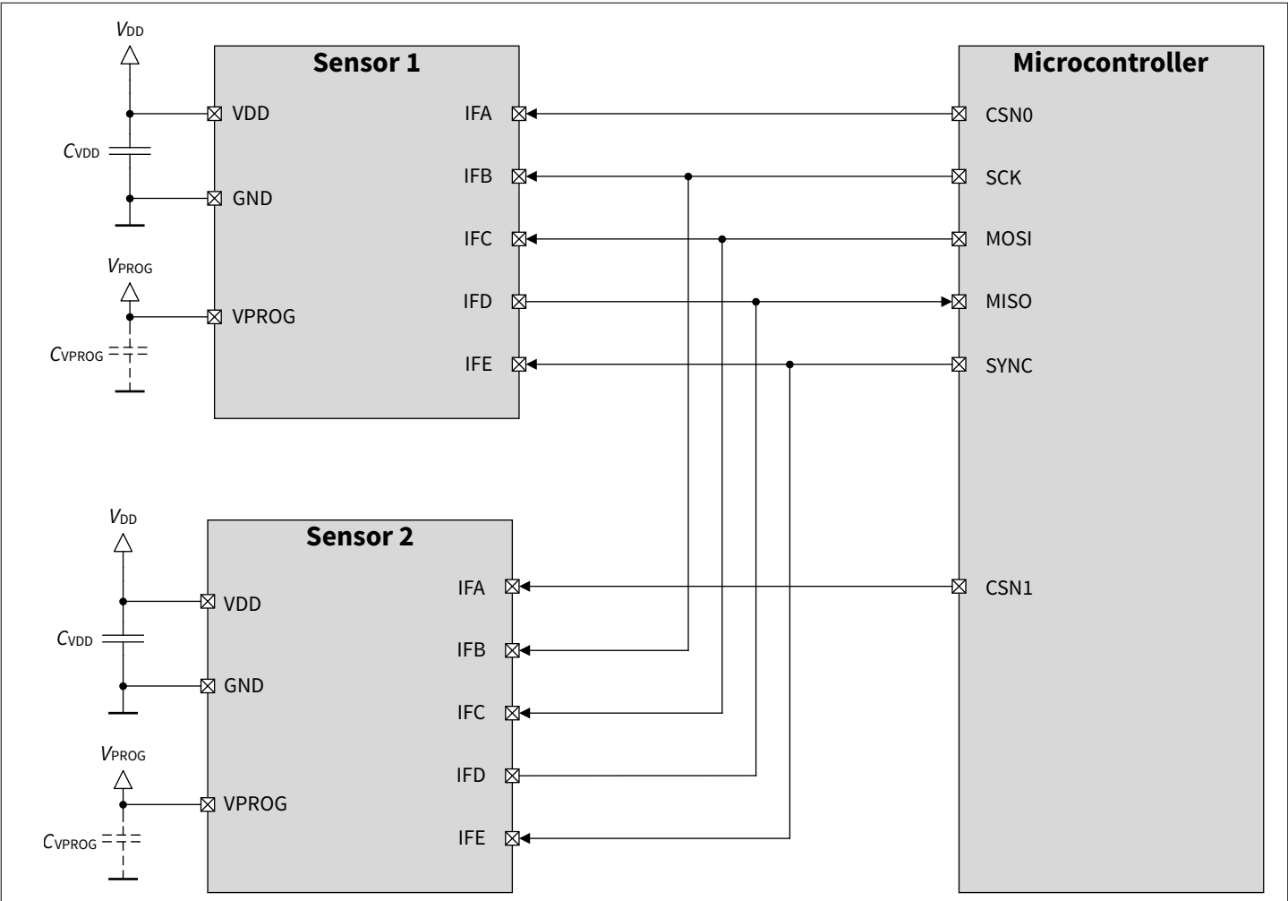
Figure 22 Application diagram - SPI multi slave
