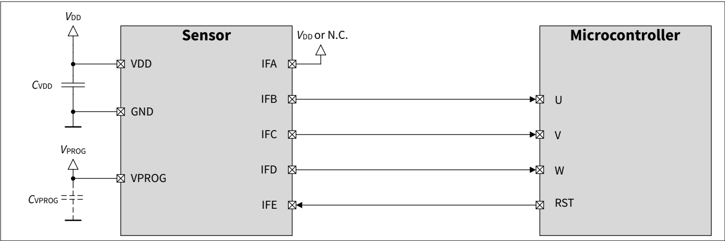
Figure 24 Application diagram - UVW (hall switch mode)
