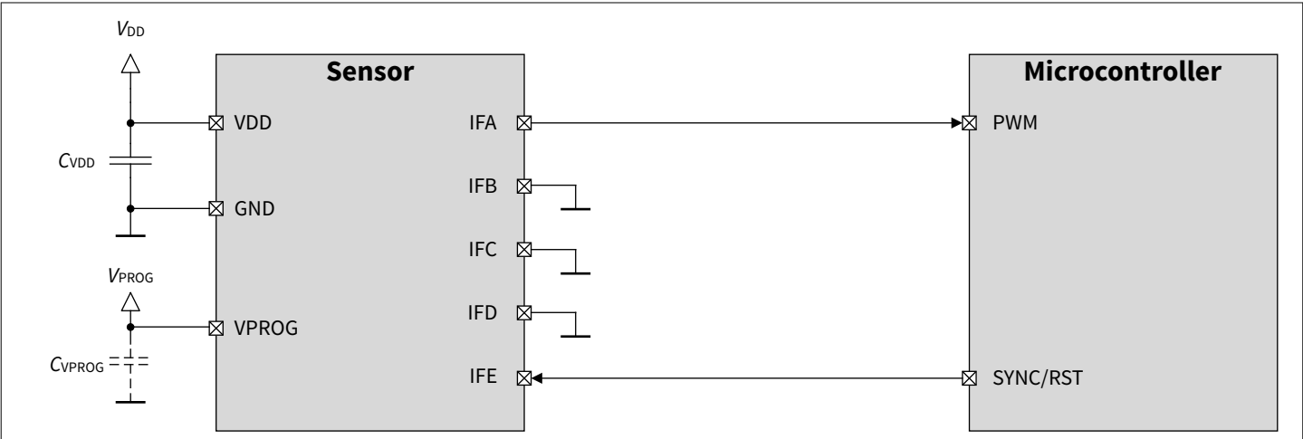
Figure 25 Application diagram - PWM
