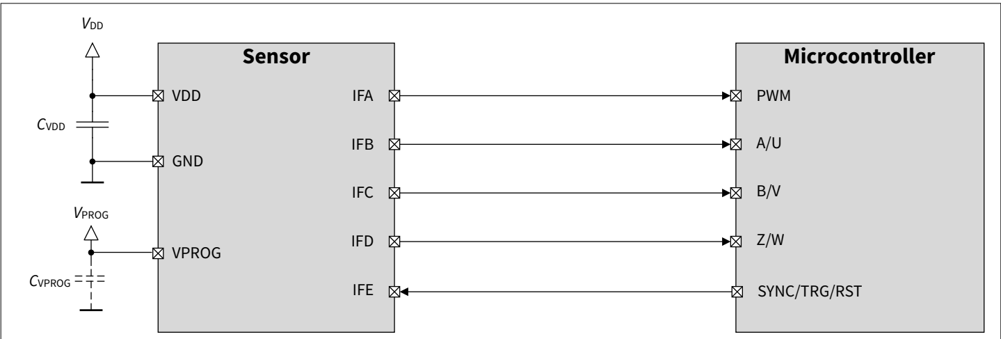
Figure 26 Application diagram - ABZ or UVW in parallel with PWM
