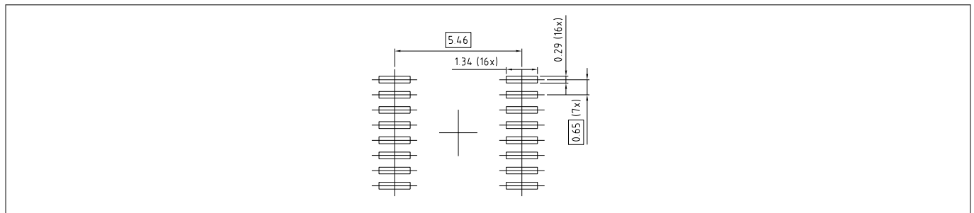
Figure 25 Footprint
