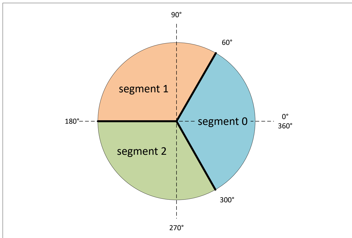
Figure 17 Programmable output 120° characteristic curve
