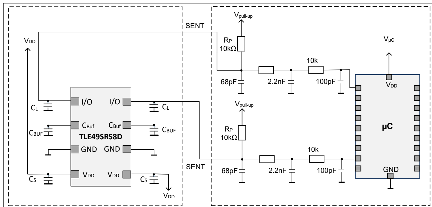
Figure 18 Application circuit for SENT interface
