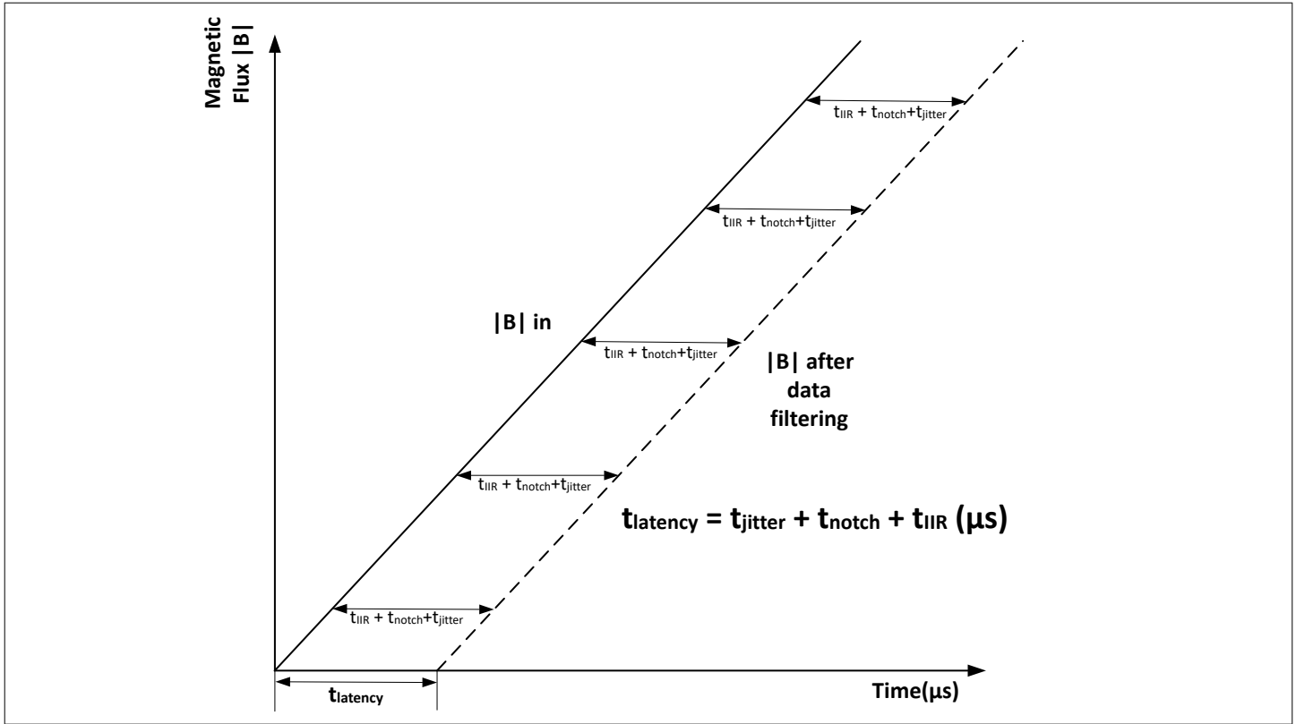
Figure 6 Latency time description
