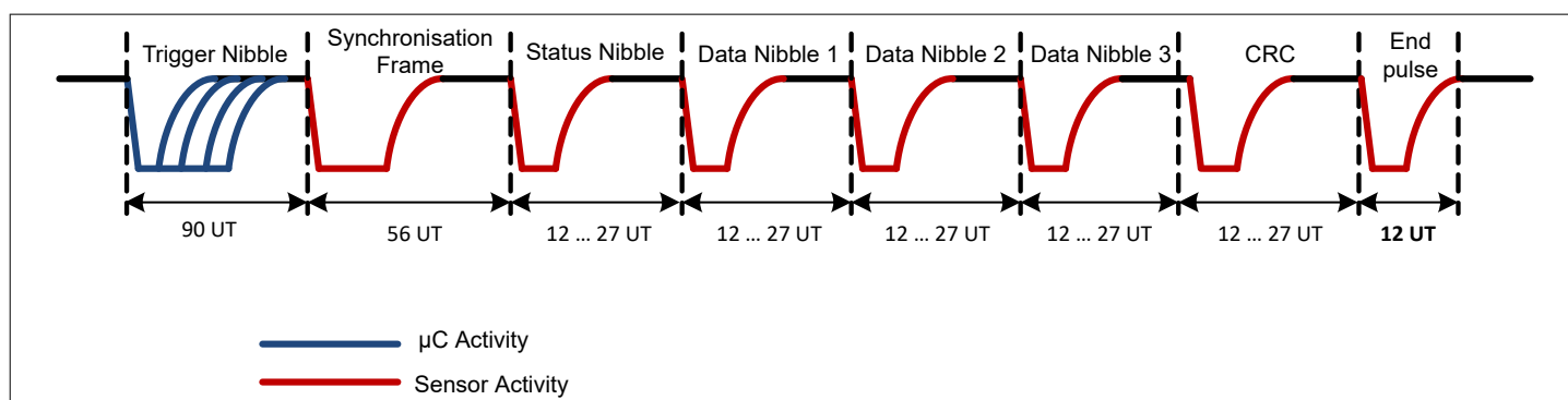
Figure 11 SPC frame with 3 data nibbles
