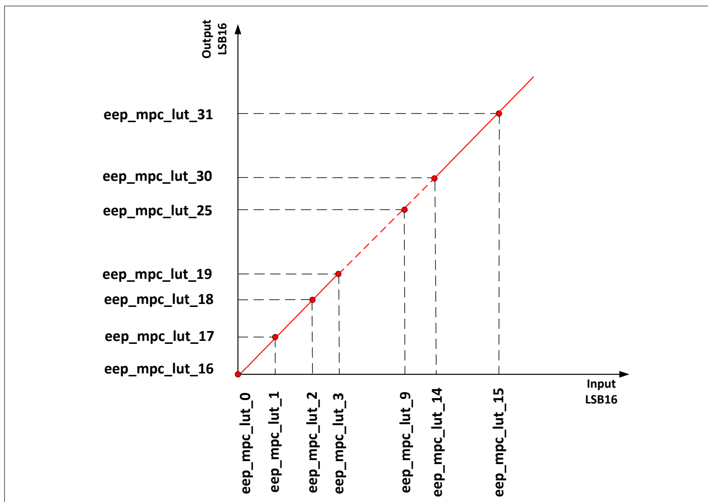
Figure 15 16 freely programmable points
