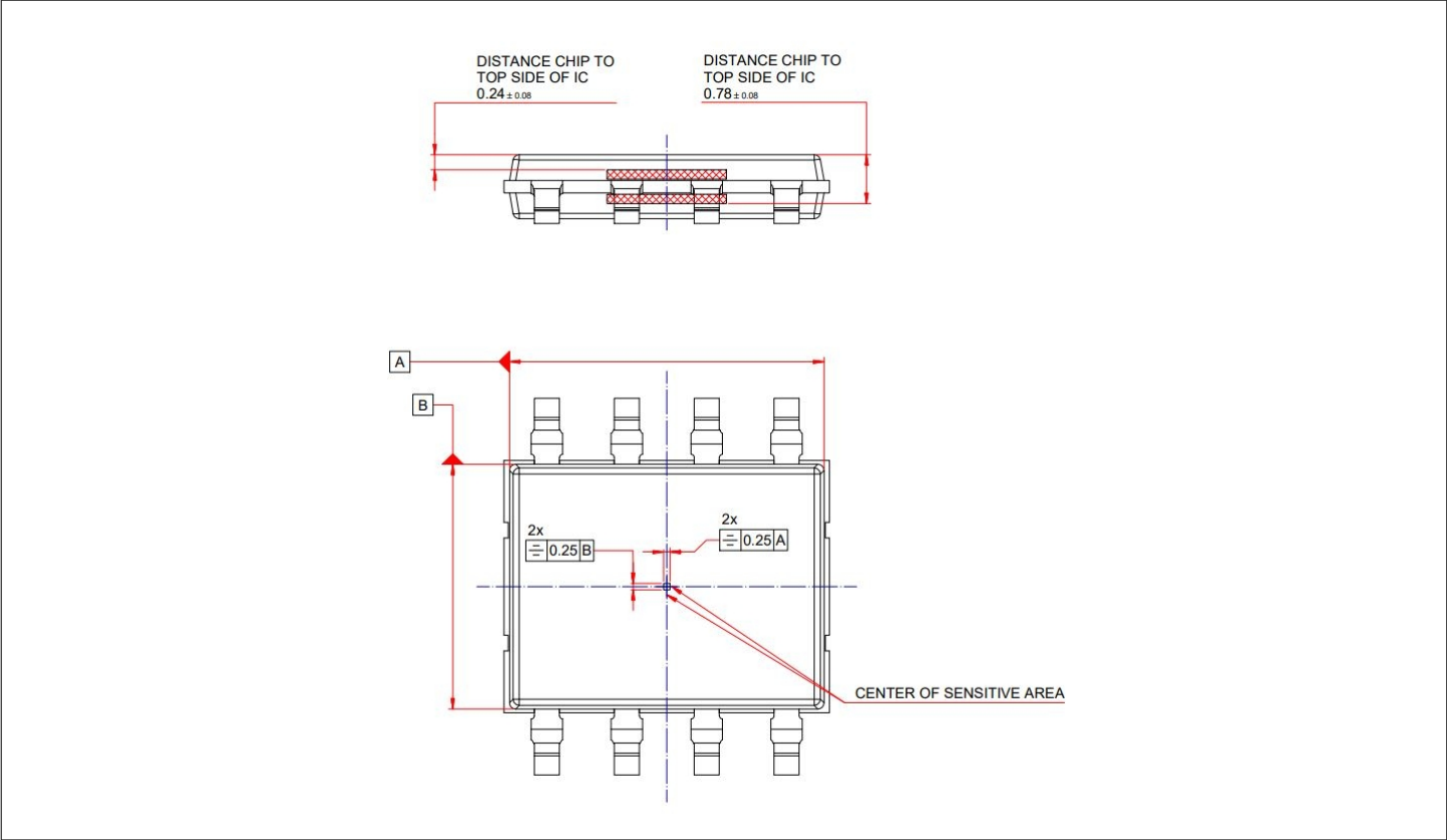
Figure 23 PG-TDSO-8-20 center of sensitive area
