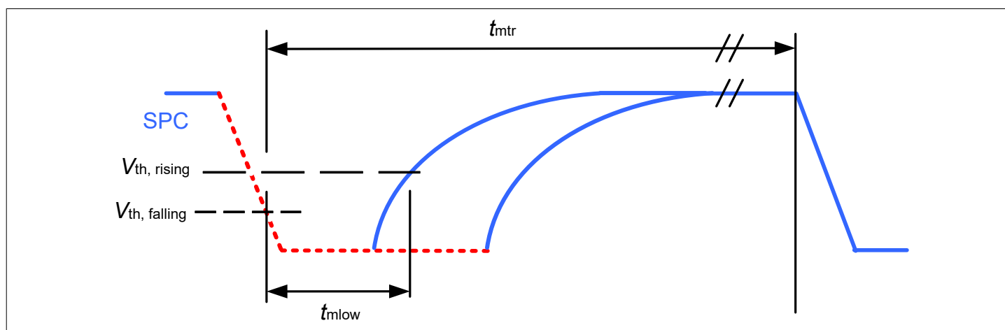
Figure 13 SPC master pulse timing
