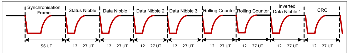
Figure 8 SENT single secure frame
