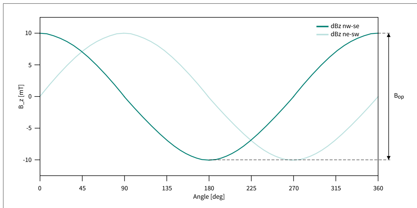
Figure 3 Operating magnetic field example
