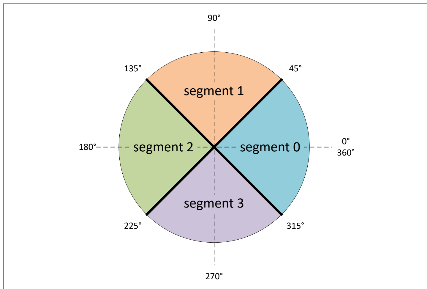
Figure 16 Programmable output 90° characteristic curve
