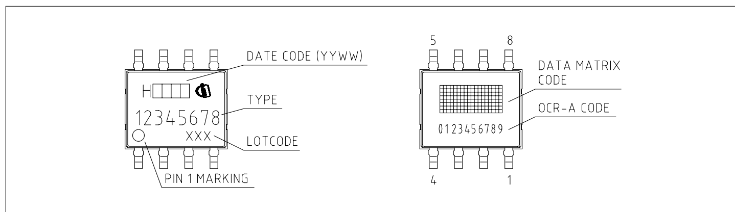
Figure 22 PG-TDSO-8 package marking
