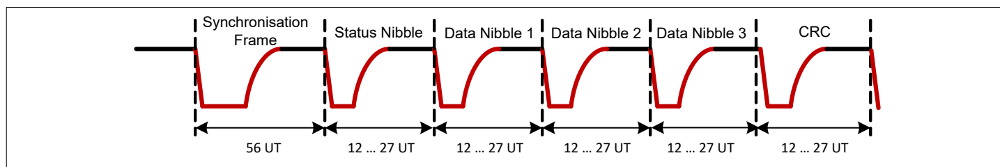
Figure 7 SENT standard frame
