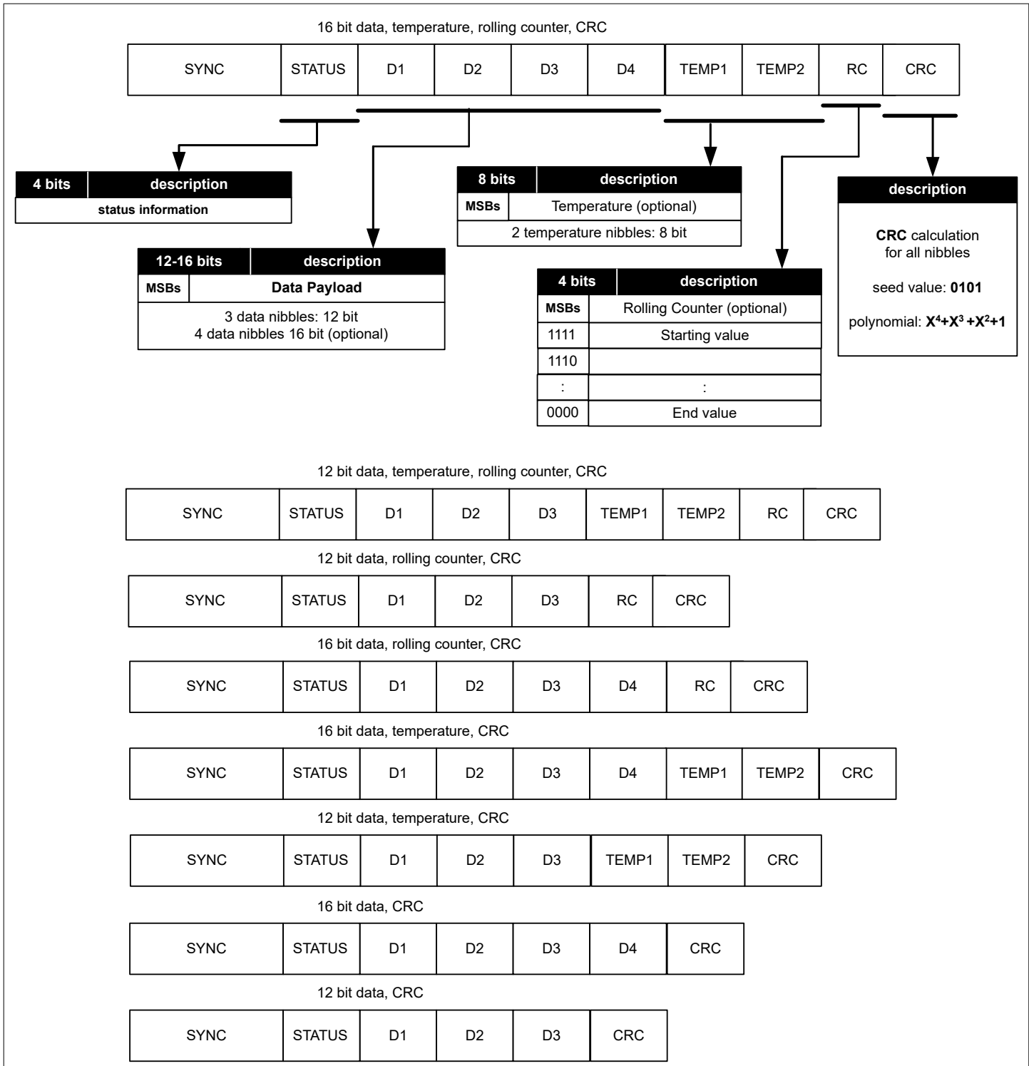
Figure 10 SENT frame options
