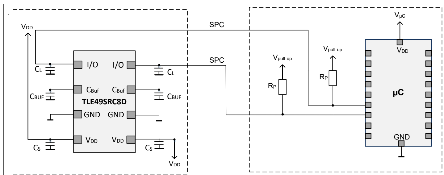
Figure 19 Application circuit for SPC interface
