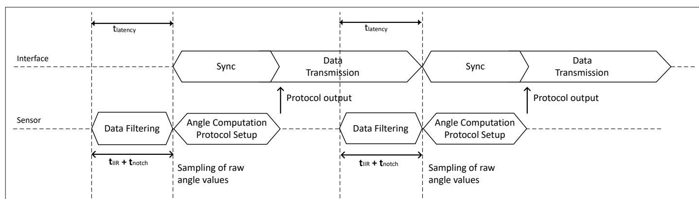
Figure 4 SENT interface timing overview
