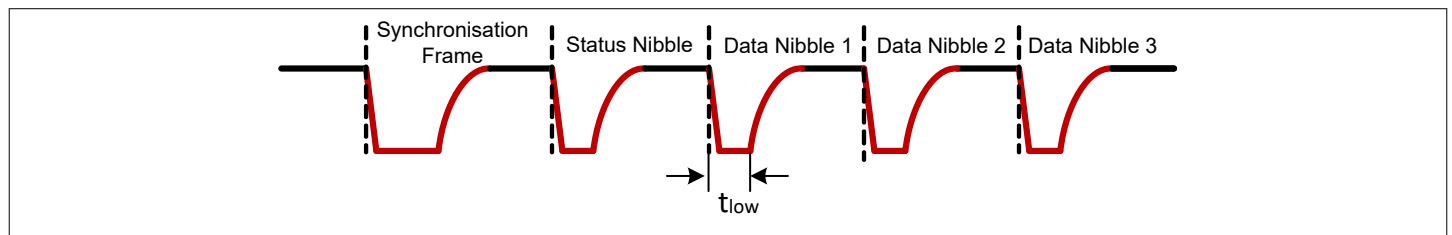
Figure 9 SENT nibble low time
