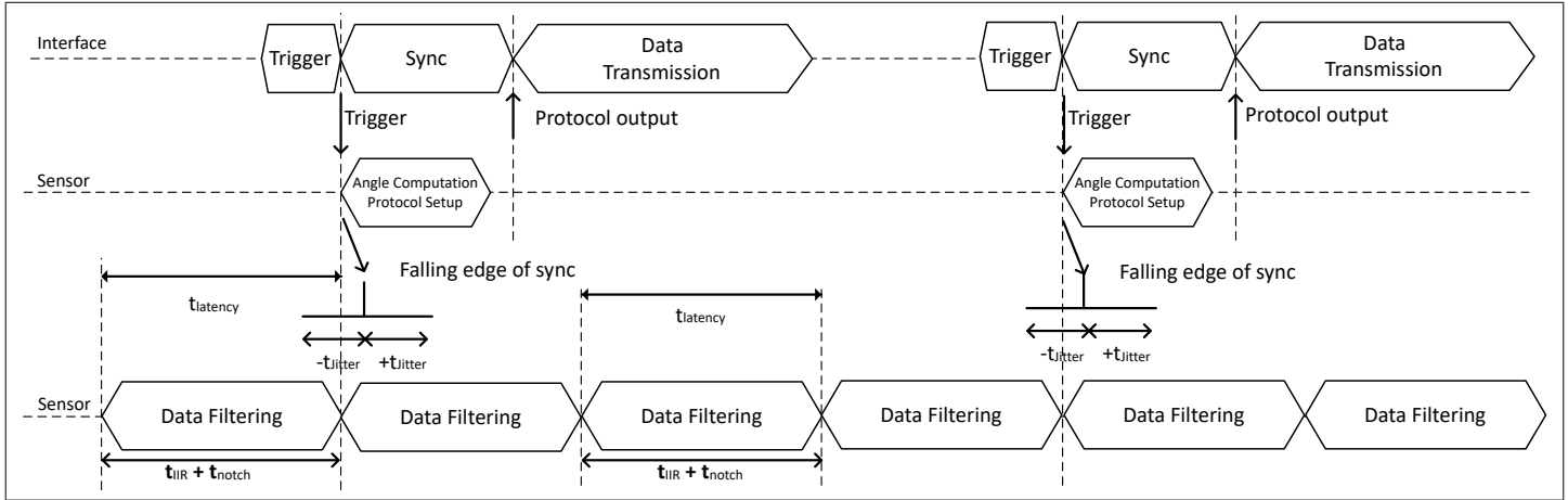
Figure 5 SPC interface timing
