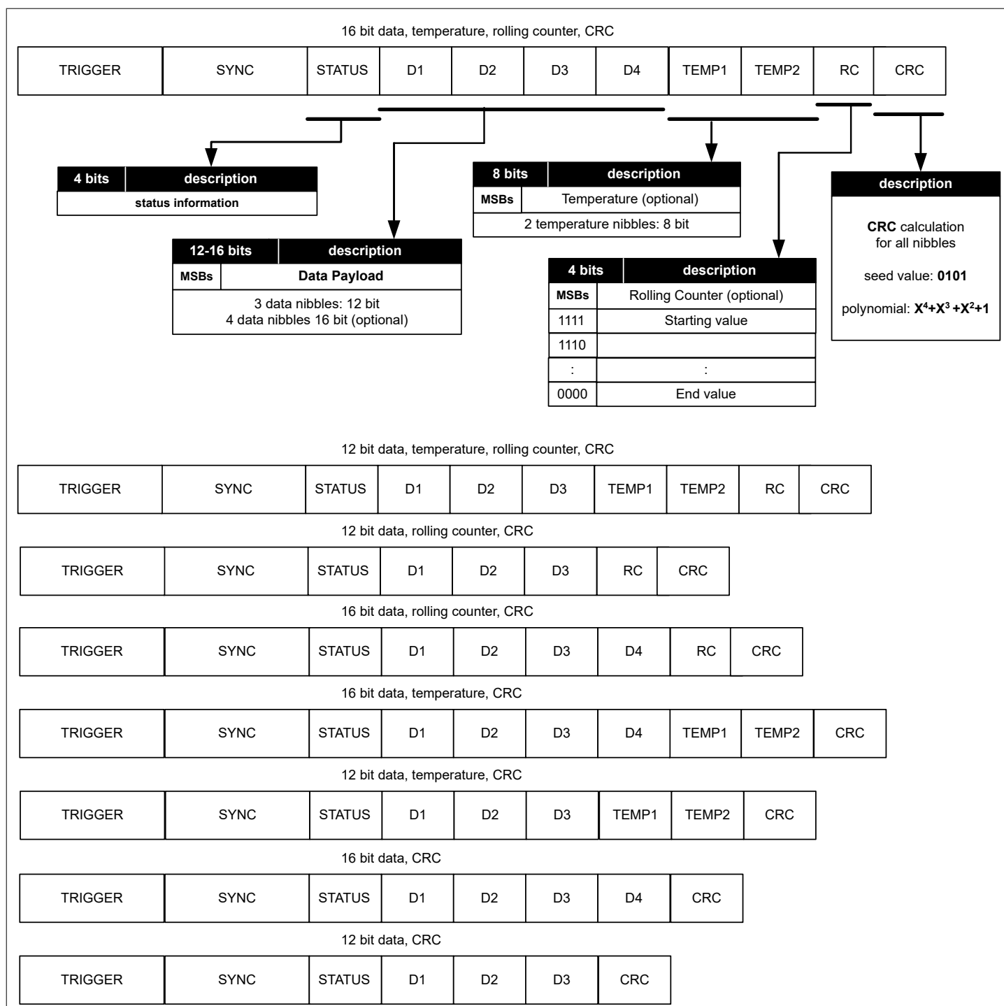
Figure 12 SPC frame modes
