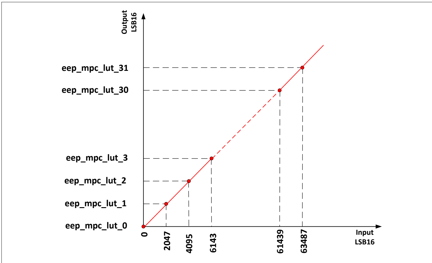
Figure 14 32 equidistant calibration points
