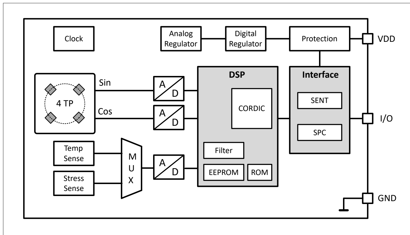
Figure 1 Functional block diagram of TLE49SR
