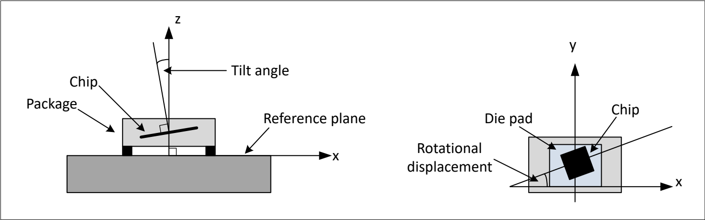
Figure 20 Tolerance of the die in the package
