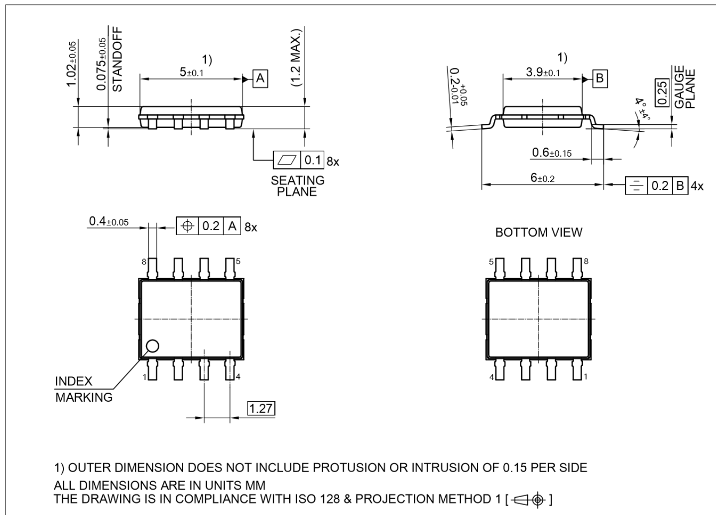
Figure 21 PG-TDSO-8-20 package drawing
