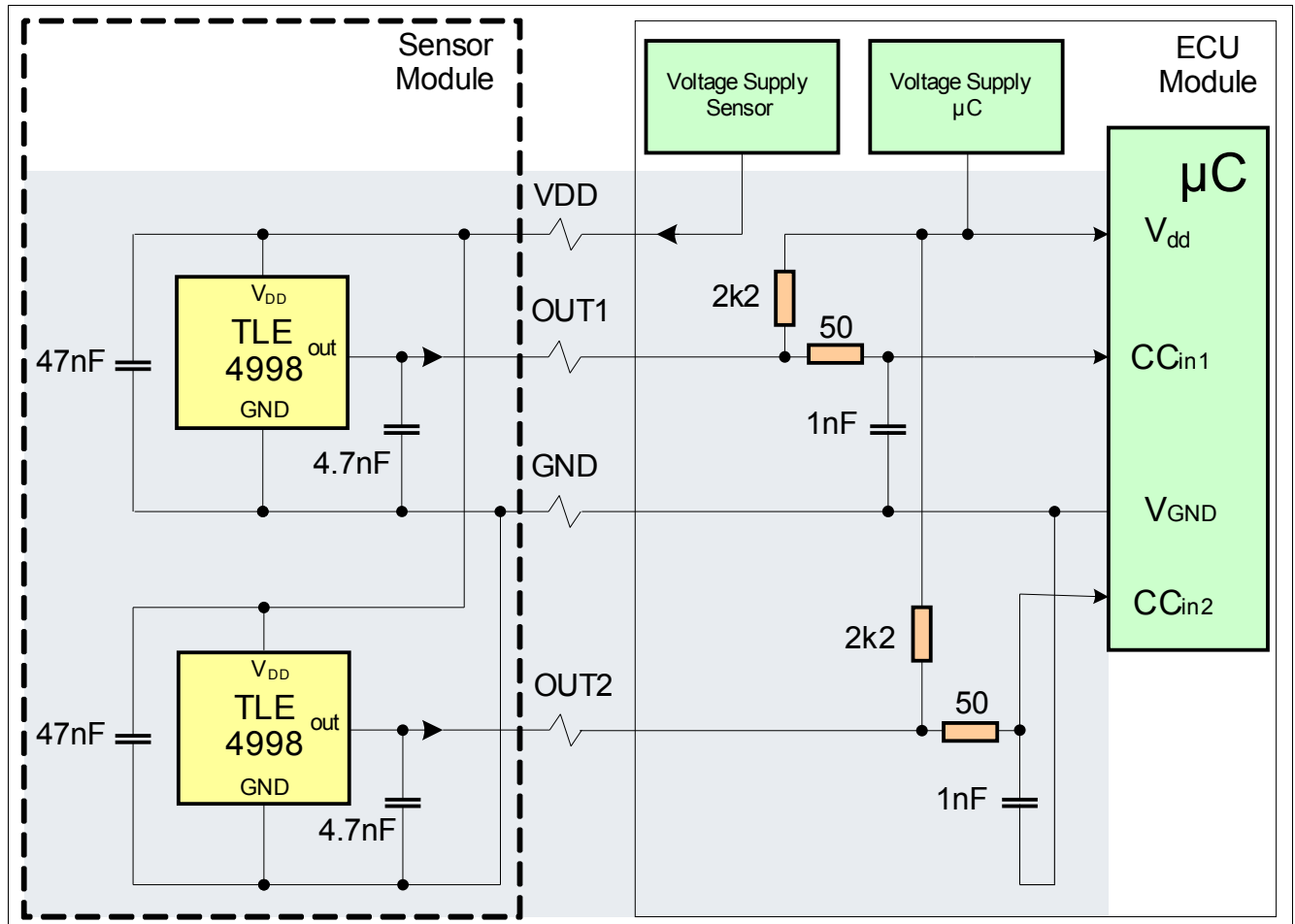
Figure 6-1 Application Circuit
