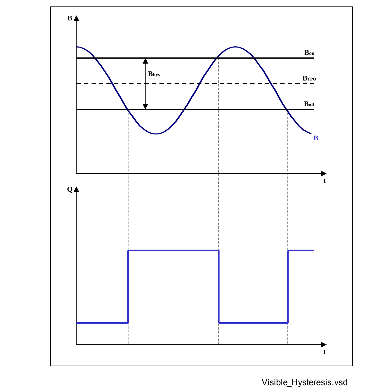
Figure 4 Visible Hysteresis
