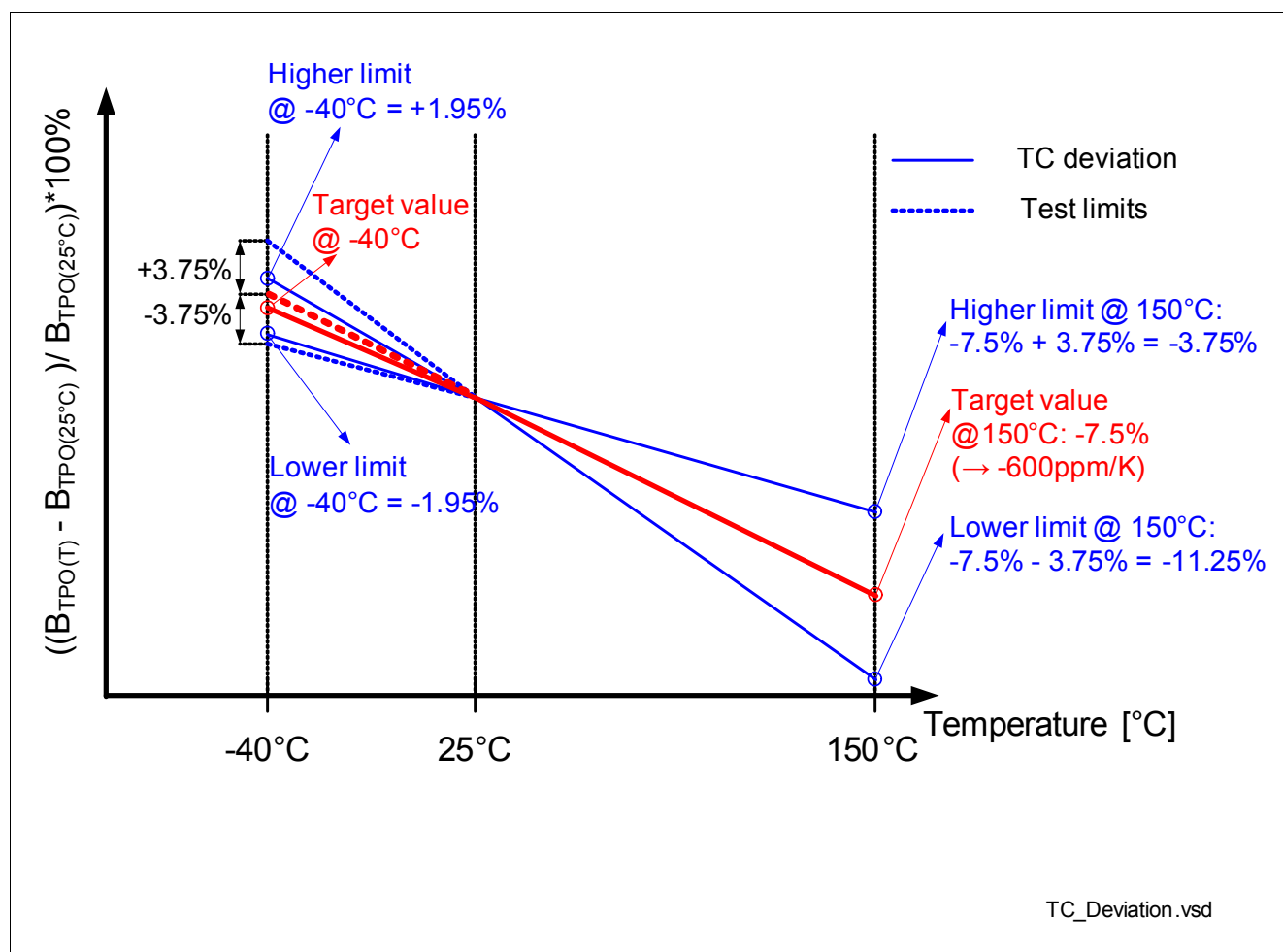
Figure 10 Temperature Coefficient of TPO Switching Point
