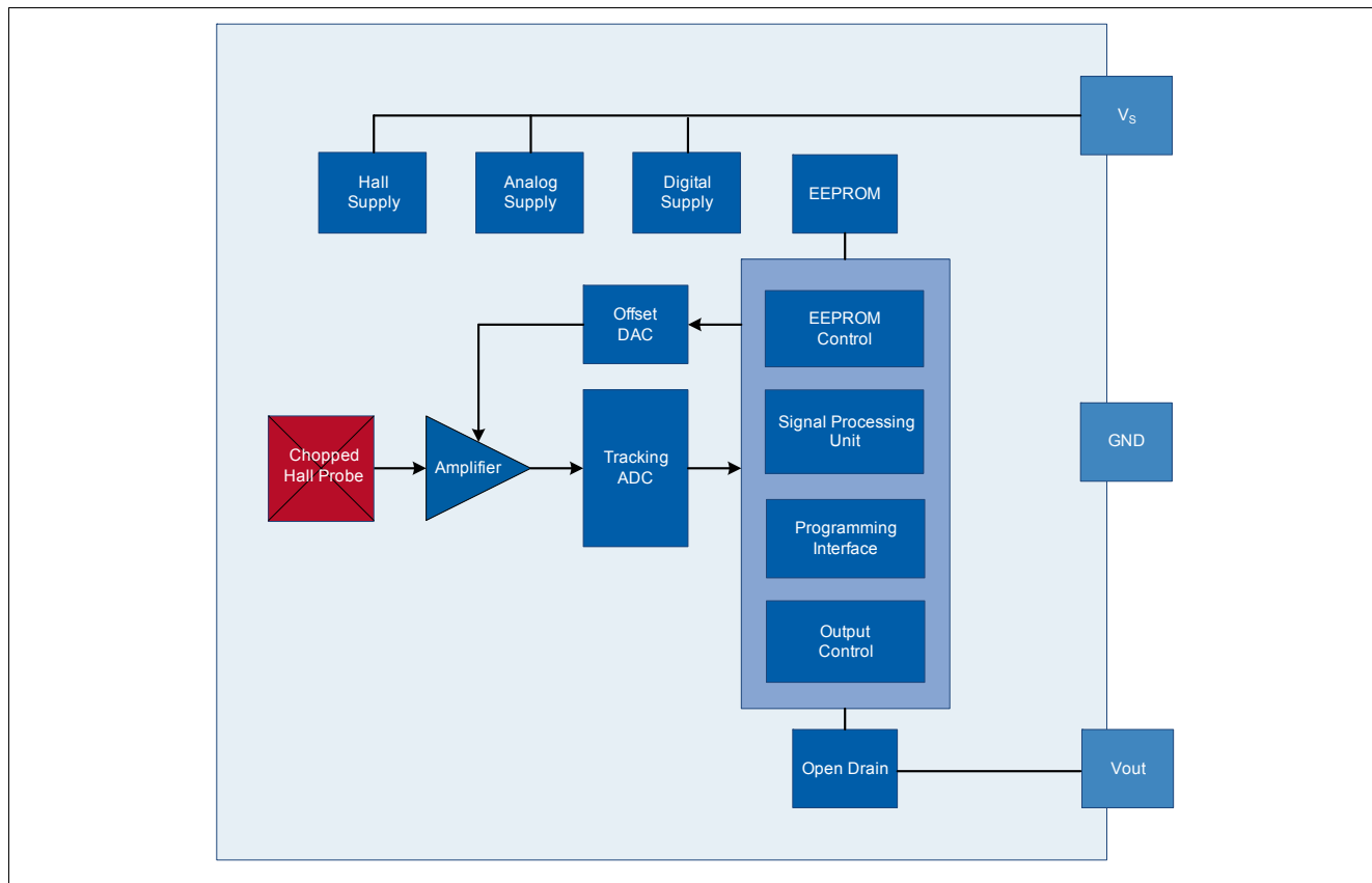
Figure 9 Block Diagram
