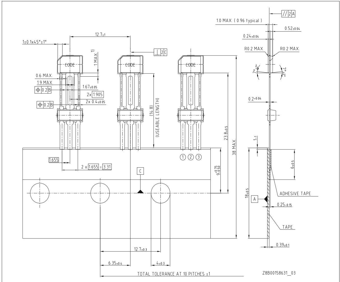
Figure 15 PG-SSO-3-52 Ammopack
