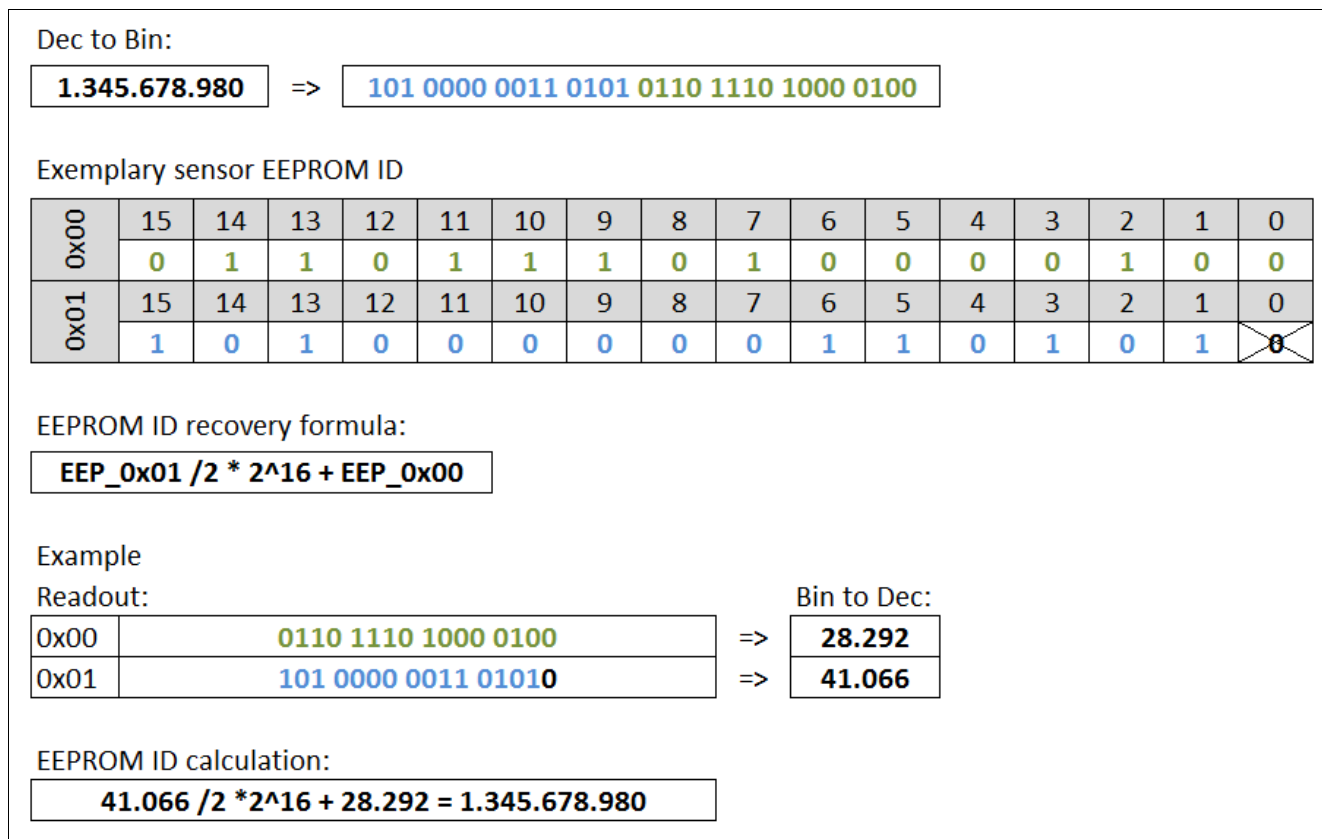
Figure 17 EEPROM ID programming example
