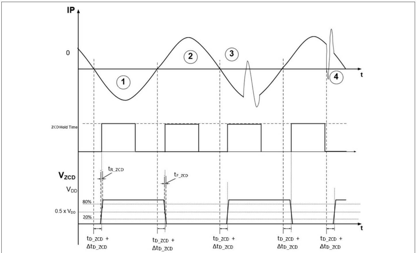
Figure 19 ZCD output timing diagram
