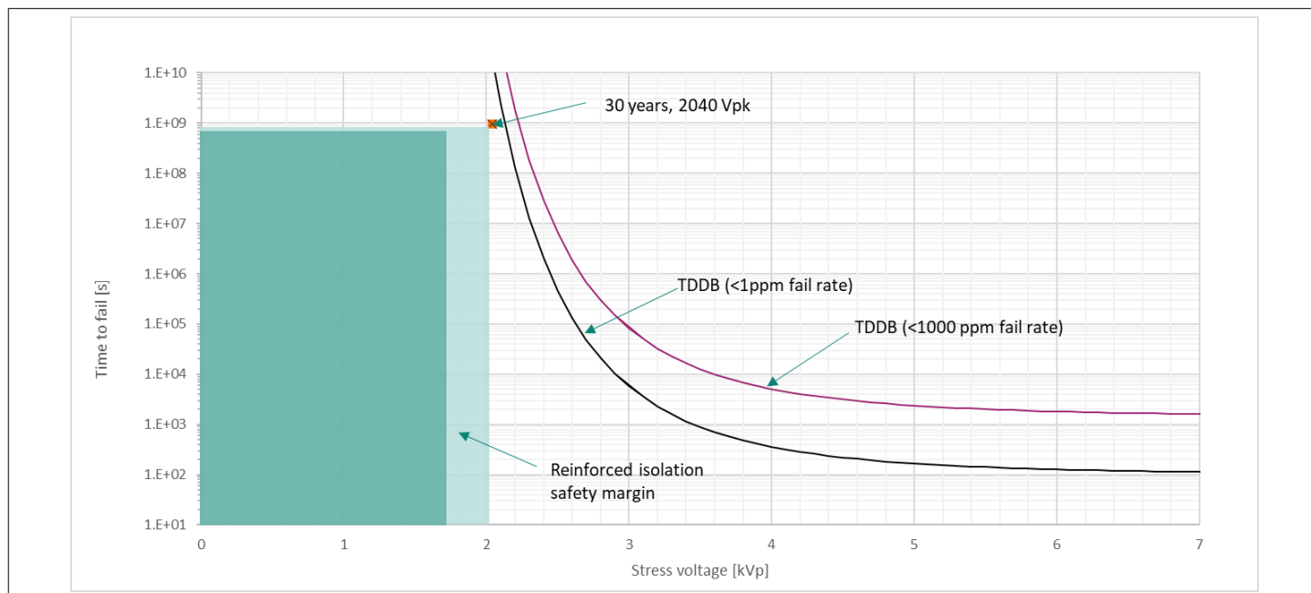
Figure 11 Insulation lifetime
