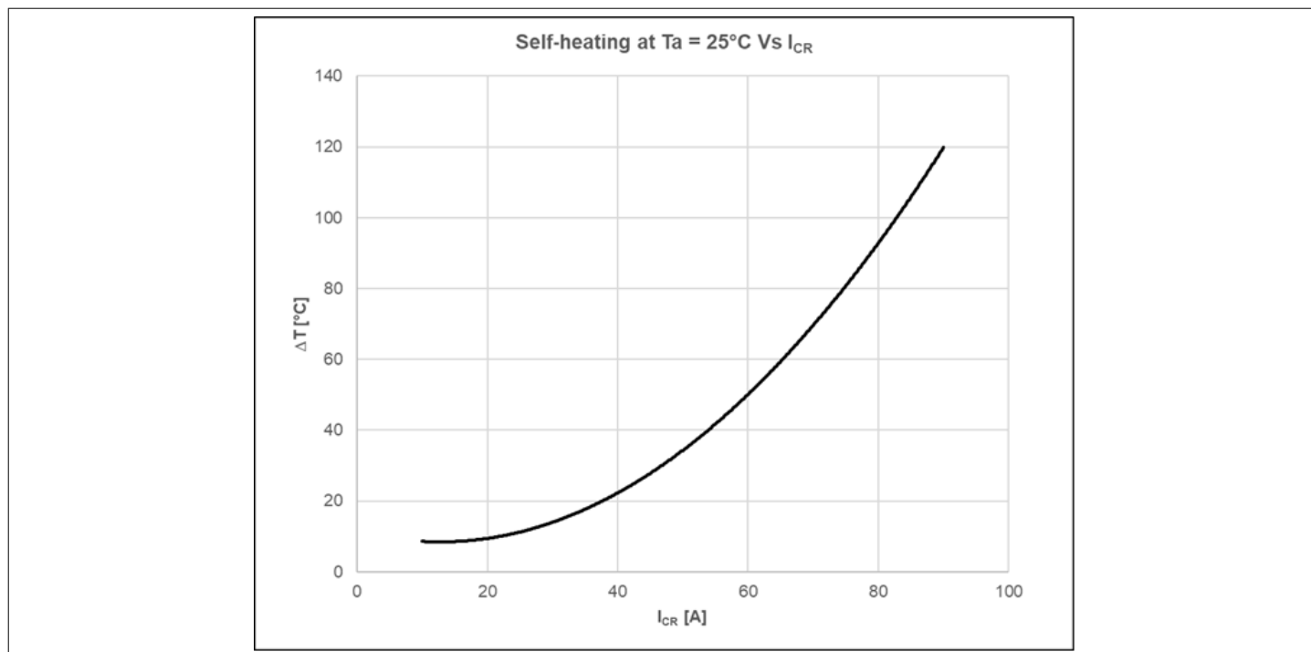
Figure 10 Self heating vs maximum continuous RMS current
