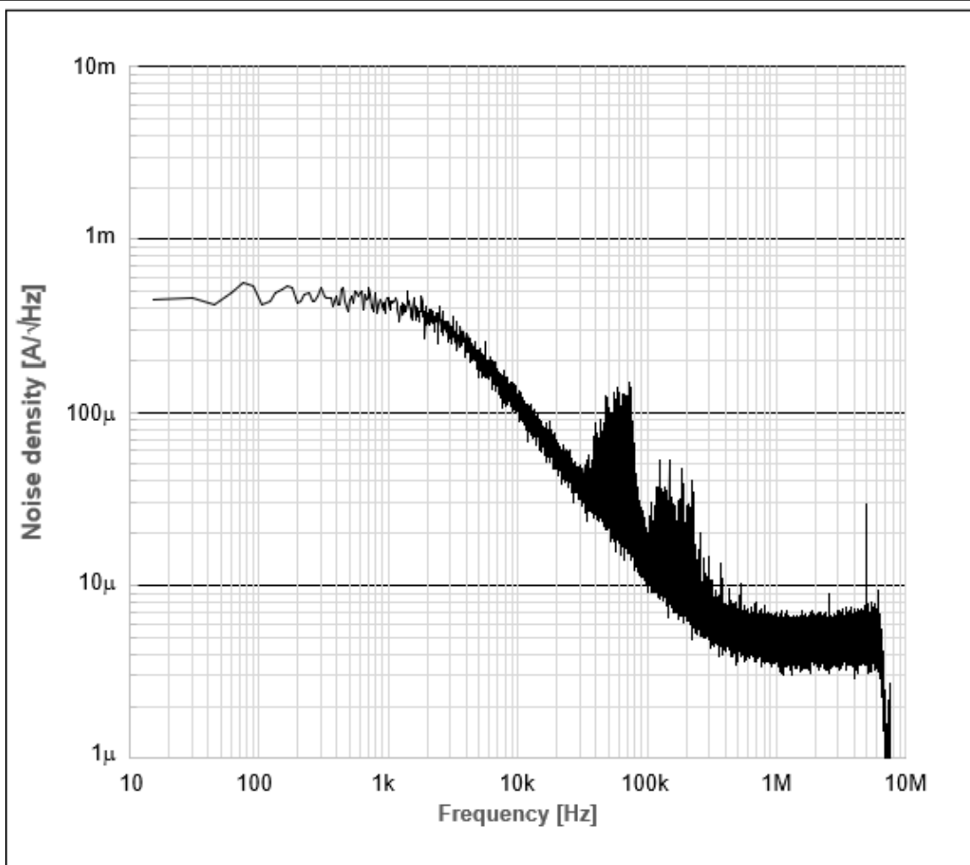
Figure 12 Noise density vs frequency
