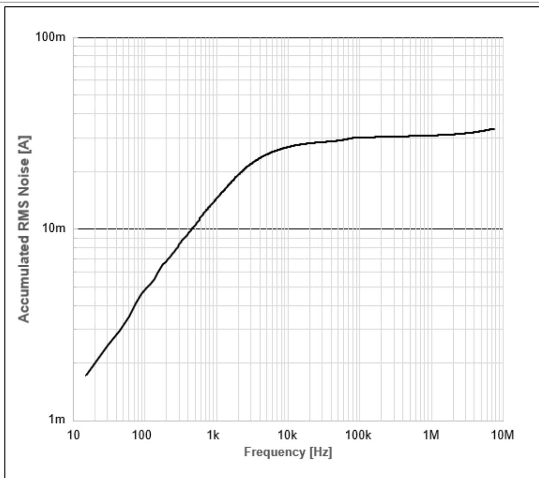
Figure 11 Input referred accumulated noise vs frequency
