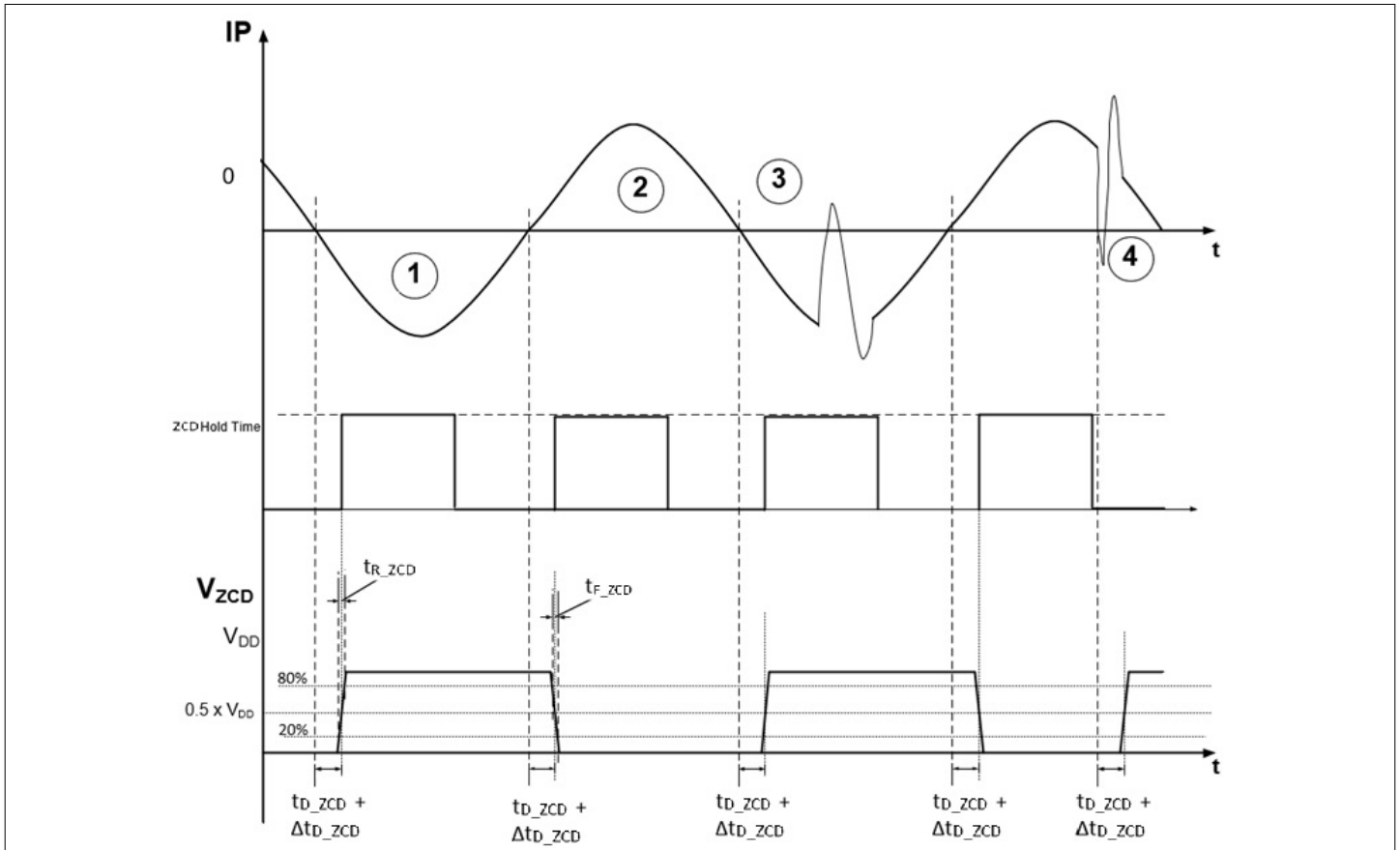
Figure 18 ZCD output timing diagram
