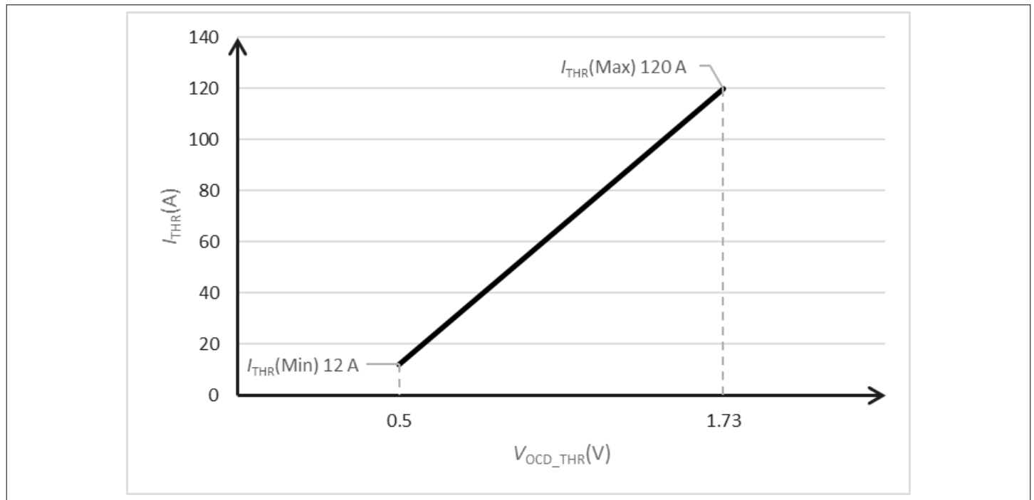
Figure 19 Threshold voltage ( V_{\text{OCD\_THR}} ) vs threshold current ( I_{\text{THR}} ) for the TLE4977-x080x product type
