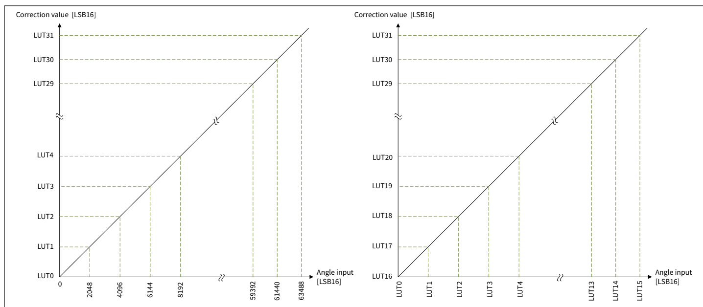
Figure 4 32 equidistant correction values (left) and 16 freely programmable correction values (right)
