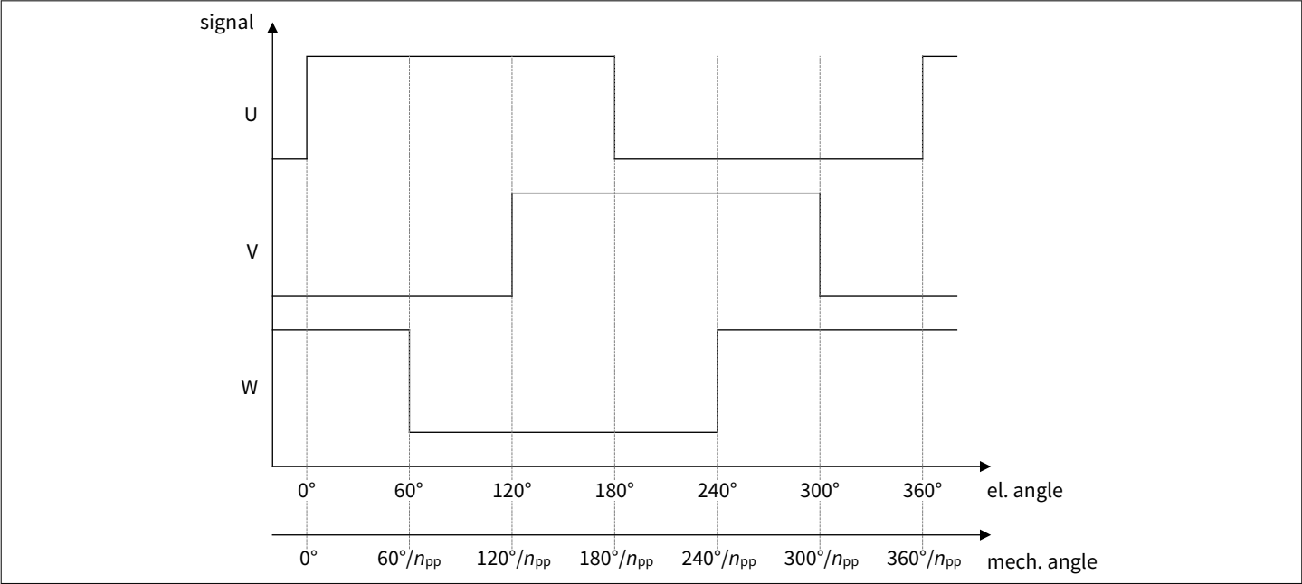
Figure 16 UVW interface switching pattern
