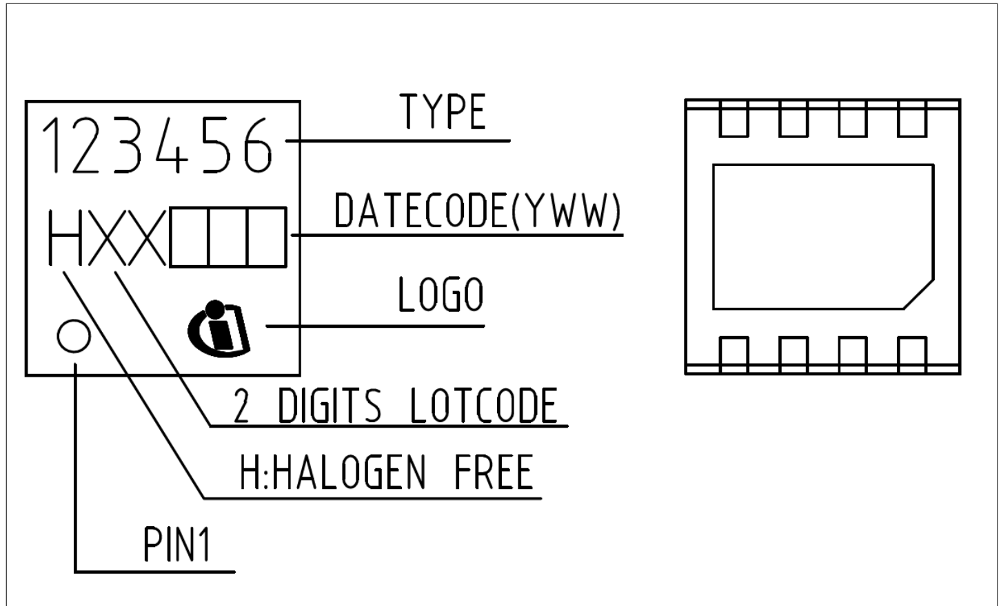
Figure 25 PG-VSON-8 package marking (left top side, right bottom side)
