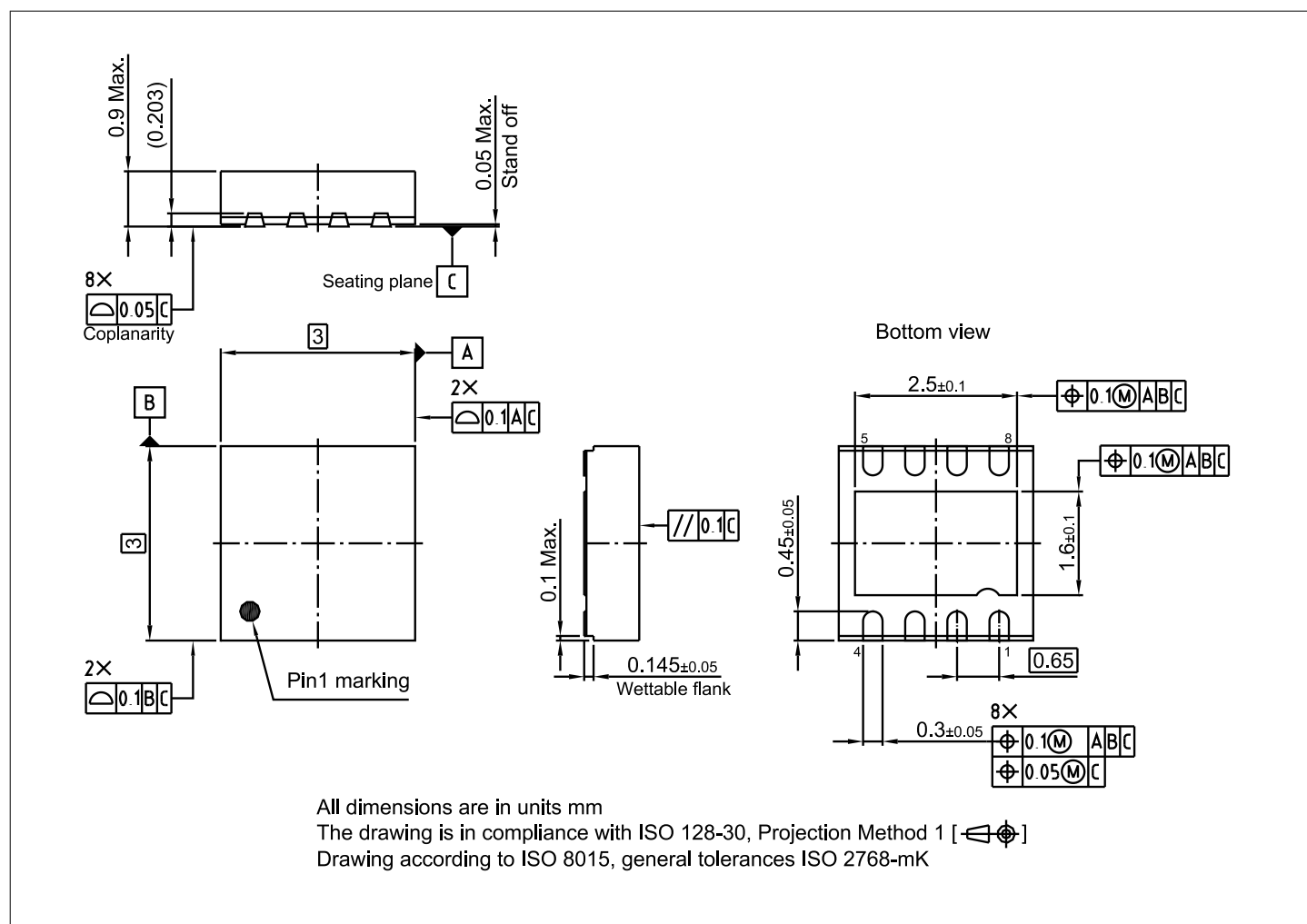
Figure 23 Package outline PG-VSON-8
