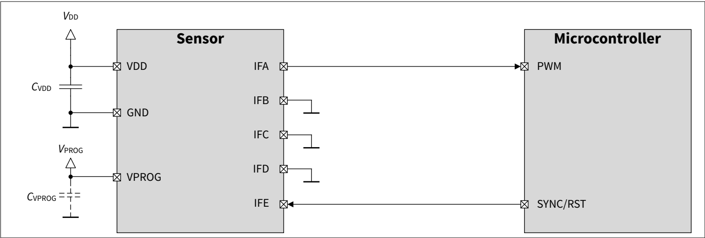
Figure 20 Application diagram - PWM
