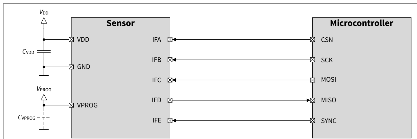
Figure 18 Application diagram - SPI
