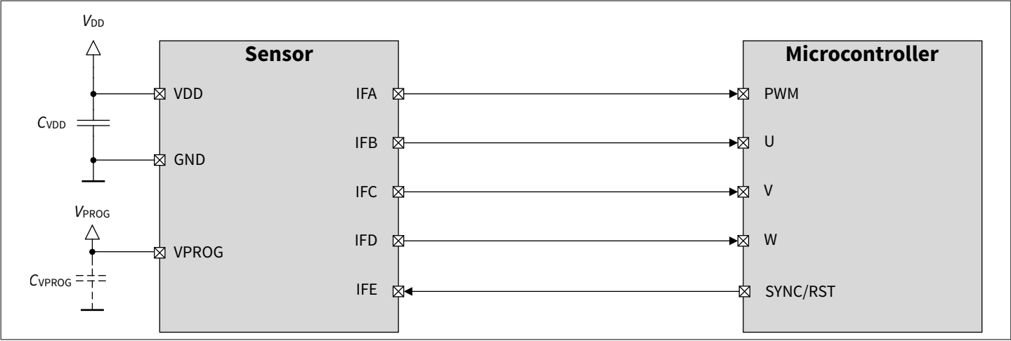
Figure 21 Application diagram - UVW in parallel with PWM
