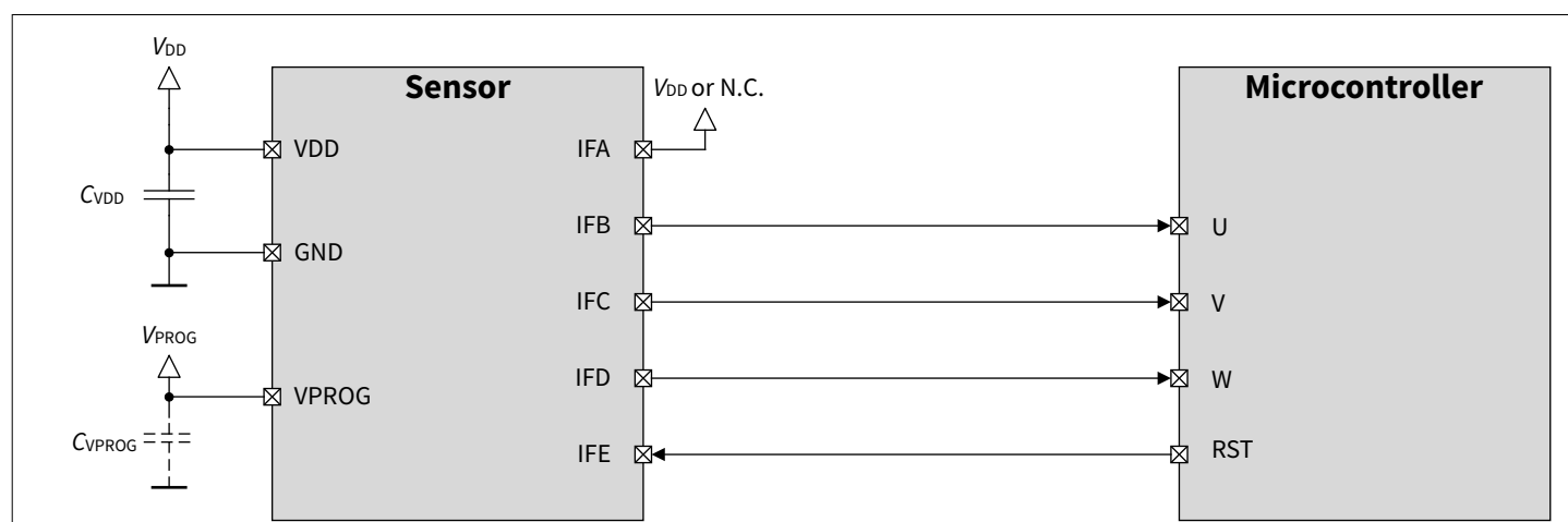
Figure 19 Application diagram - UVW (hall switch mode)
