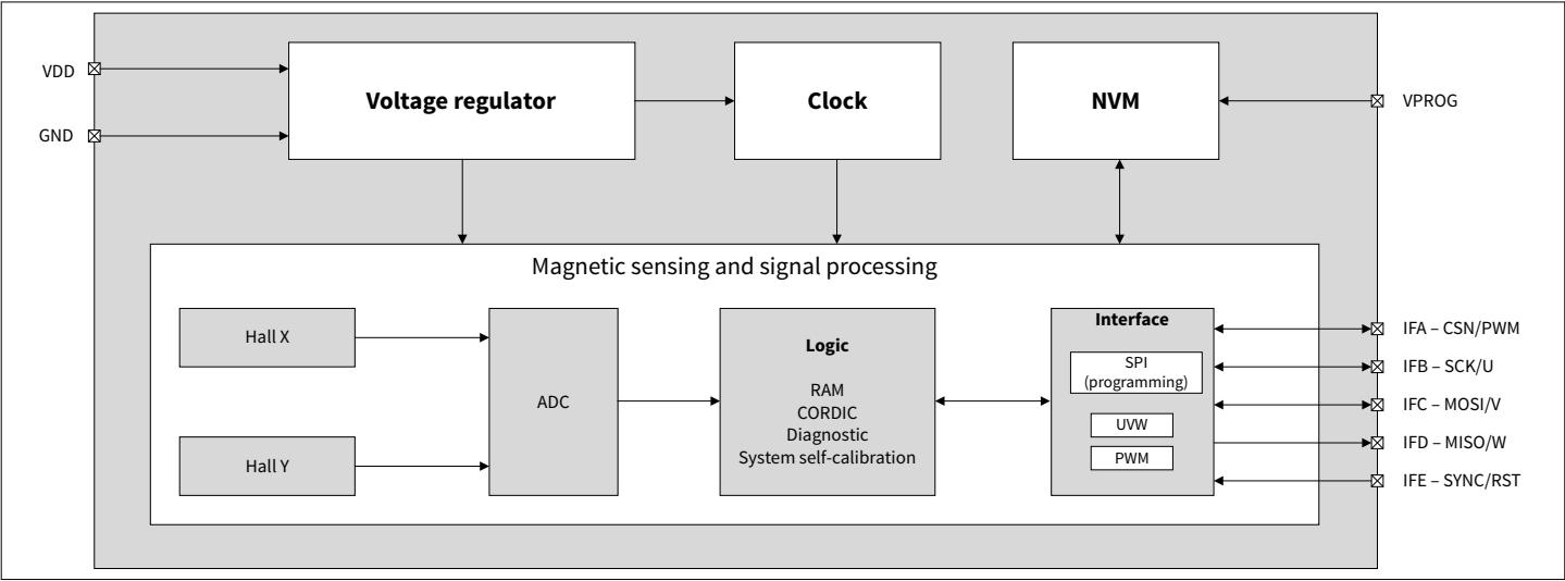
Figure 1 Block diagram
