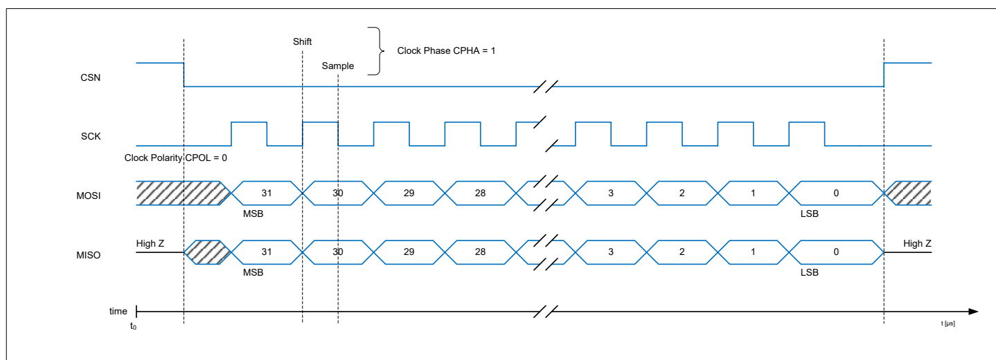
Figure 5 SPI mode 1
