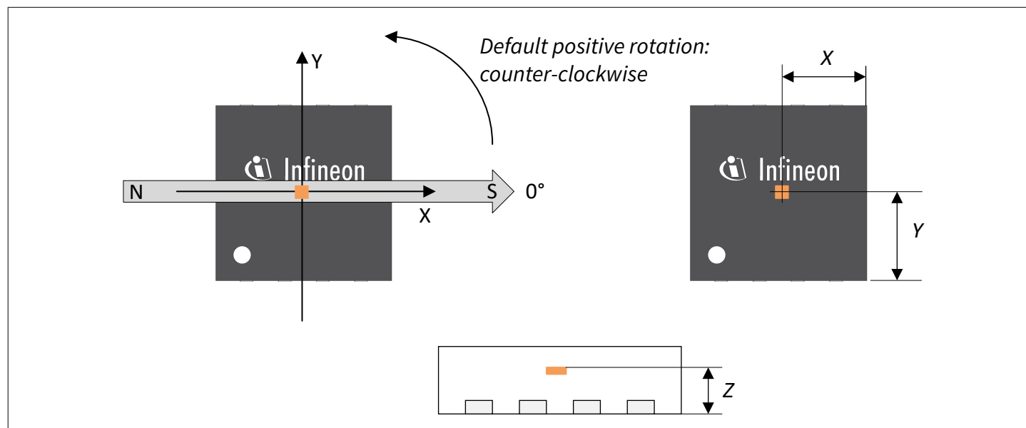
Figure 22 Sensitive area location (orange), Cartesian measurement reference system (black) and magnetic field vector indicating the 0° angle (grey)
