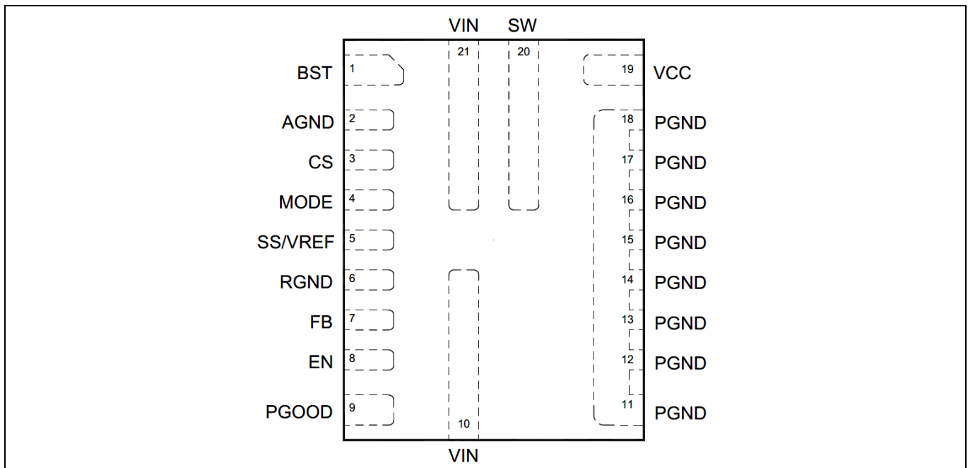
Figure 1 Package Top View – TDA48415
