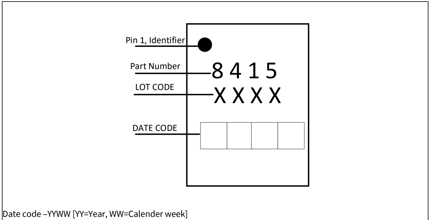
Figure 11 Package Marking
