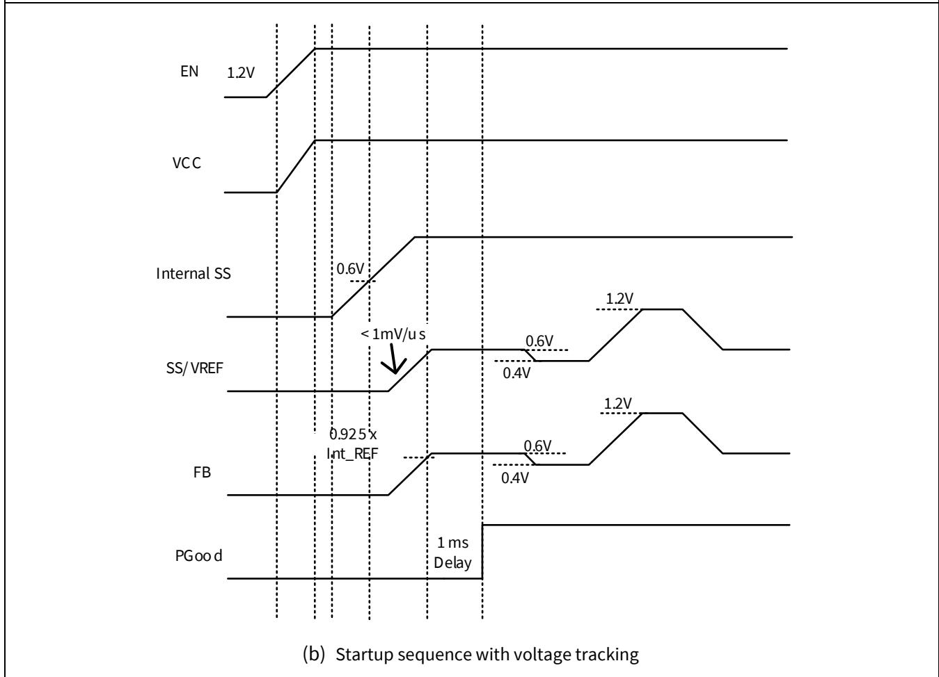
Figure 5 Startup sequence with external reference and voltage tracking
