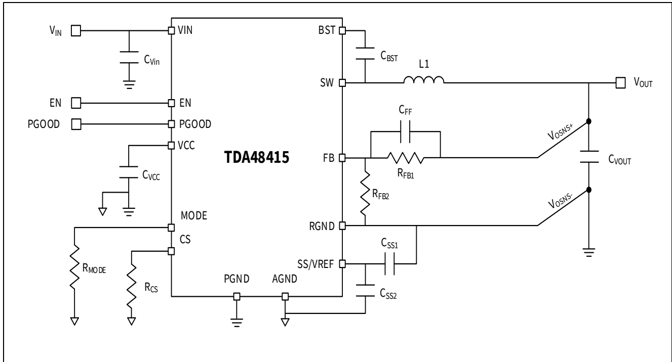
Figure 3 TDA48415 Typical application circuit
