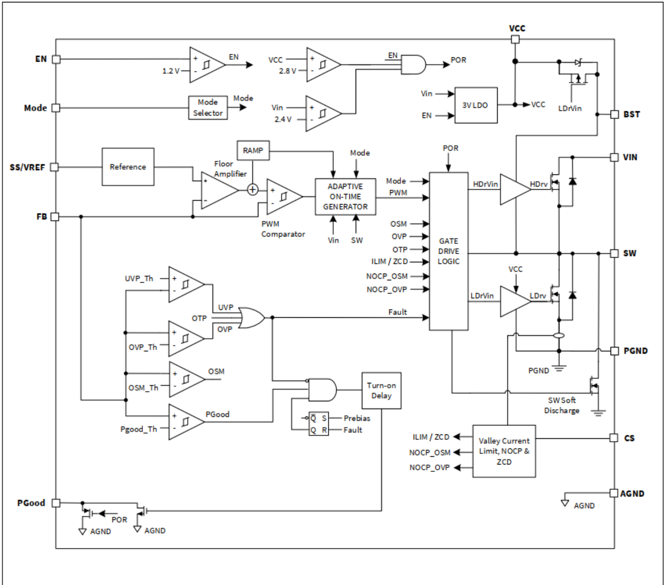
Figure 2 框图
