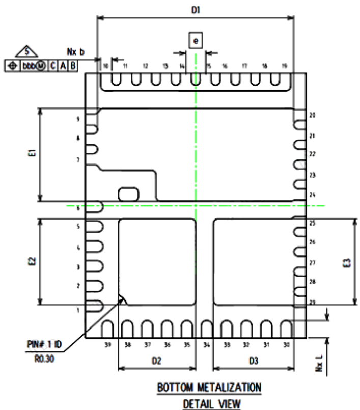
Figure 14 Mechanical Dimensions of Package (Bottom View) in mm
