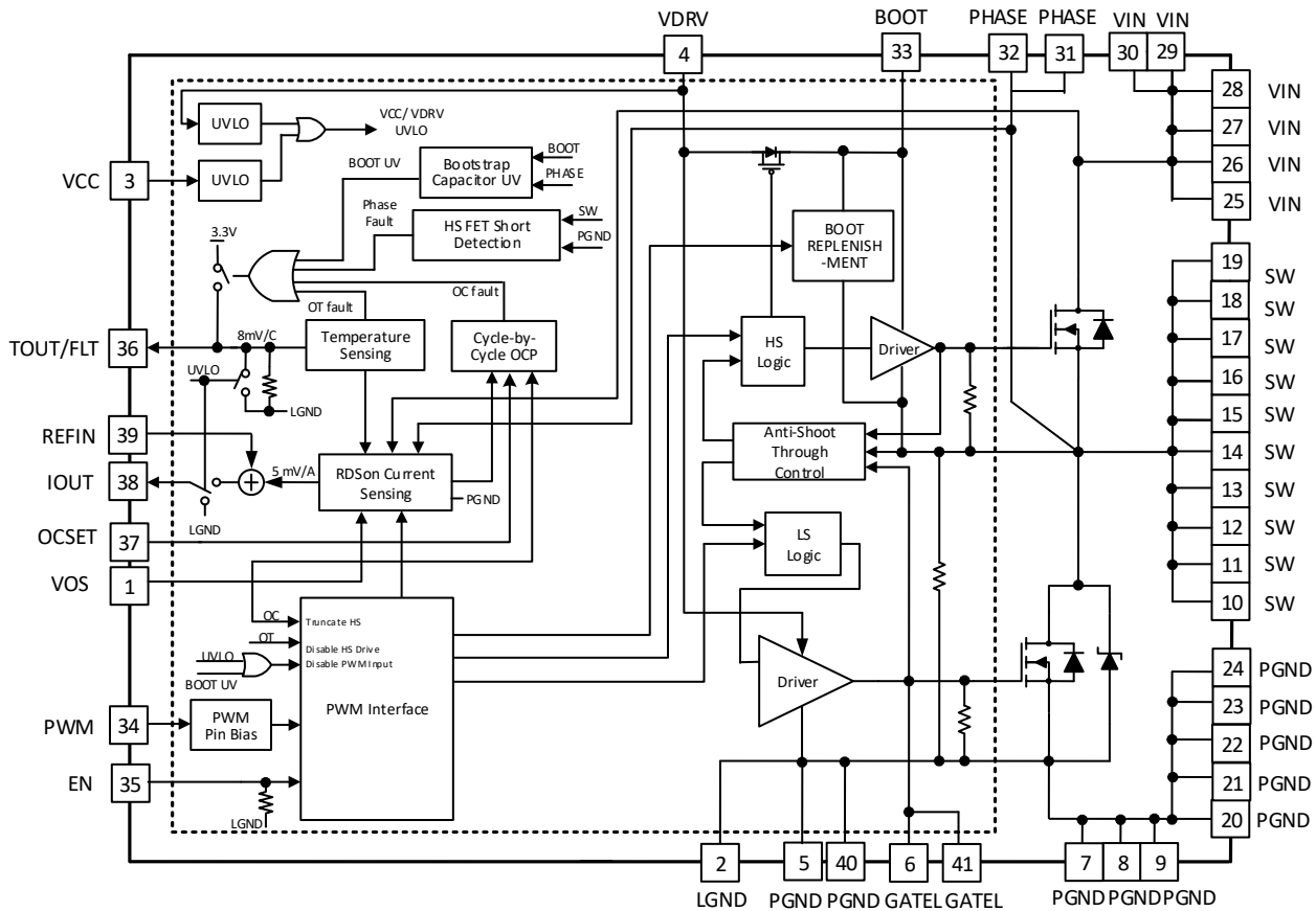
Figure 3 Block Diagram
