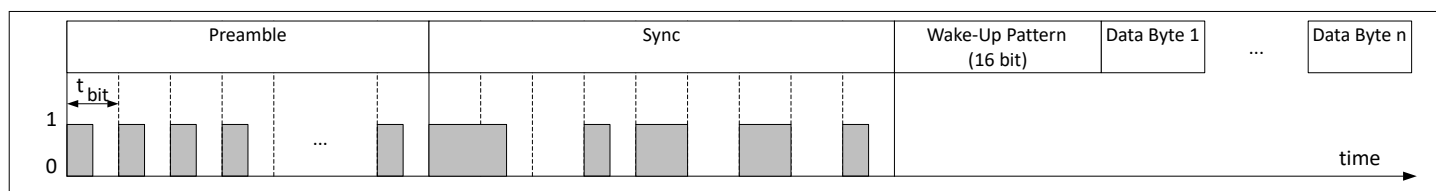
Figure 9 LF telegram
