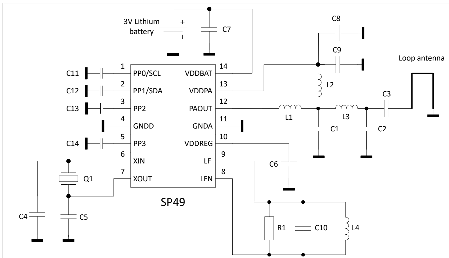
Figure 12 Application circuit
