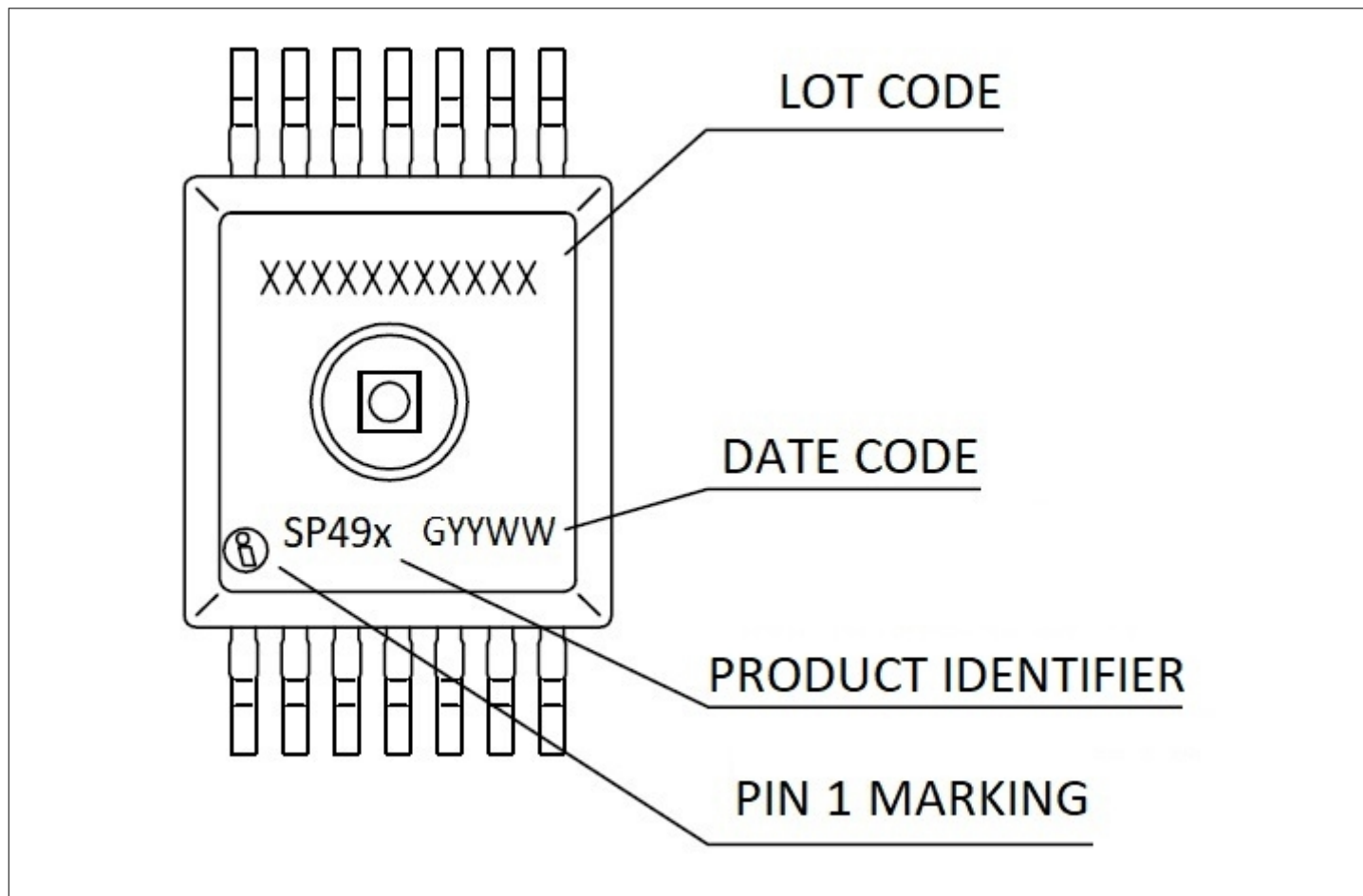
Figure 14 Package Marking
