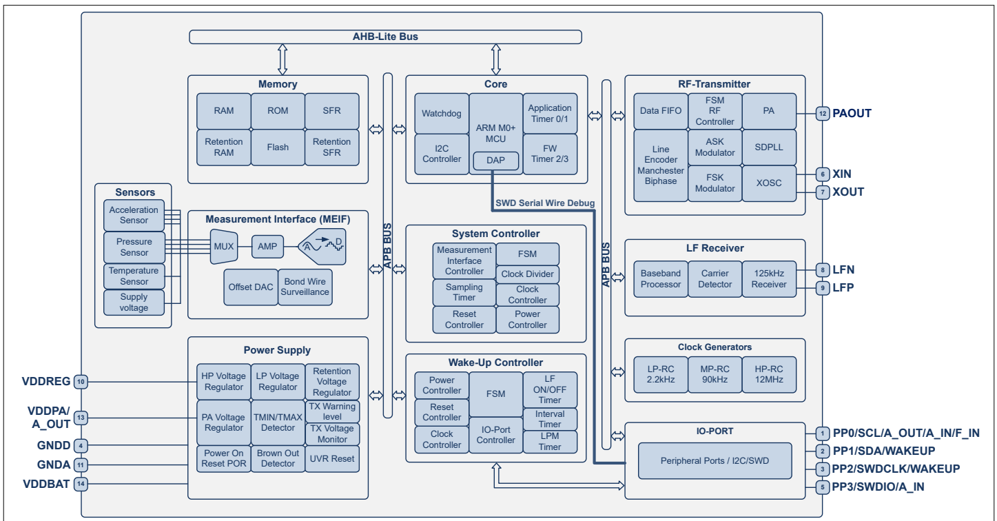
Figure 4 Block diagram
