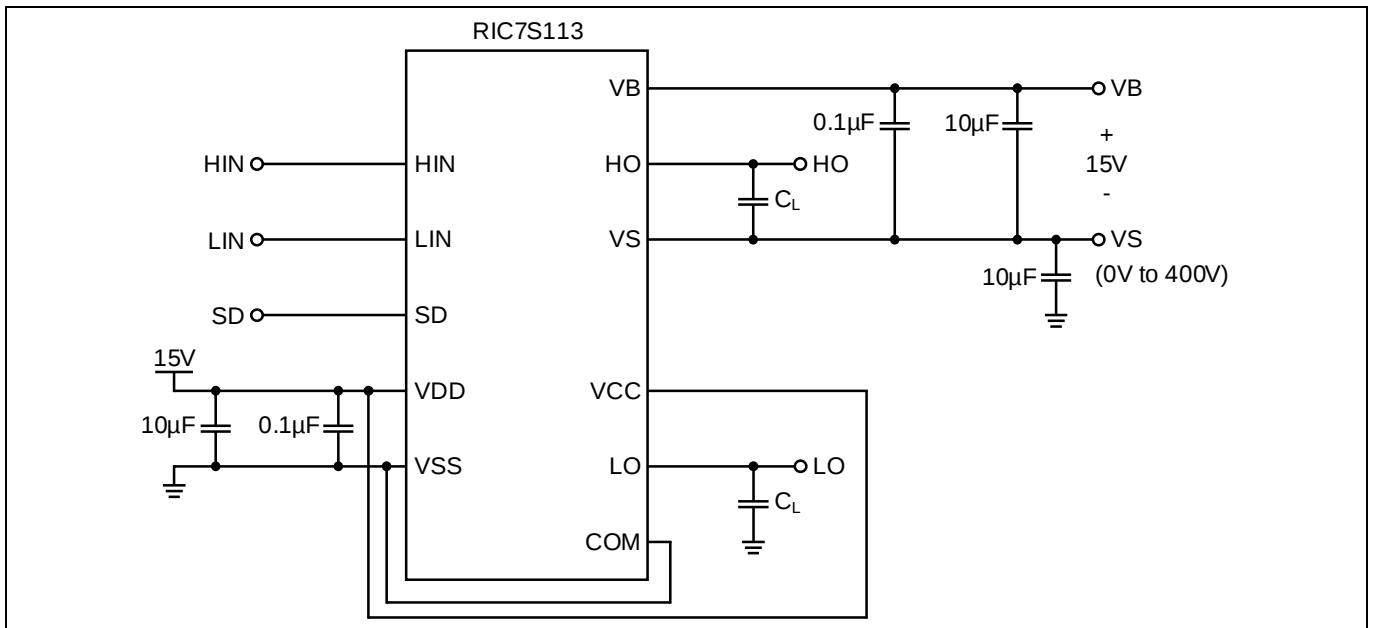
Figure 7 Switching time test circuit
