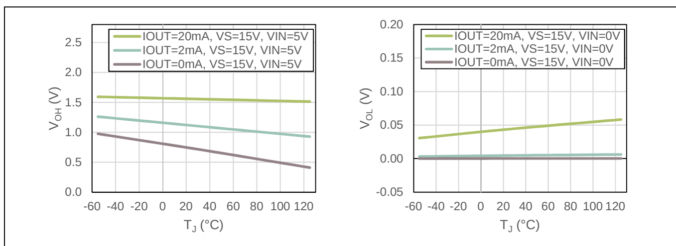
Figure 10 V_{OH} and V_{OL} over temperature
