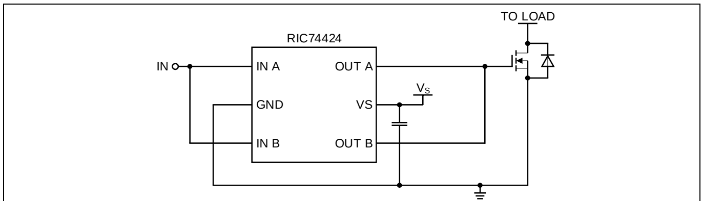
Figure 14 Parallel output
