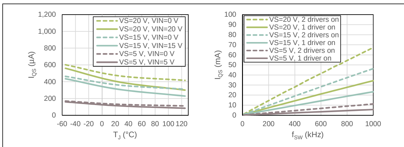
Figure 7 I_{QS} over temperature and frequency
