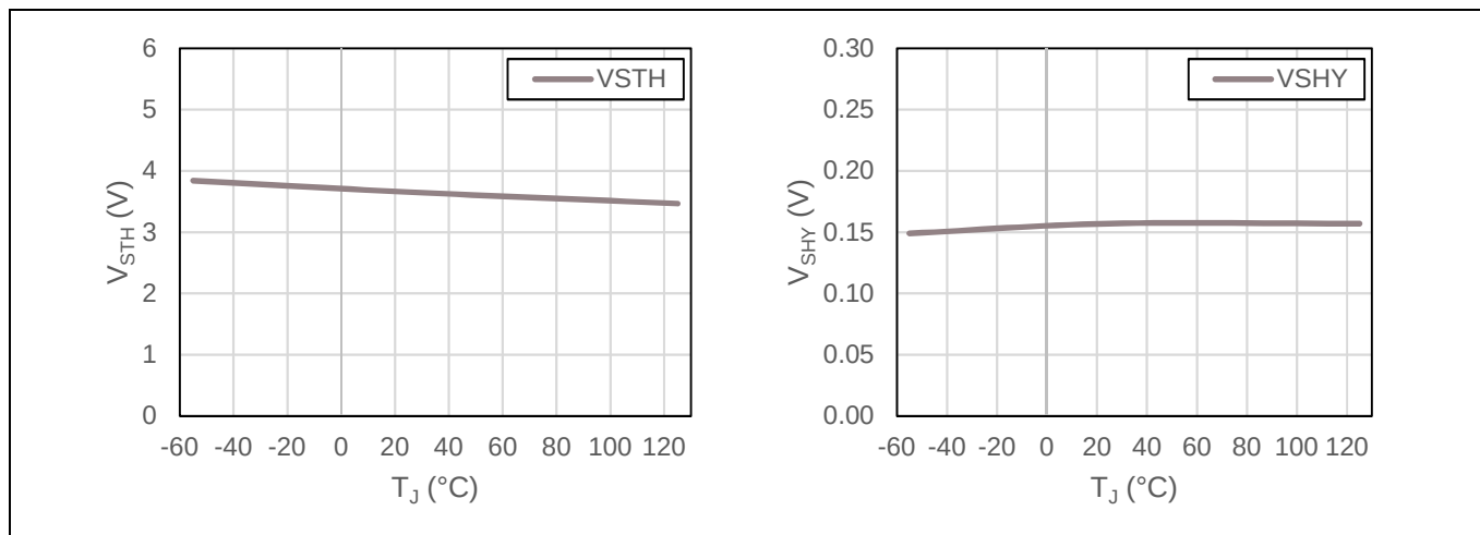
Figure 6 V_{STH} and V_{SHY} over temperature
