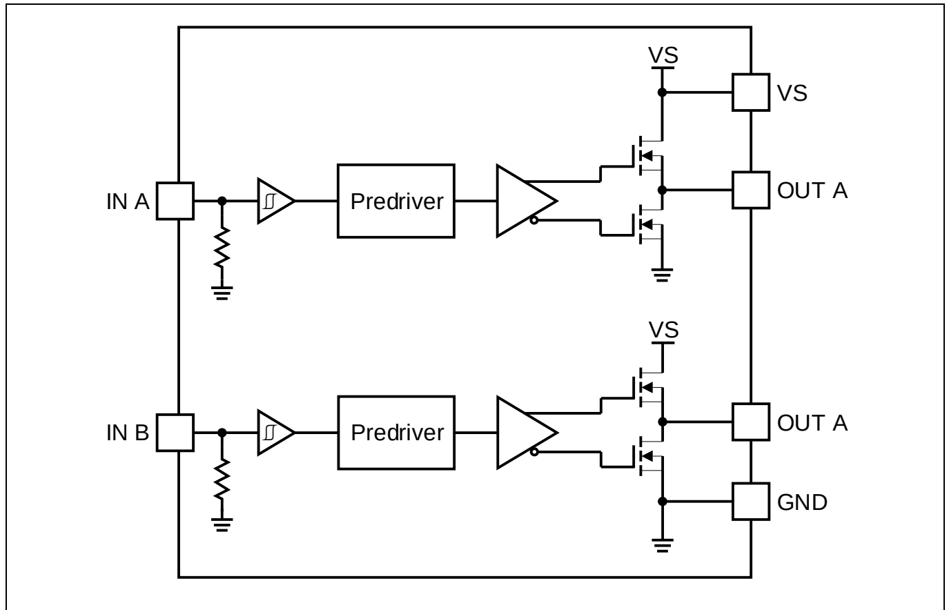
Figure 2 Block diagram
