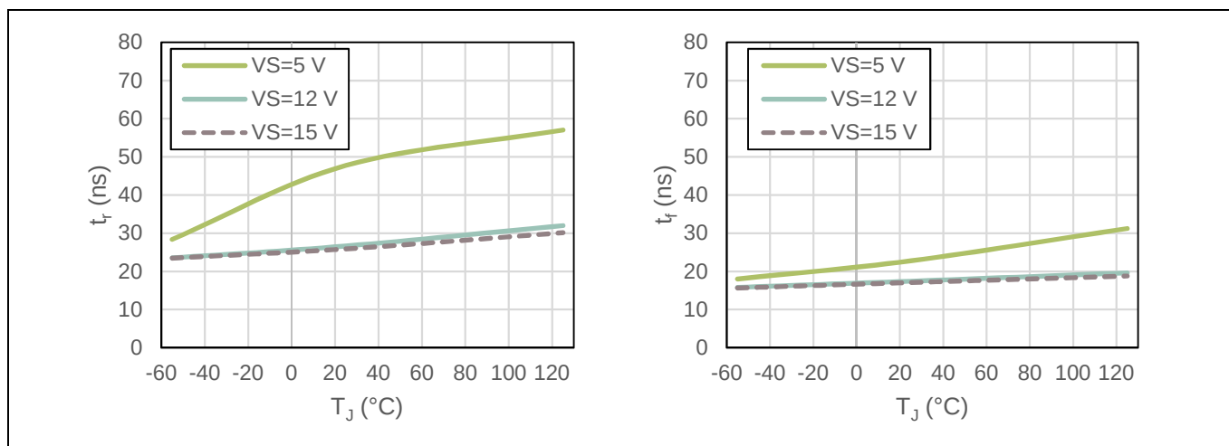
Figure 11 t_r and t_f over temperature
