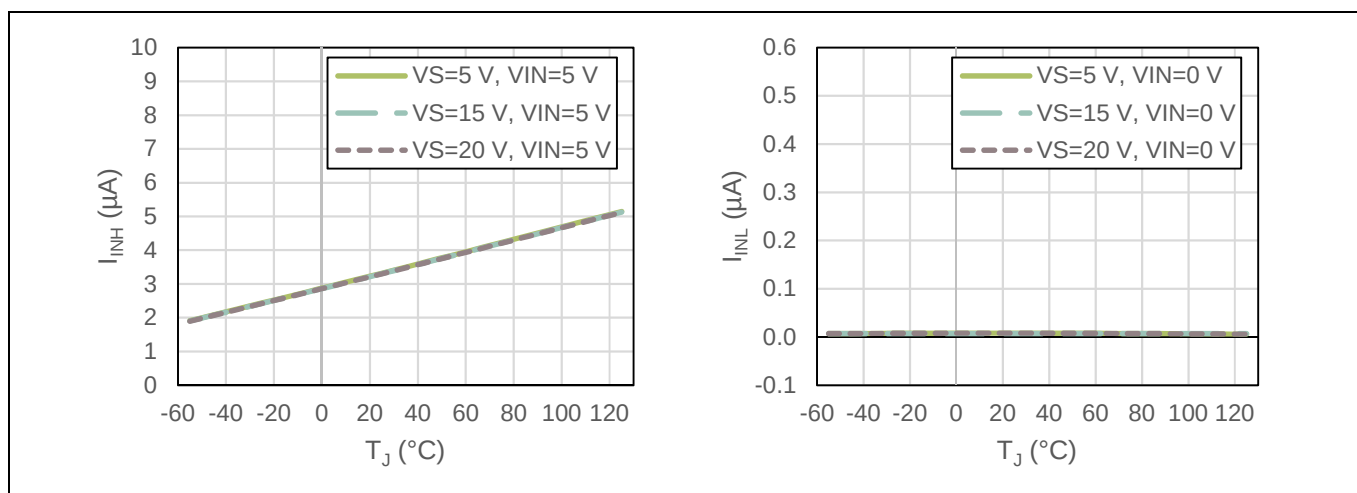
Figure 9 I_{INH} and I_{INL} over temperature
