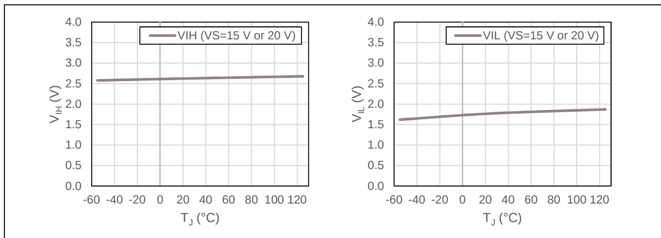
Figure 8 V_{IH} and V_{IL} over temperature
