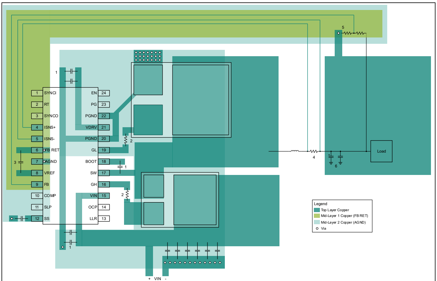
Figure 36 Recommended PCB layout for RIC70847
