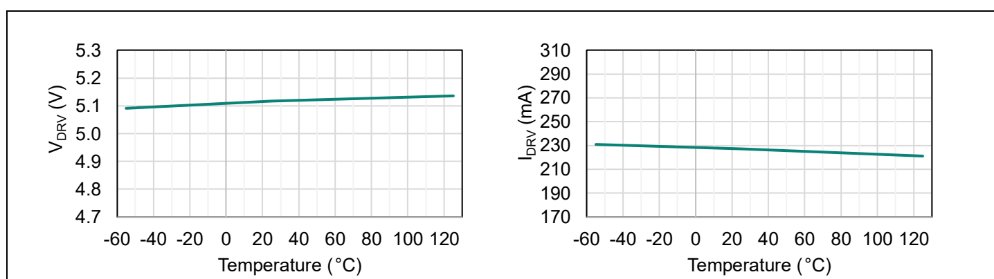
Figure 12 VDRV voltage ( V_{DRV} ) and VDRV current limit at V_{IN}=13.2 V ( I_{DRV} ) over temperature
