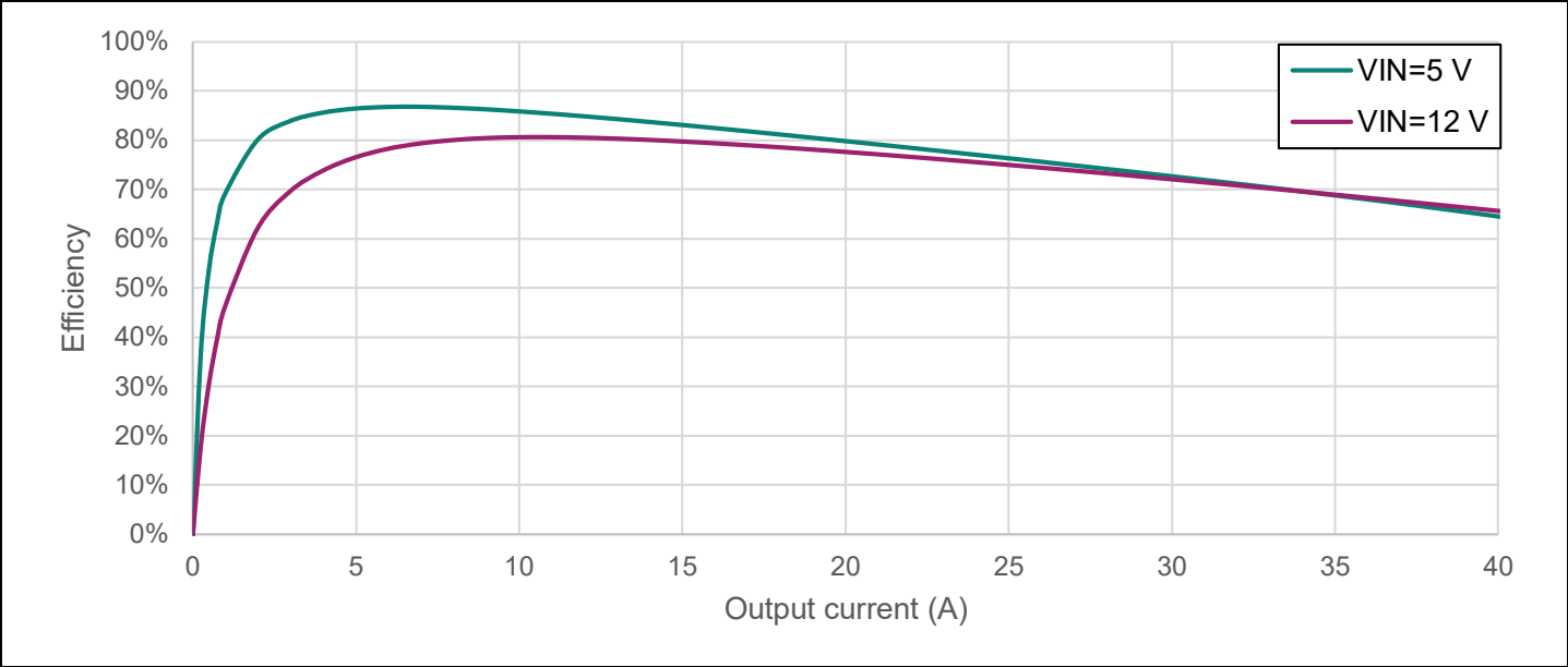
Figure 4 Efficiency over load at 500 kHz and V_{OUT}=1 V at V_{IN}=5 V and V_{IN}=12 V, L=270 nH, C_{OUT}=5.6 mF
