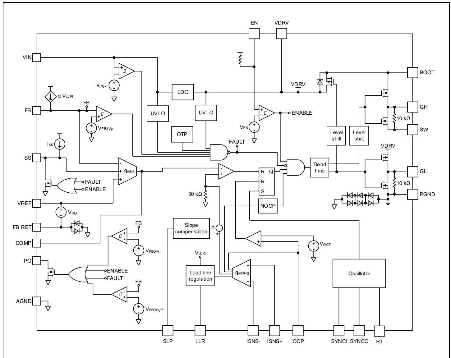
Figure 2 RIC70847 block diagram
