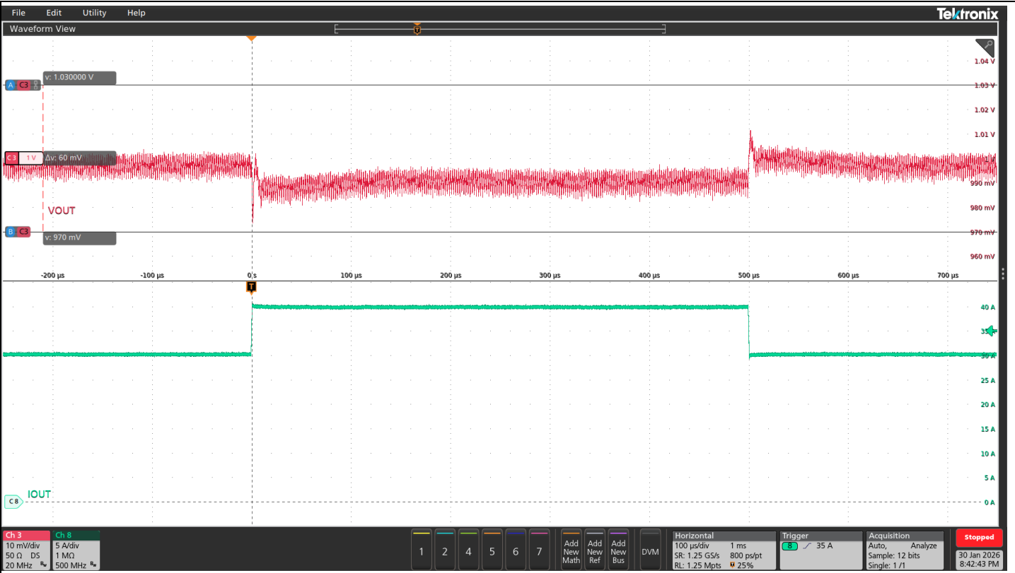
Figure 7 Transient load step and release with LLR enabled at maximum load (30 A to 40 A at 10 A/μs)
