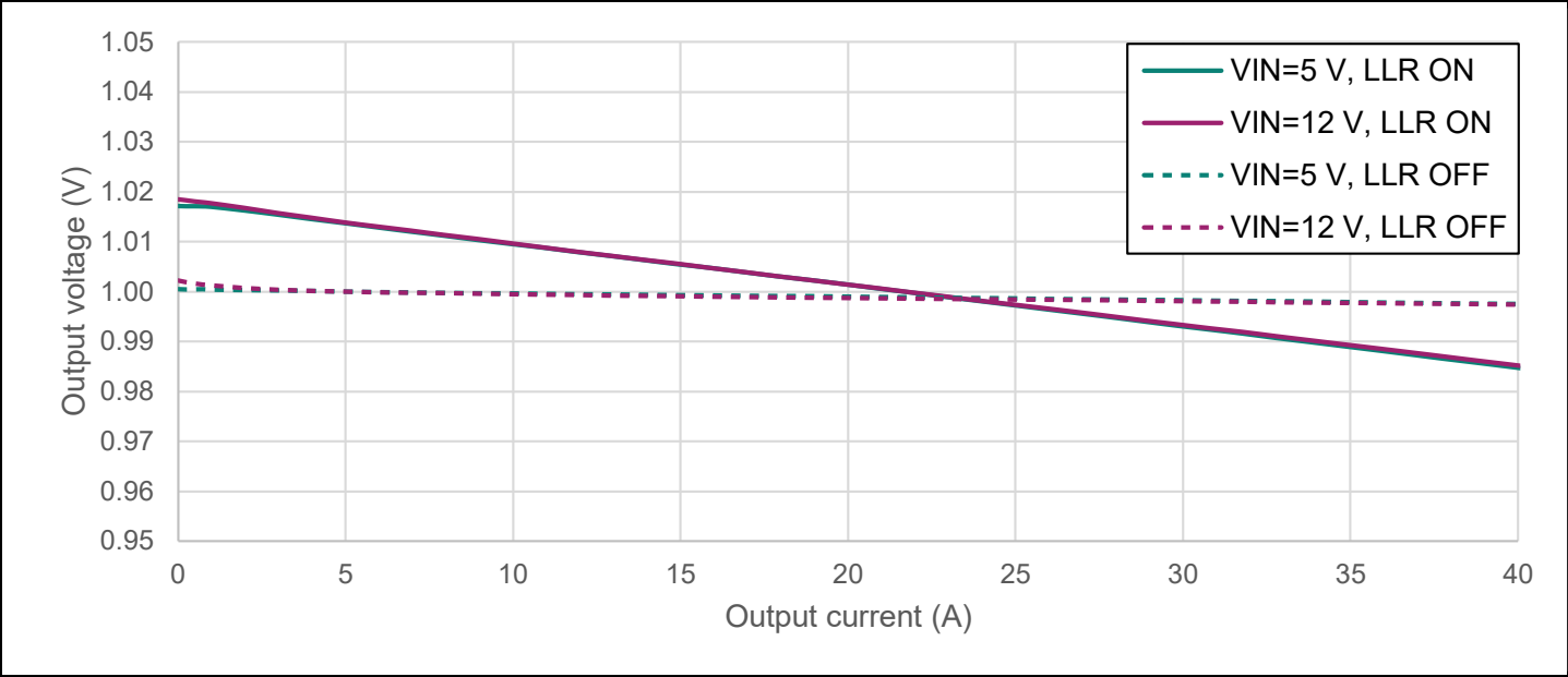
Figure 5 Output voltage regulation accuracy with and without LLR over load at 500 kHz and V_{OUT}=1.0 V at V_{IN}=5 V and V_{IN}=12 V, L=270 nH, C_{OUT}=5.6 mF
