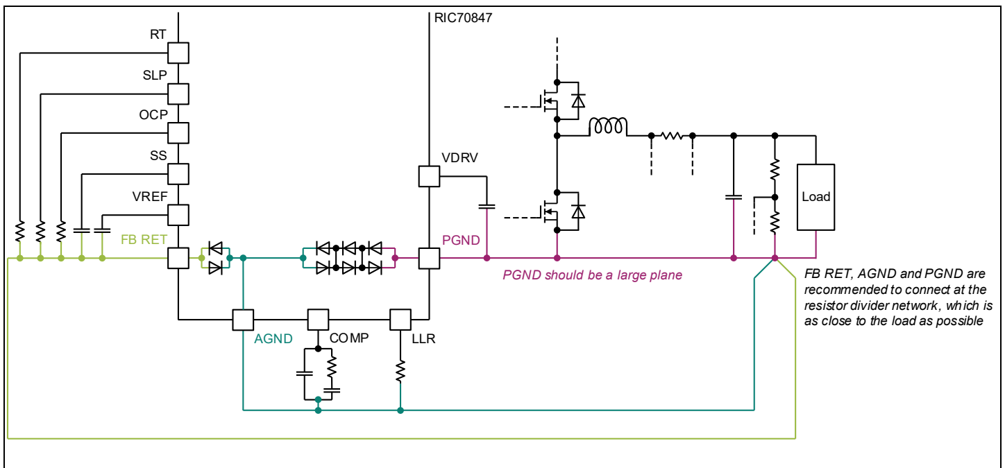
Figure 24 Example external connections for return pins PGND, AGND and FB RET
