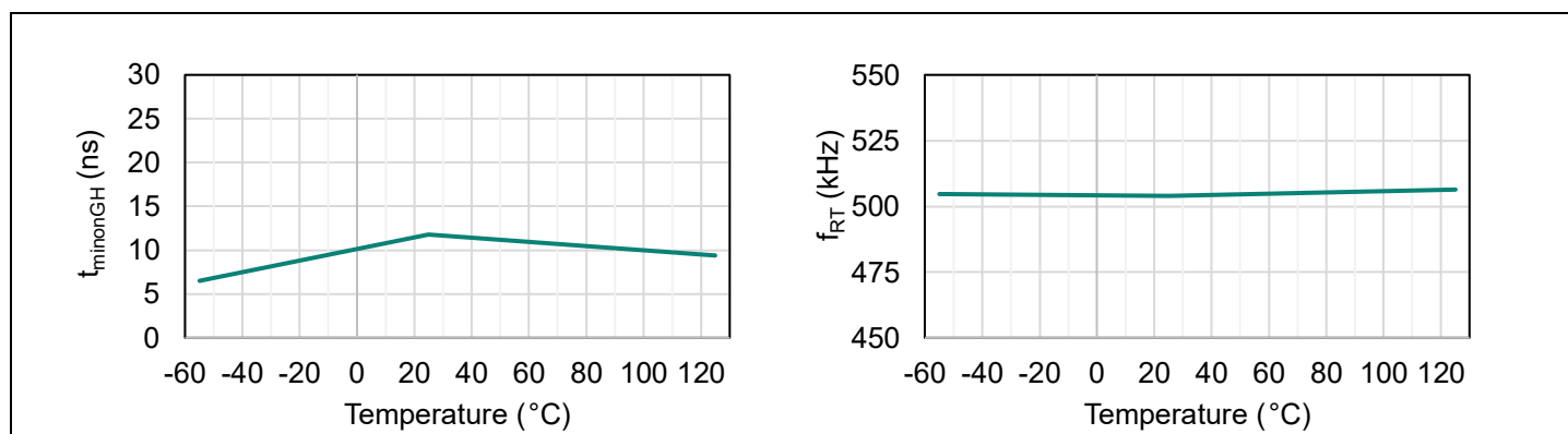
Figure 13 Minimum on time for GH ( t_{minonGH} ) and internal oscillator frequency with R_T=28.6 k \Omega ( f_{RT} ) over temperature
