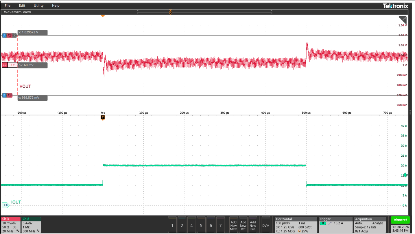
Figure 6 Transient load step and release with LLR enabled at minimum load (10 A to 20 A at 10 A/μs)
