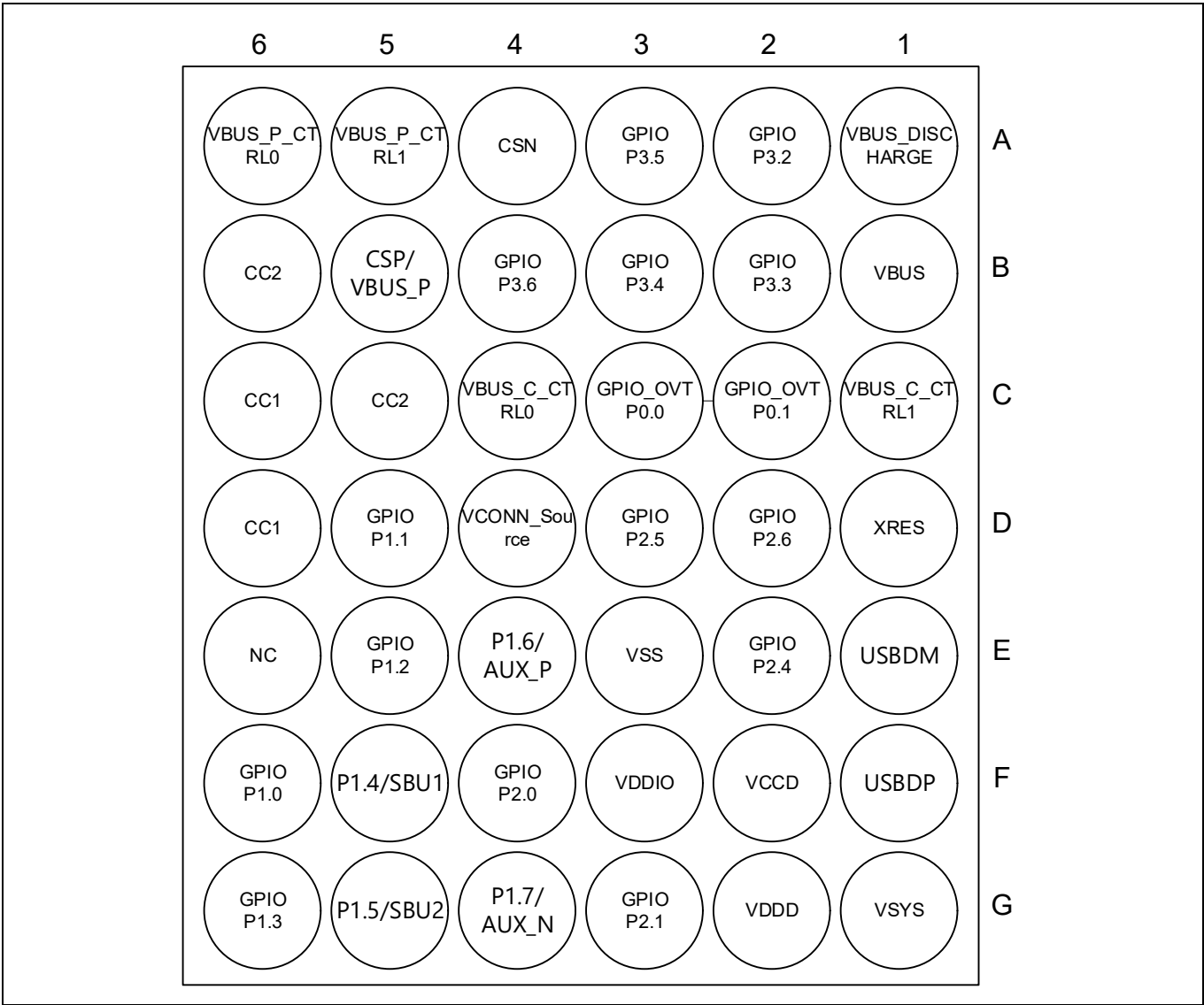
Figure 5 Pinout of 42-WLCSP bottom (balls up) view
