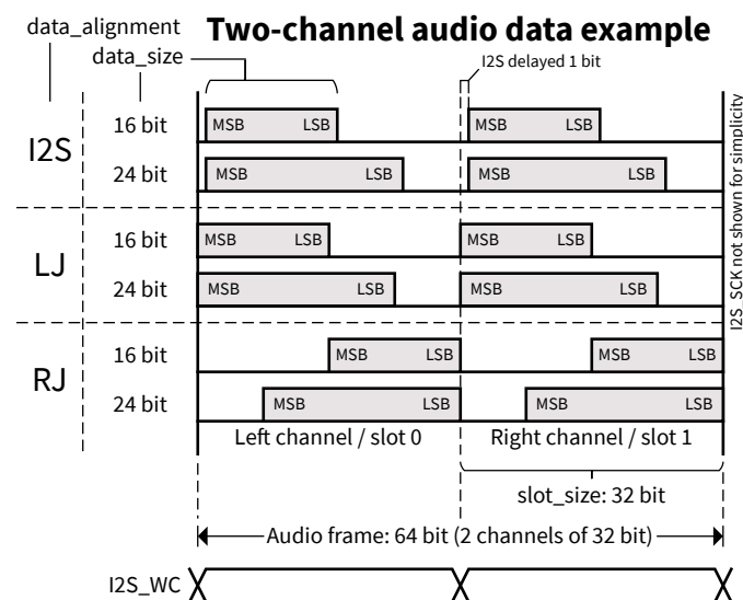
Figure 11.15: Audio data configuration/timing for two channels
