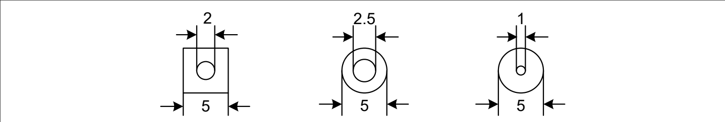
Figure 22 Examples of nozzle shapes for sealing on the lid
