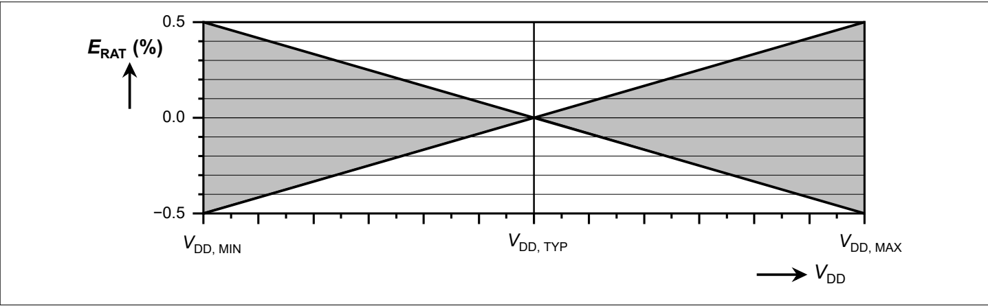
Figure 4 Ratiometric error
