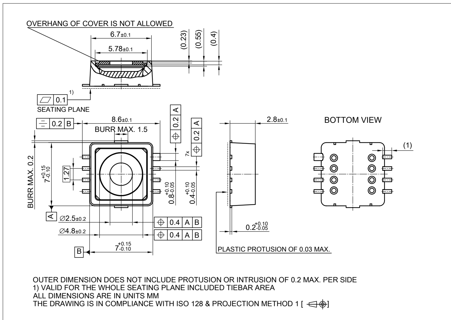
Figure 11 Package outline
