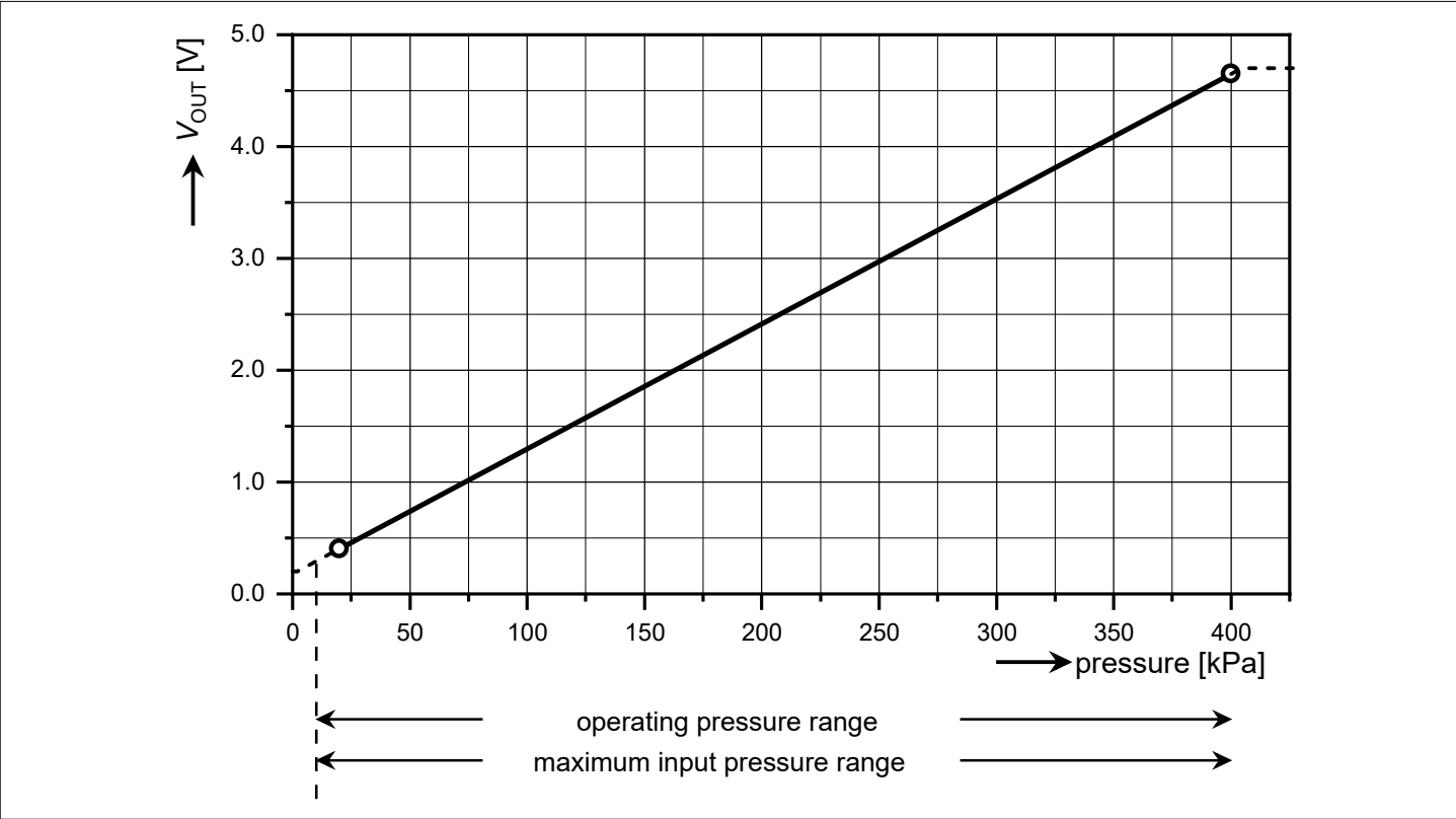
Figure 3 Transfer function
