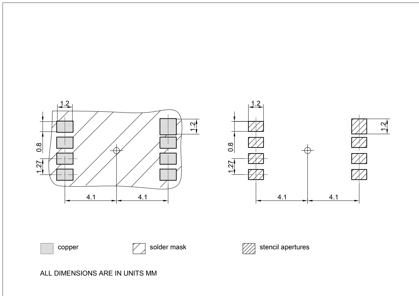
Figure 12 Footprint drawing
