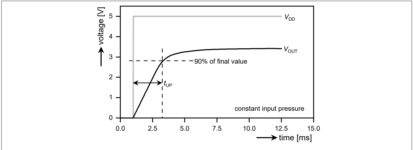
Figure 8 Power-up time
