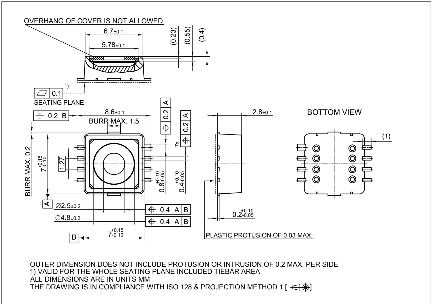
Figure 11 Package outline
