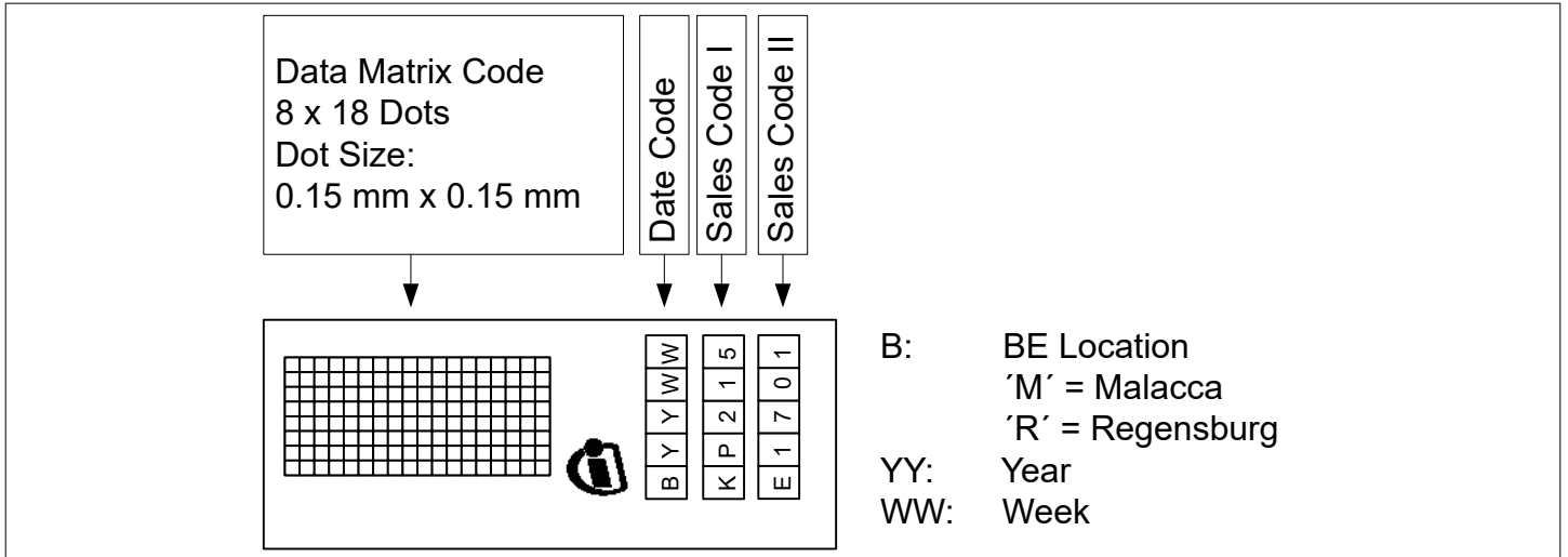
Figure 13 Identification code
