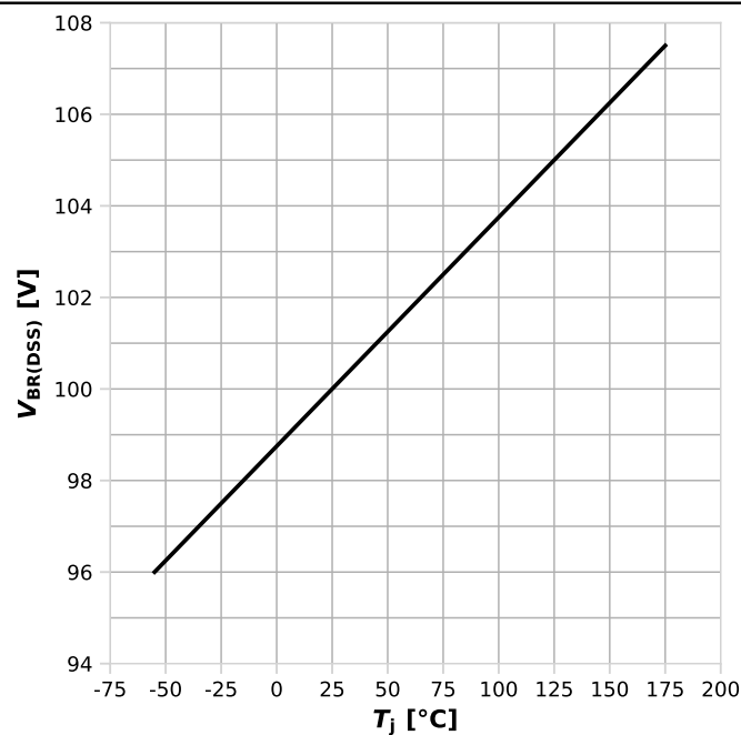
Diagram 16: Drain-source breakdown voltage
