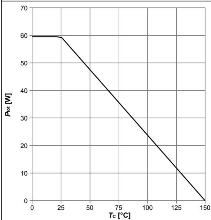
Diagram 1: Power dissipation
