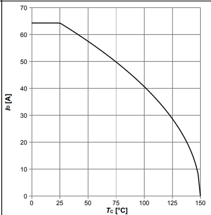
Diagram 2: Drain current
