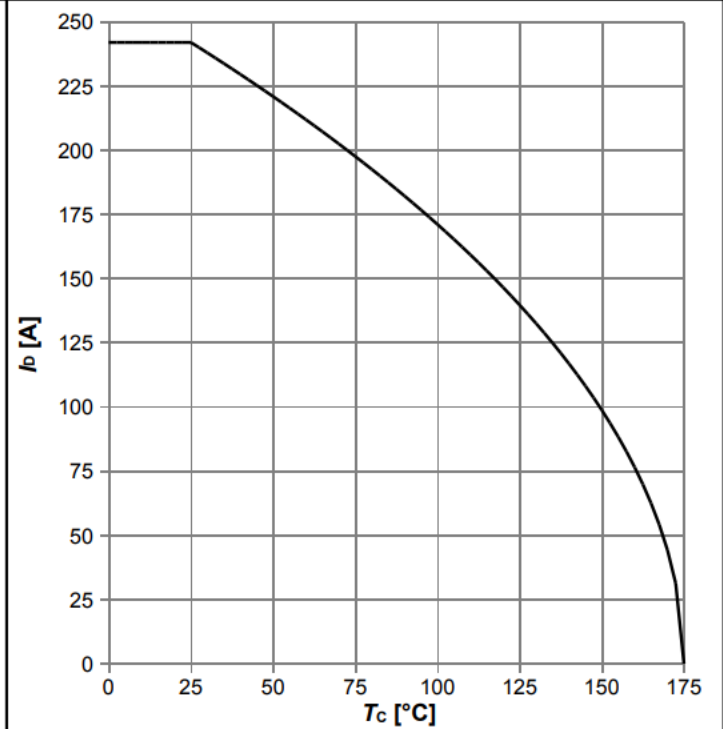
Diagram 2: Drain current
