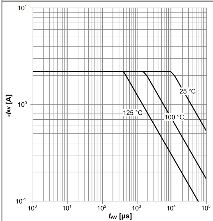
Diagram 13: Avalanche characteristics
