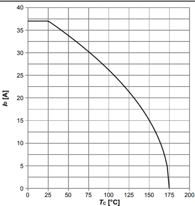
Diagram 2: Drain current
